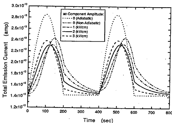
FIG. 4. Total nonadiabatic photoemission current I_e[\mathcal{E}_b(t), \Phi_{op}(t)] - \Delta I_e(t) as a function of time for different ac-component amplitudes \mathcal{E}_m=0, 1, 2, and 3 kV/cm. For convenience, the adiabatic photoemission current I_e[\mathcal{E}_0, \Phi_{op}(t)] with \mathcal{E}_m=0 (dotted curve) is also included in the figure.
