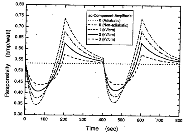
FIG. 5. Dynamical photoresponsivity \mathcal{R}_{ph}(t) as a function of time for different ac-component amplitudes \mathcal{E}_m=0, 1, 2, and 3 kV/cm. The static photoresponsivity \mathcal{R}_{ph}^0 with \mathcal{E}_m=0 (dotted curve) is also included in the figure for the sake of convenience.
