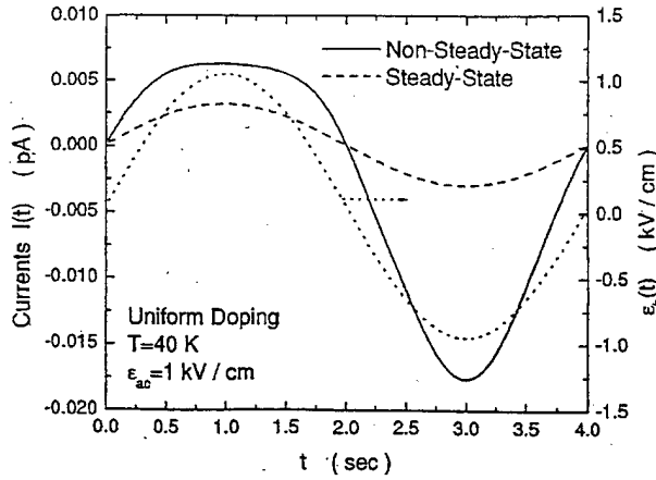
FIG. 1. Calculated time dependence of electron sequential-tunneling currents I(t) = \mathcal{A}[J^{\mu_0}[\mathcal{E}_b] + \Delta J_{na}(t)] (left scale) for nonadiabatic [ \Delta J_{na}(t) \neq 0 , solid curve] and adiabatic [ \Delta J_{na}(t) = 0 , dashed curve], and an applied ac electric field \mathcal{E}_b(t) (right scale) for T=40 K and \mathcal{E}_{ac}=1 kV/cm with uniform doping inside GaAs quantum wells.
