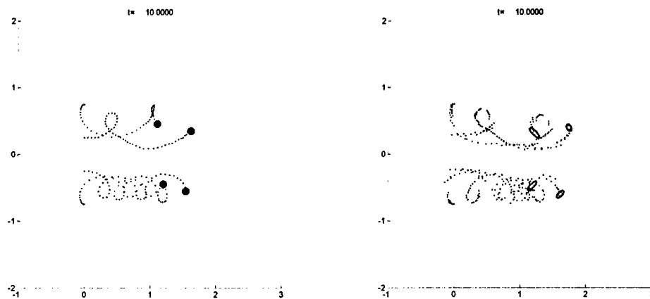
Figure 1. Surface layer observation system for subsurface layer estimation. [left: underlying truth by control run with surface (blue) and sub-surface (red) ocean dipole; right: successful data assimilation with parameter estimation]
