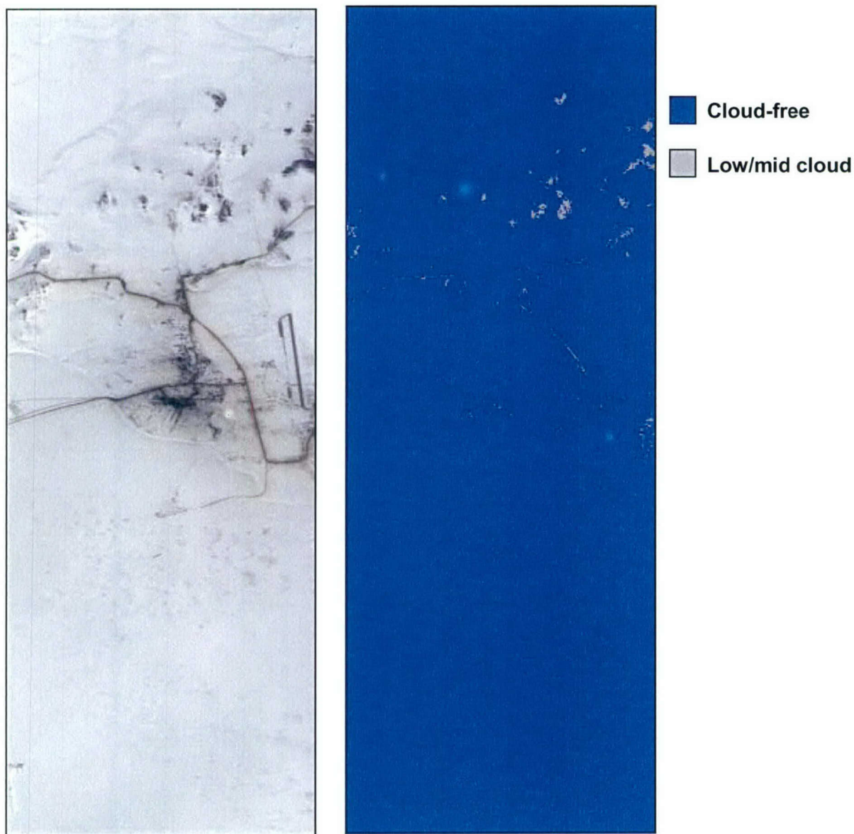
Figure 2-8 Hyperion image collected in the Bering Sea, displaying clear conditions over both snow-covered ice and land. The scene was taken on 20 April 2002 at 2318 UTC. The algorithm computed the cloud amount for the scene to be 0.7%.
