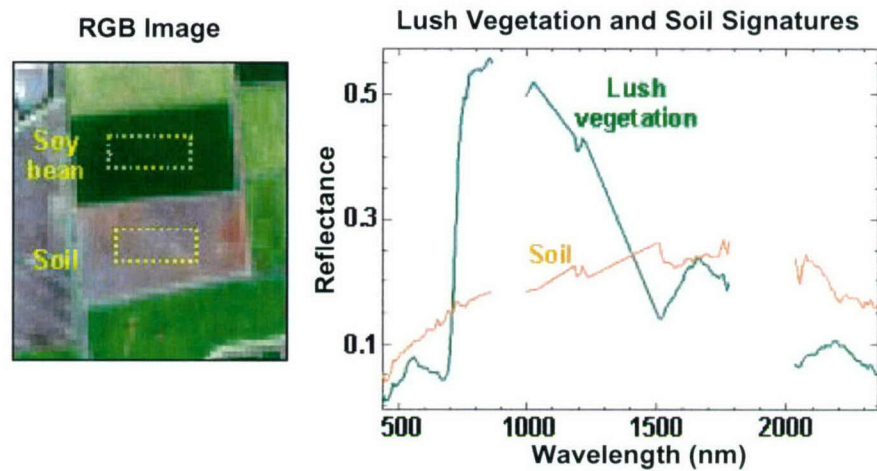
Figure 4-6 Sample areas of soybean and soil in the Coleambally image. Regions of interest are selected as shown on the Hyperion image to include a lush vegetative area in the soybean field and a bare region in the soil area. The mean spectra of the regions are used to demonstrate a two-class unmixing analysis of lush vegetation and bare soil.
