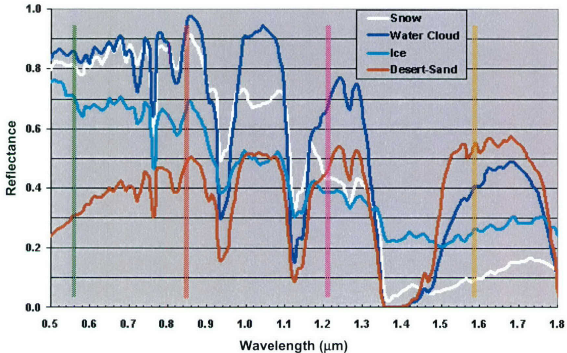
Figure 2-3 Plot of the spectral signatures for four features in the visible, NIR, and SWIR: clouds, surface ice and snow, and desert sand. The red and orange vertical bands represent locations of the NIR and SWIR channels, respectively, used in the desert sand index test. The green and orange bands represent channels used in the snow/ice discrimination tests.
