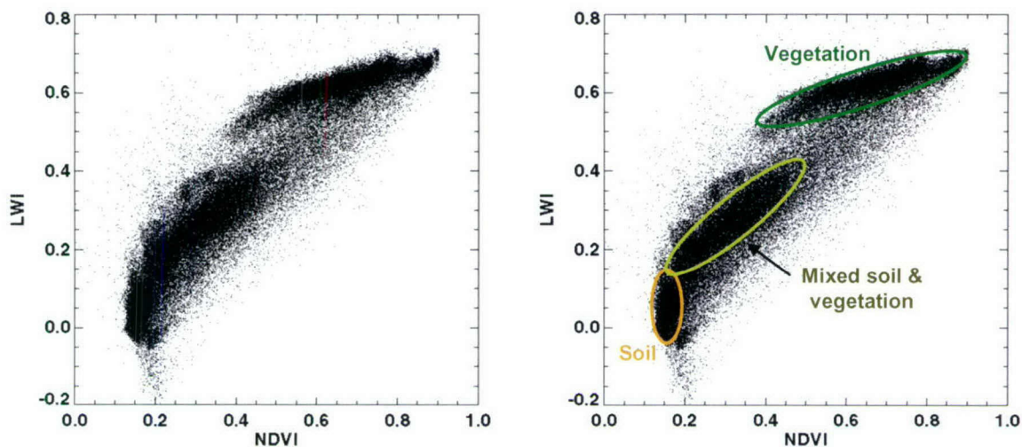
Figure 4-3 Scatter plot of LWI and NDVI derived from Hyperion data over Coleambally. Separate clusters can be delineated from the index plot as shown on the right. The cluster located at lower left consists of data from soil. Some spread in the LWI dimension is seen, indicating different levels of moisture content in the soil. The cluster at the top represents data from vegetation and has a larger response in NDVI than in LWI.
