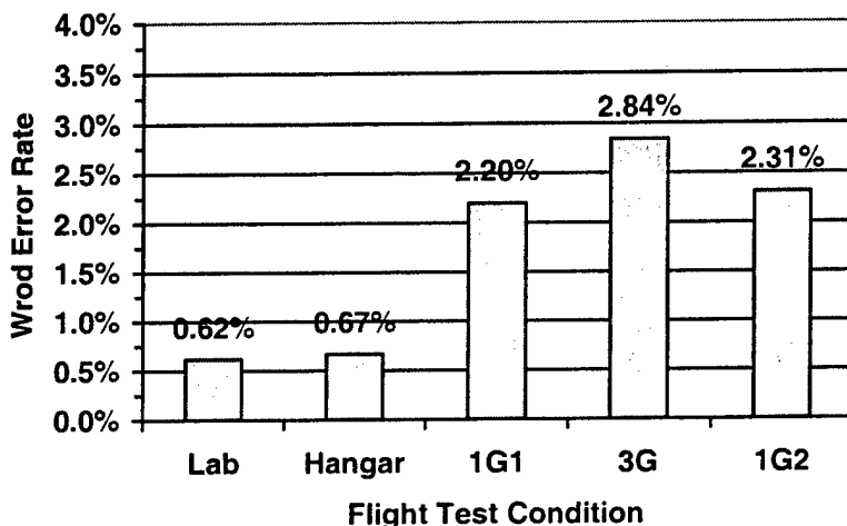
Figure 4. Results for English-8K-030502 Model, WTW=-50, by OV-10A Test Condition
