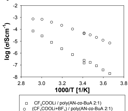
Figure III.2.18. Ionic conductivity of electrolytes comprising CF_3COOLi or CF_3COOLi + BF_3 and poly(AN-co-BuA 2:1)[1.2:1] .
