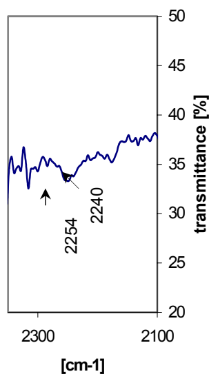
Figure III.2.17. Absorption bands in infrared of the matrix CN groups in the CF_3COOLi+BF_3 / poly(AN-co-BuA 2:1)[1.2:1] electrolyte
