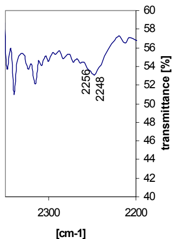
Figure III.2.19. CN groups absorption bands of the electrolyte comprising (CF_3COOLi+SbCl_5) / poly(AN-co-BuA 2:1) [1.2:1].
