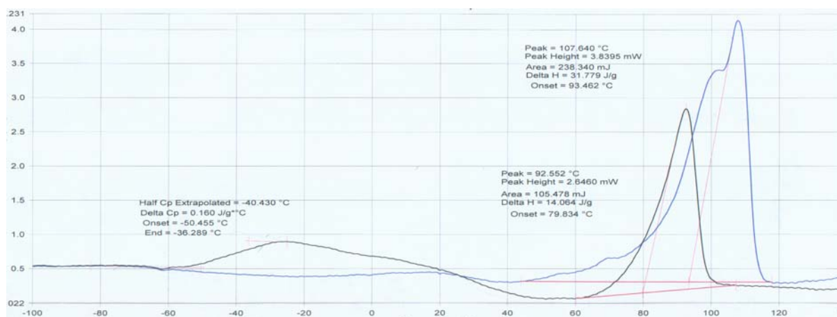
Figure III.2.13. DSC traces of the CF_3COOLi / poly(AN- co -BuA 2:1) [1.2:1] electrolyte.
