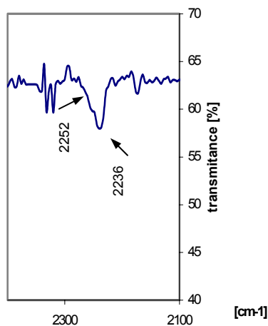
Figure III.2.15. Absorption bands in infrared of the CN group in the \text{CF}_3\text{COOLi} / poly(AN-co-BuA 2:1) electrolyte.
