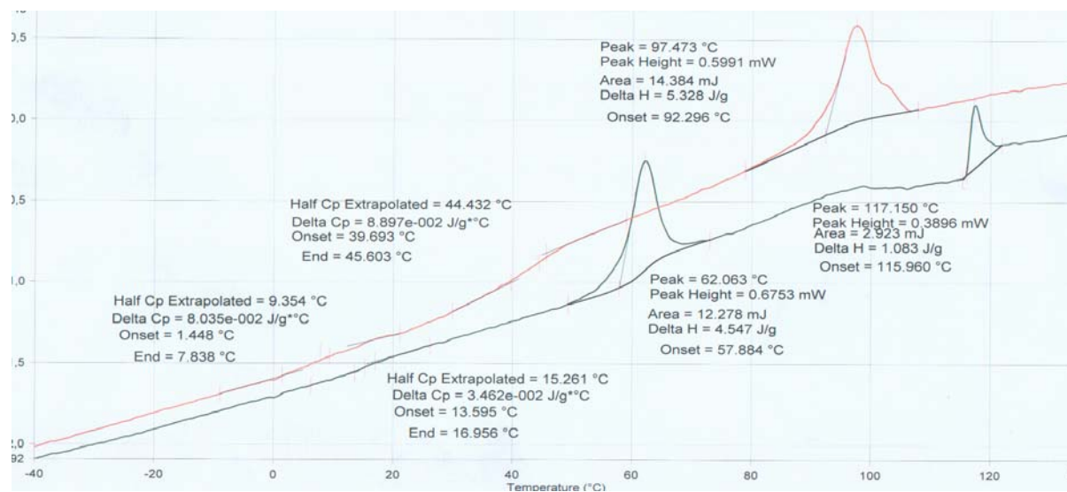
Figure III.2.24. DSC traces of the electrolyte comprising (CF_3COOLi+AlCl_3) / poly(AN-co-BuA 2:1)[1.2:1]
