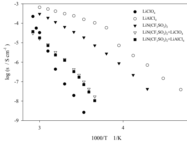
Figure II.2.7. Changes in ionic conductivity as a function of inverse temperature for electrolytes composed of butyl acrylate and acrylonitrile copolymer doped with various salts.
