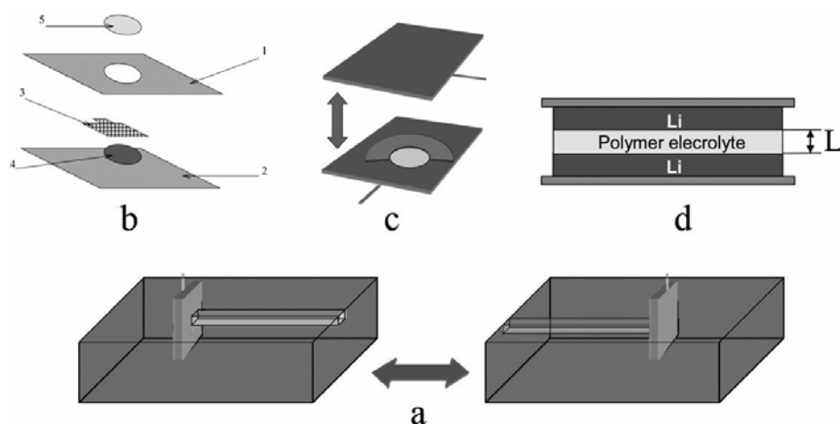
Figure IV.3.2. Measurement cell.
