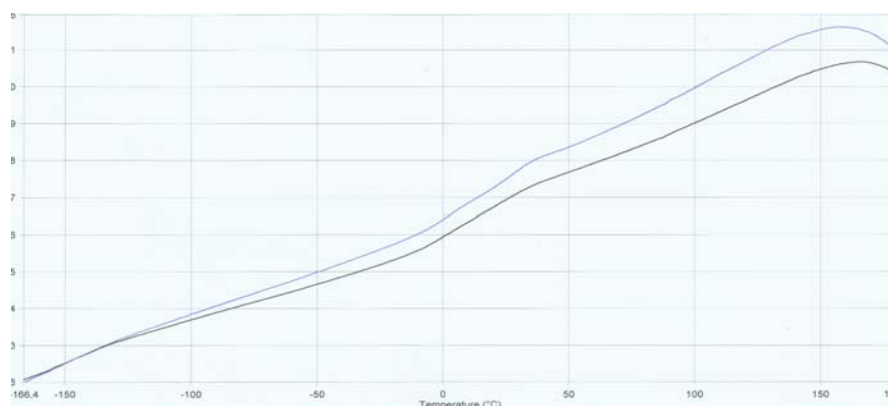
Figure III.2.21. DSC traces of the electrolyte comprising (CF_3COOLi+SbF_5) / poly(AN-co-BuA\ 2:1)[1.2:1] .
