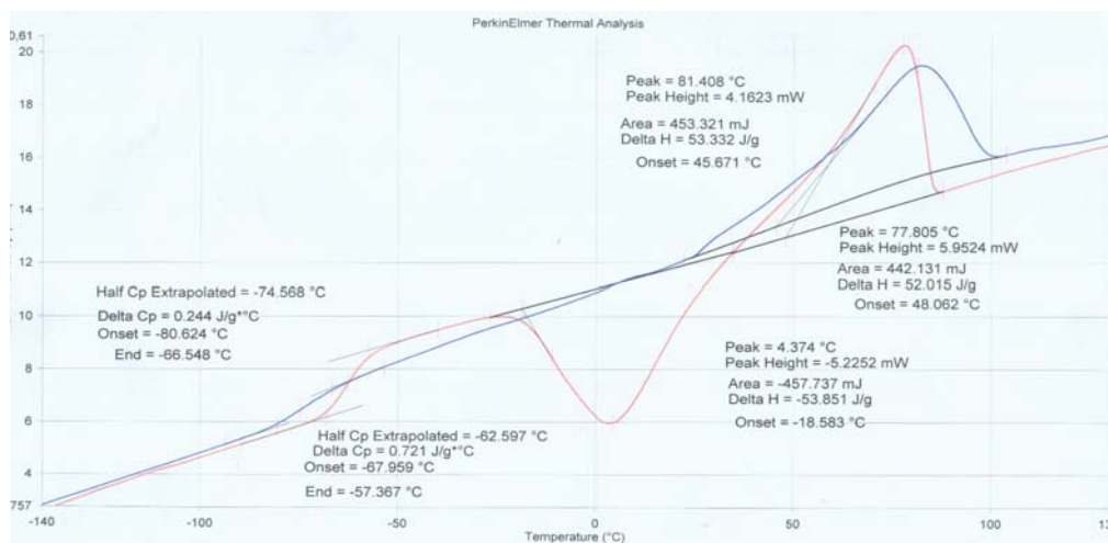
Figure III.2.16. DSC traces of the (CF_3COOLi+BF_3) / poly(AN-co-BuA 2:1) [1.2:1] electrolyte
