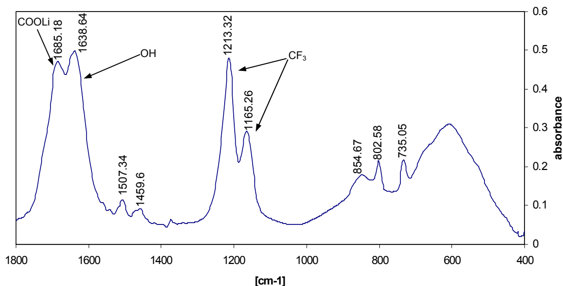
Figure III.2.12. FTIR spectrum of the lithium trifluoroacetate and AlCl_3 reaction products.
