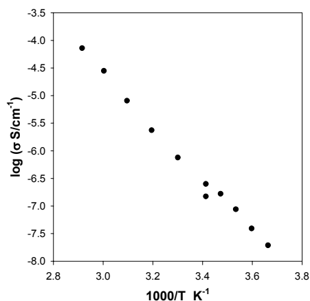
Figure III.2.14. Conductivity of an electrolyte comprising \text{CF}_3\text{COOLi} and poly(AN-co-BuA 2:1) [1.2:1].
