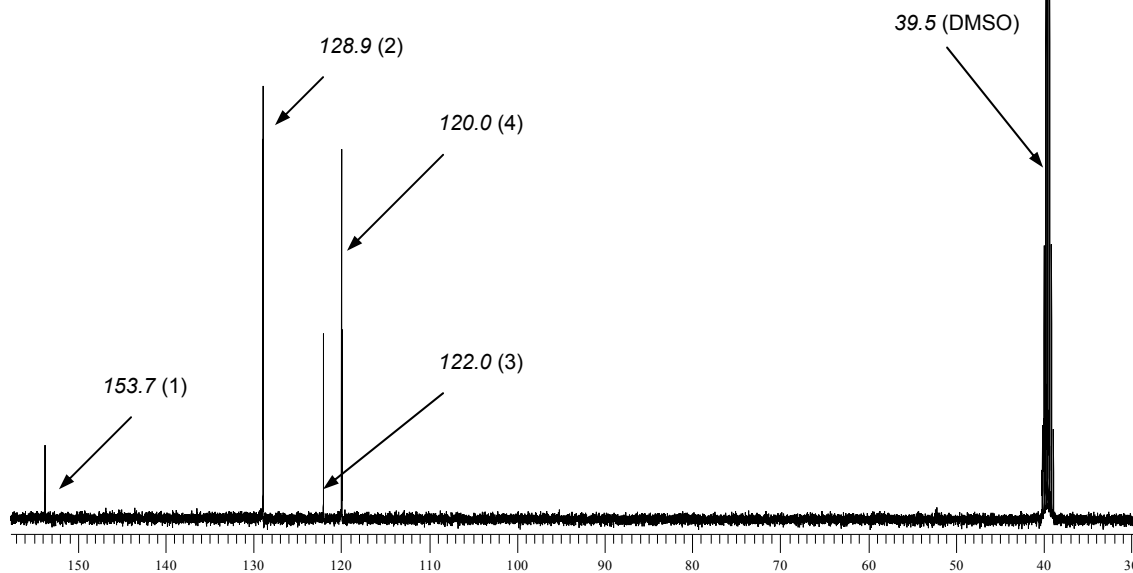
Figure III.1.1. ^{13}\text{C} NMR spectrum of LiDPhP (DMSO- d_6 )
