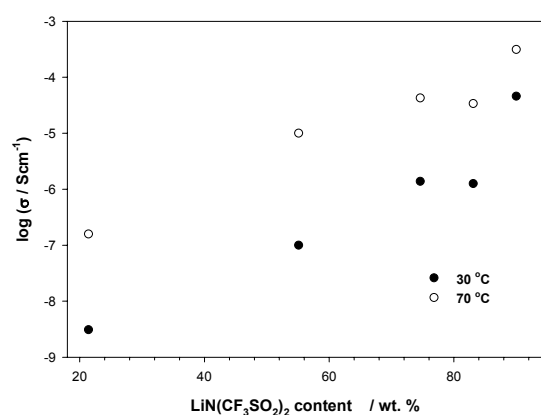
Figure II.1.5. Conductivity isotherms determined at (●) 30 and (○) 70 °C for electrolytes comprising poly(AN-co-BuA 2:1) and LiN(CF 3 SO 2 ) 2 depending on the salt concentration.
