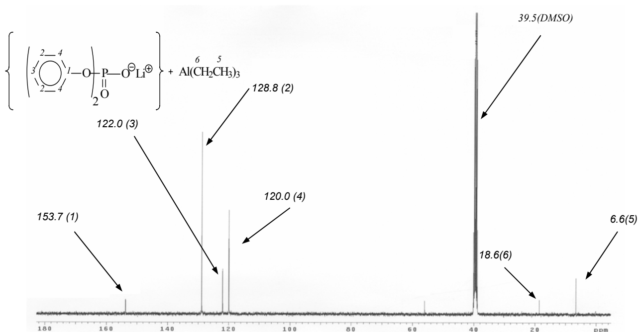
Figure III.1.2. ^{13}\text{C} NMR spectrum of LiDPhP complexed with \text{Al}(\text{C}_2\text{H}_5)_3 (DMSO- d_6 )
