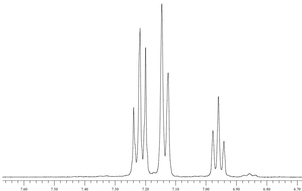
Figure III.1.4. ^1\text{H} NMR spectrum of LiDPhP ( \text{DMSO-d}_6 ).
