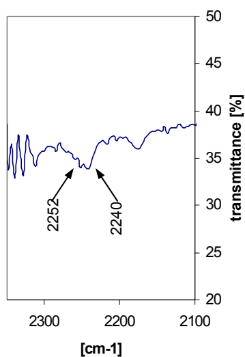
Figure III.2.22. CN groups absorption bands of the electrolyte comprising CF_3COOLi+SbF_5 / poly(AN-co-BuA\ 2:1)[1.2:1] .
