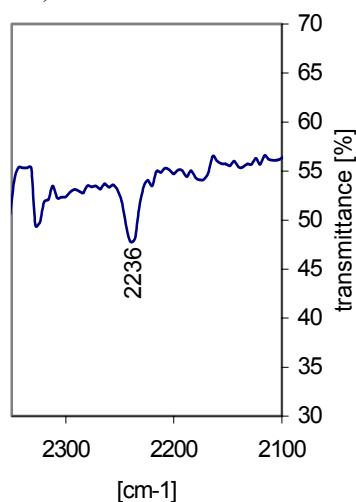
Figure III.2.27. CN groups absorption bands of the electrolyte comprising (CO_2Li)_2 and poly(AN-co-BuA 2:1)[1.2:1] .
