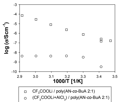
Figure III.2.26. Ionic conductivity of electrolytes comprising CF_3COOLi and CF_3COOLi+AlCl_3 / poly(AN-co-BuA 2:1) .
