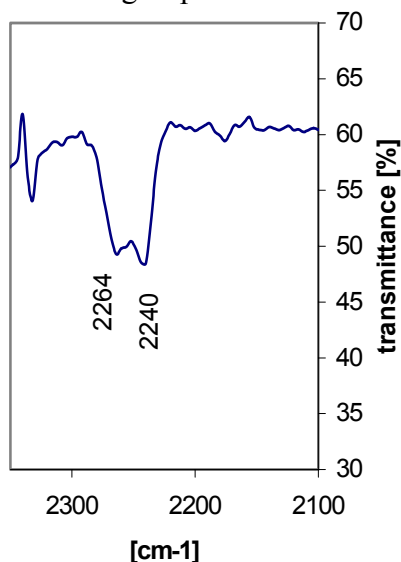
Figure III.2.30. CN groups absorption bands of the electrolyte comprising (\text{CO}_2\text{Li})_2 + \text{BF}_3 and poly(AN-co-BuA 2:1)[1.2:1].
