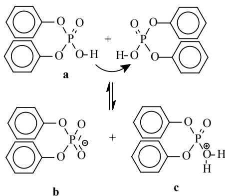
Scheme of diphenylphosphoric acid autodissociation
