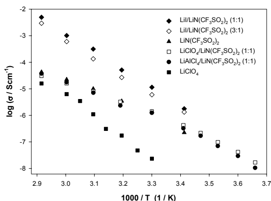
Figure II.1.3. Ionic conductivity of electrolytes based on poly(AN-co-BuA 2:1) and mixtures of lithium salts with LiN(CF 3 SO 2 ) 2 (molar ratio of salt : AN m. u. in the copolymer = 1.2).
