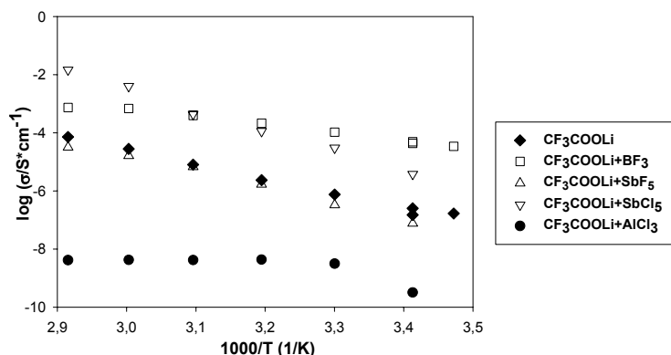
Figure III.2.39. Conductivity of electrolytes comprising poly( AN-co-BuA 2:1) and \text{CF}_3\text{CO}_2\text{Li} [1.2:1] and its complexes with various Lewis acids.
