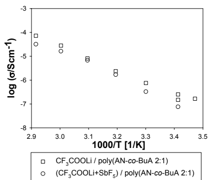
Figure III.2.23. Ionic conductivity of electrolytes comprising CF_3COOLi or CF_3COOLi+SbF_5 and poly(AN-co-BuA\ 2:1)[1.2:1] .
