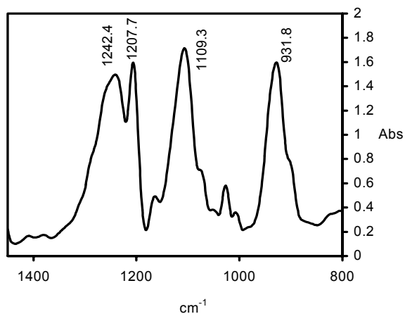
Figure III.1.9. FTIR spectrum of the LiDPhP complex with Al(C 2 H 5 ) 3 .
