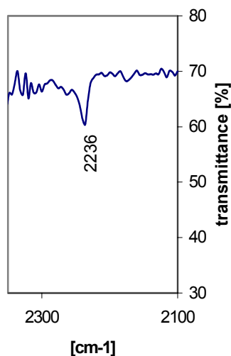
Figure III.2.25. CN groups absorption bands of the electrolyte comprising poly(AN-co-BuA 2:1)[1.2:1] / CF_3COOLi+AlCl_3 .
