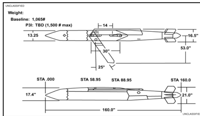
Figure 1 JSOW Dimensions (From TOPGUN MANUAL Chapter 33)
