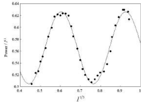
Figure 2: Normalized sub-threshold power vs. I^{1/3} fit to Cosine, verifying a three-wave interaction.
