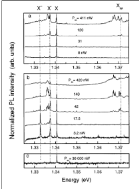
Figure 2: PL spectra of an individual QD at T=4\text{K} for a number of excitation powers P_{\text{ex}} (shown in the figure) and different pump photon energies. a) h\nu=1.684\text{eV} , b) h\nu=1.536\text{eV} and c) h\nu=1.433\text{eV} . All spectra are normalized to the maximum value of their PL amplitude and are vertically shifted for clarity.
