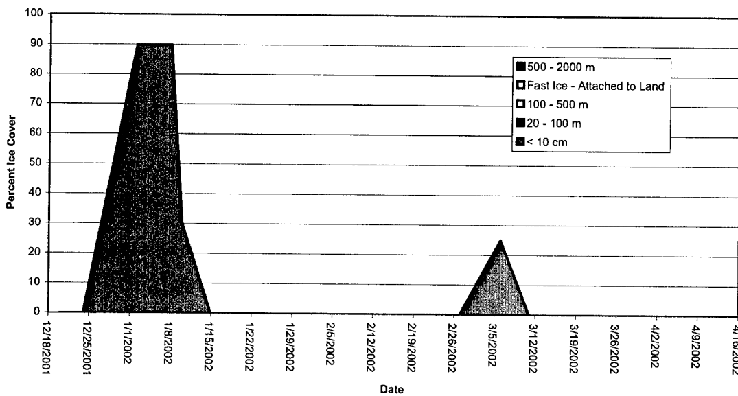
Figure 37. Ice thickness and ice floe size for winter 2001-2002 (NOAA)
