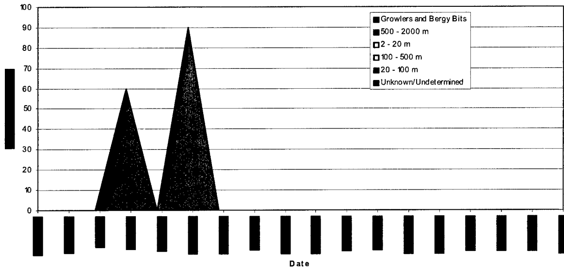
Figure 39. Ice thickness and ice floe size for winter 2001-2002 (Environment Canada)
