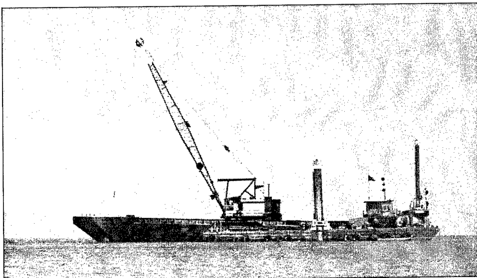
Figure 6. 1999 dredging layout
