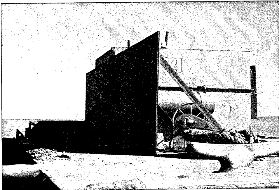
Figure 9. Scow release operators protective barrier
