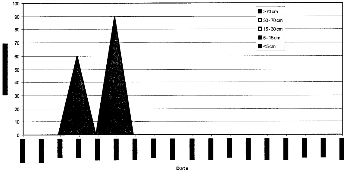
Form of Ice - Size of Ice Floe on Lake Erie Near Toussaint River for Winter 2001-2002 (Env. Canada)
