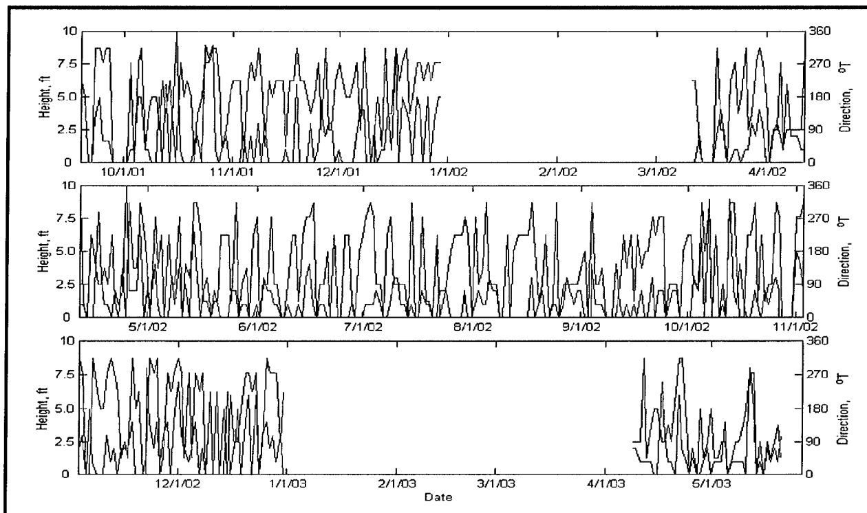
Figure 47. Daily forecast of wave heights near Toussaint River from Great Lakes Forecasting System
