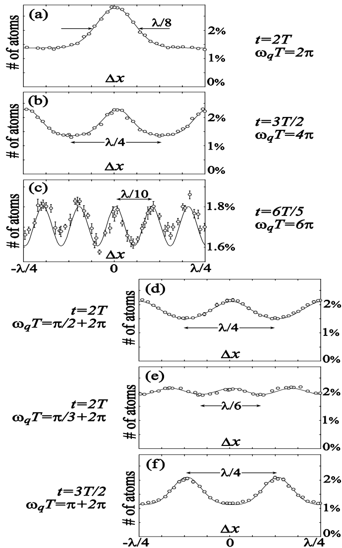
FIG. 1: Images of atomic density generated with the Talbot-Lau effect: (a) - (c) is the atomic density measured at various times. (d) and (e) shows the atomic density measured at t = 2T for different values of the recoil phase \omega_q T . The difference between these curves and those of (a) are due to matter-wave interference. (f) shows a shift in the position of the maxima compared to (b) due to matter-wave interference. Open circles are data and the solid lines are fits.
