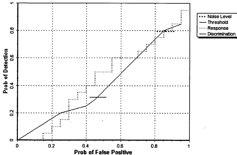
Figure 2. TM-5 EMU hand held blind grid probability of detection for response and discrimination stages versus their respective probability of false positive over all ordnance categories combined.
