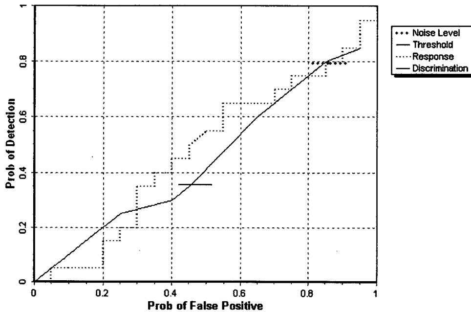
Figure 4. TM-5 EMU hand held blind grid probability of detection for response and discrimination stages versus their respective probability of false positive for all ordnance larger than 20 mm.
