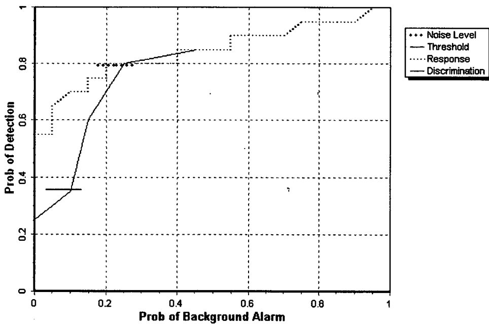
Figure 5. TM-5 EMU hand held blind grid probability of detection for response and discrimination stages versus their respective probabilities of background alarm for all ordnance larger than 20 mm.
