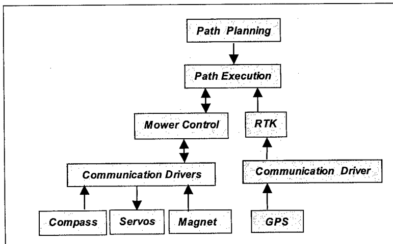
► FIGURE 2 Miami Red Blade system overview (below) and control algorithm overview (right)
