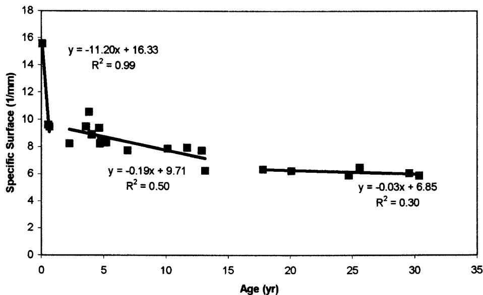
Figure 30. Specific surface decrease with time in the 2000-1 firm core.
