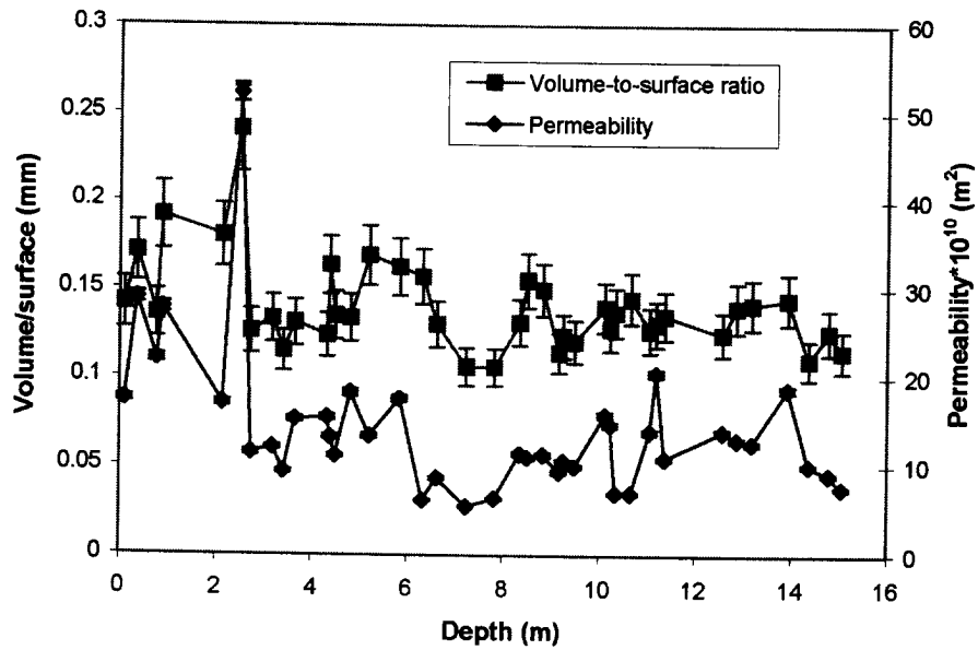
Figure 46. Volume-to-surface ratio of the pores in the 2000-1 firm core. Note the similarity between the permeability and volume-to-surface curves.
