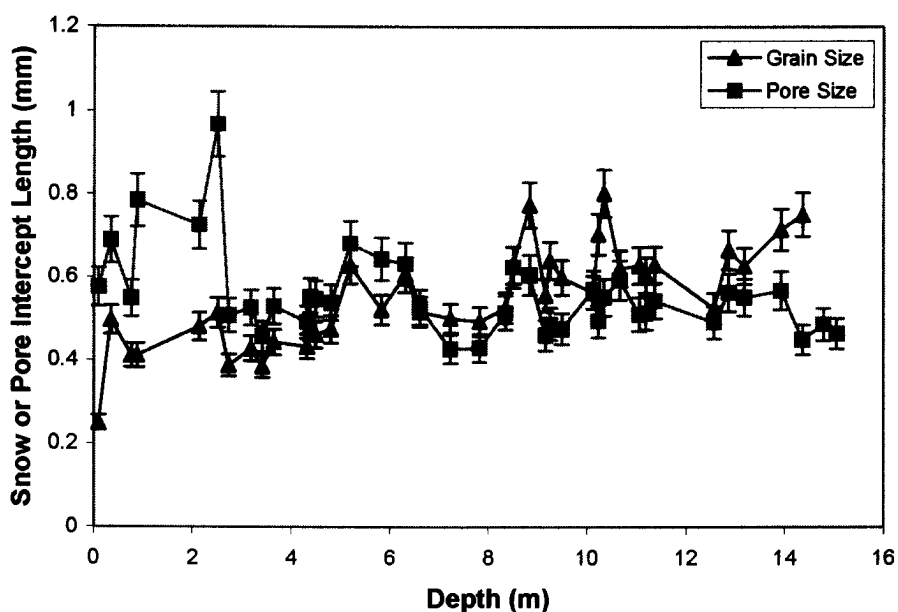
Figure 16. Mean grain and pore intercept lengths of the homogeneous 2000-1 firn core samples.
