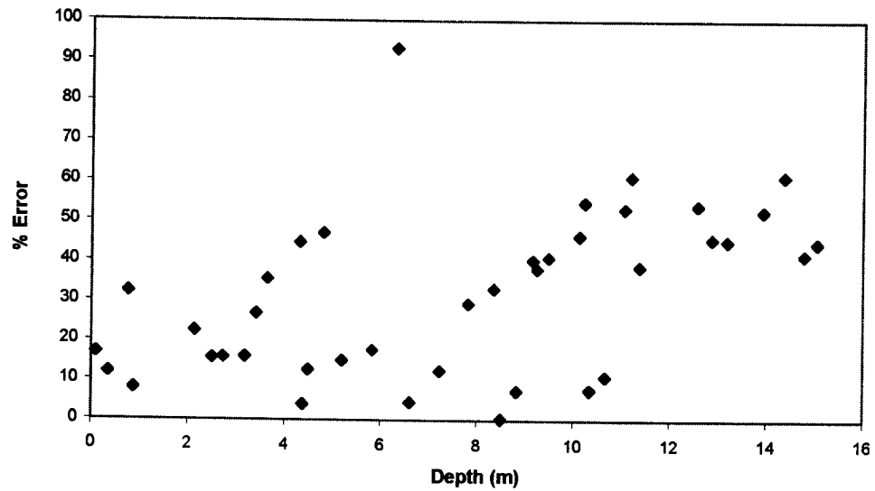
Figure 48. Percent error of each sample permeability predicted by Equation 22.
