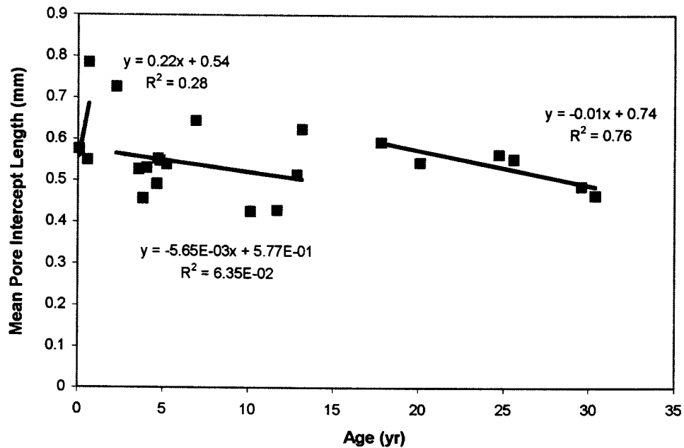
Figure 31. Pore size change with time.
