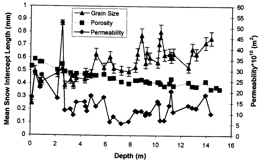
Figure 45. Grain size and porosity increase with depth, which does not follow the permeability pattern of increase and then decrease.
