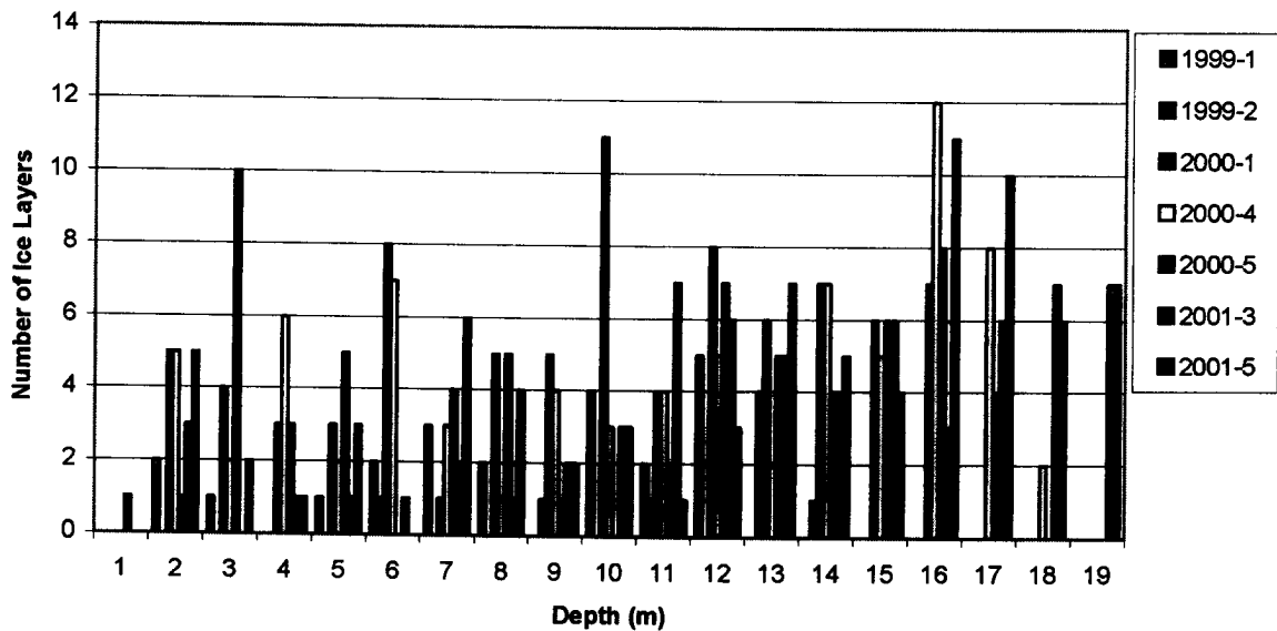
Figure 9. Frequency and distribution of single-grained ice layers throughout the ITASE firm cores.
