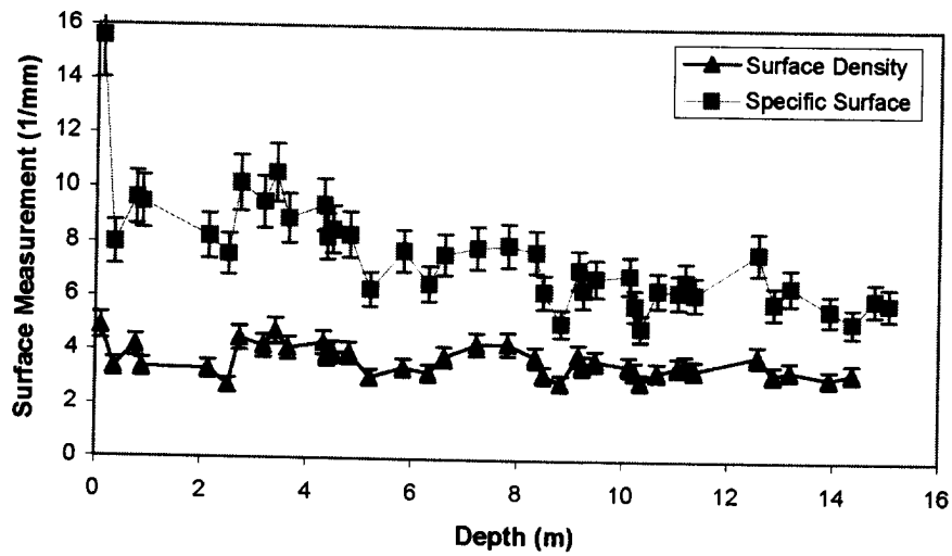
Figure 20. Snow surface measurements of the 2000-1 firn core.
