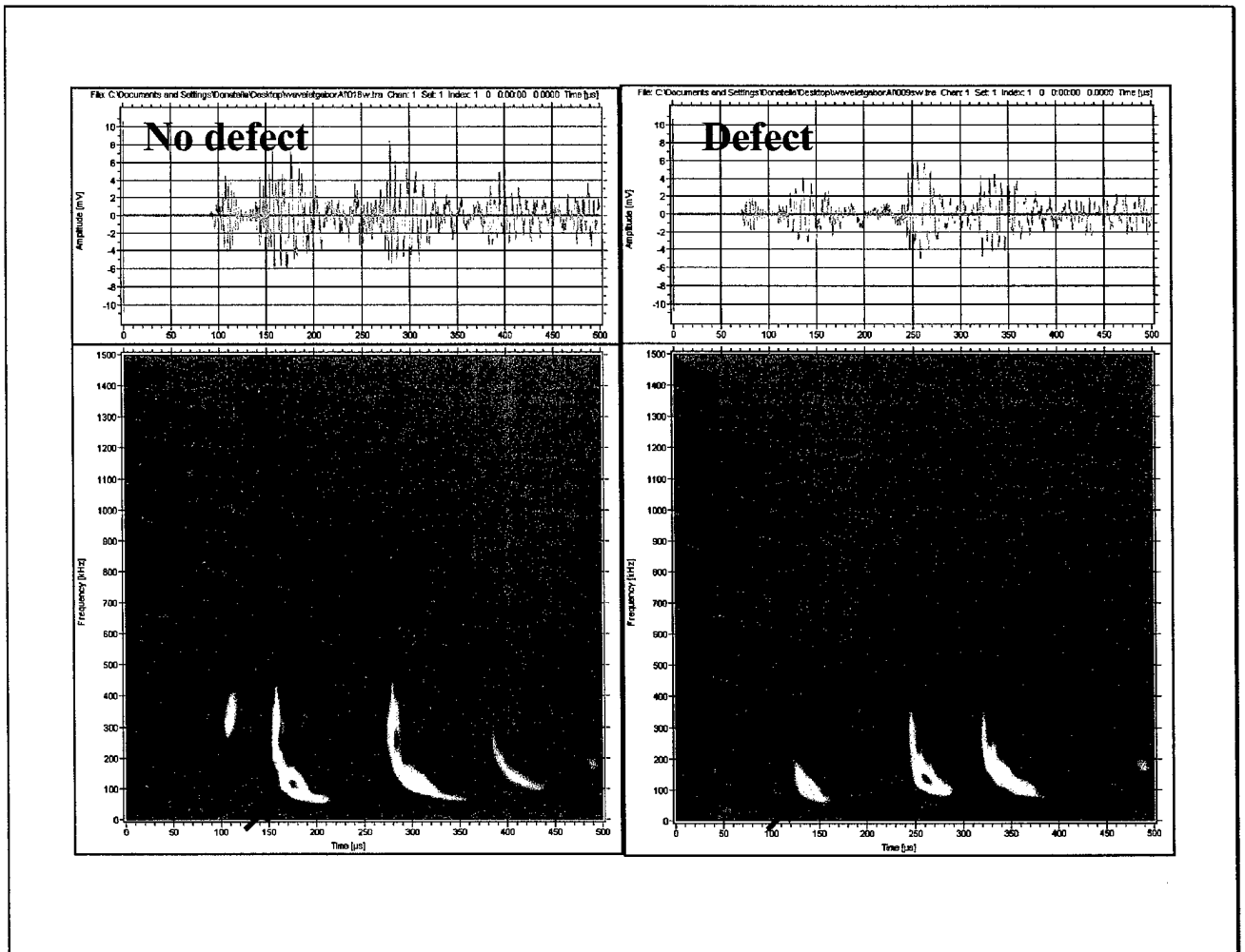
Figure 3.11. Lamb wave signal changes due to presence of skin crack. The wavelet modal analysis diagrams show a loss of energy in lower frequency mode and corresponding ultrasonic energy shift to higher modes when crack discontinuity is present in the sample. The lower mode in the diagrams is highlighted by an arrow.
