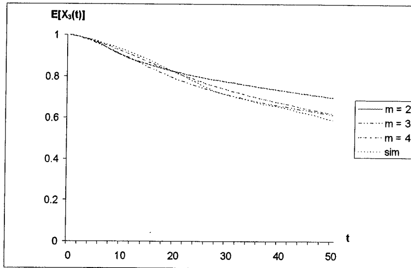
Figure 5: Graph of R(t) = E[X_3(t)] for Varying Truncation Levels
