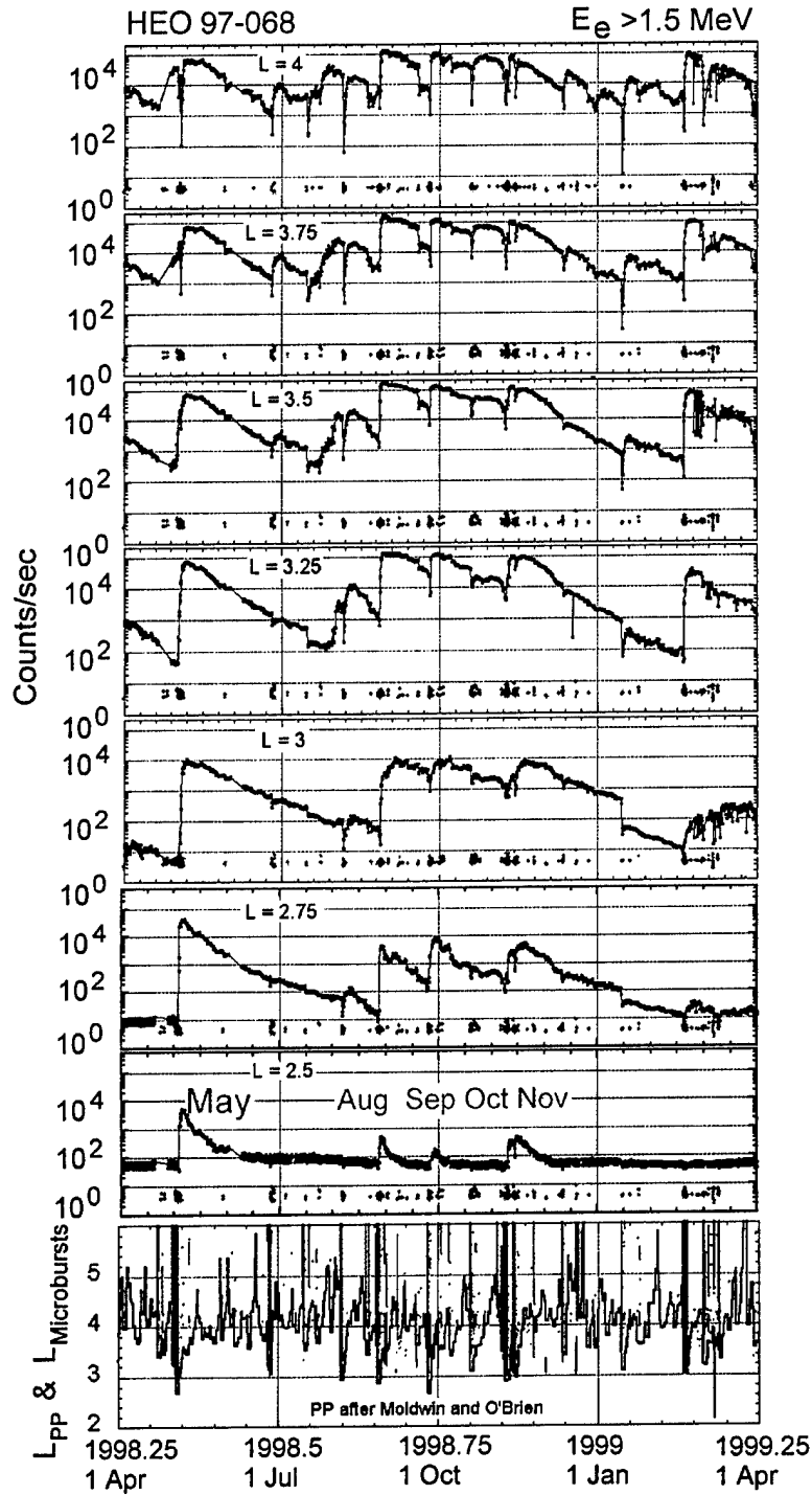
Figure 1. Daily average >1.5 \text{ MeV} electron intensity for several L values during the period April 1998 to April 1999 (upper panels) and the estimated plasmopause position ( L_{PP} , black line) and the range of L where microbursts ( L_{Microbursts} ; blue and red markings) were observed by SAMPEX (bottom panel)
