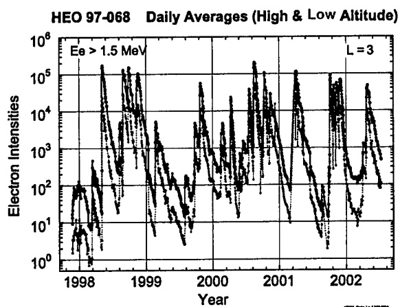
Figure 2. Plot of high (black) and low (red) E_e > 1.5 MeV fluxes at L=3 .
