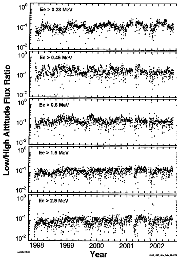
Figure 6. Ratio of four years of low to high altitude electron fluxes from HEO 97-068 L = 4 for several energies.
