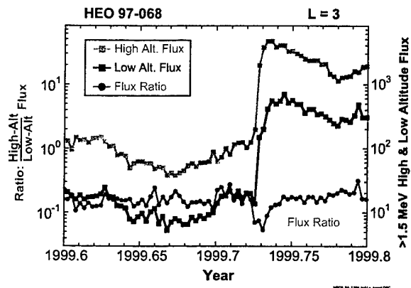
Figure 5. Comparison of low and high altitude HEO3 fluxes and their ratio at L = 3 for the interval around the 22 Sept. 1999 magnetic storm.
