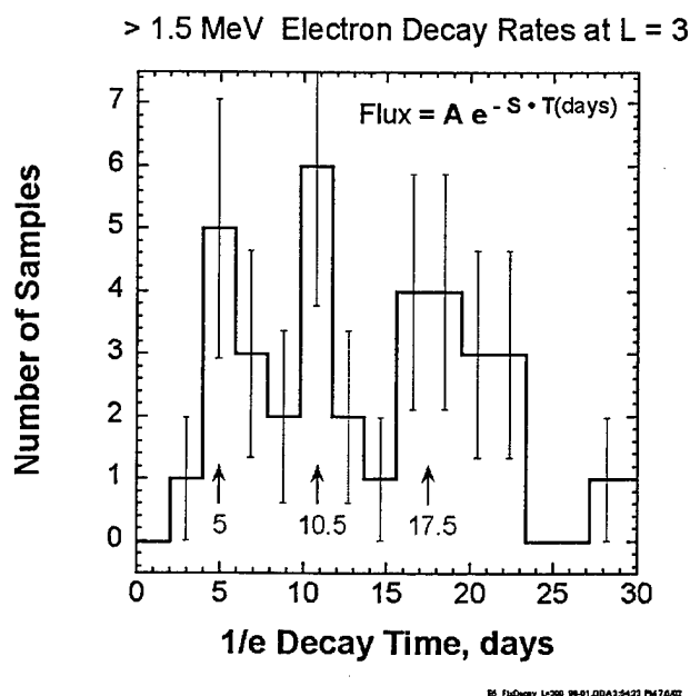
Figure 9. Histogram of e-folding decay times, in days, for the data in Figure 8.
