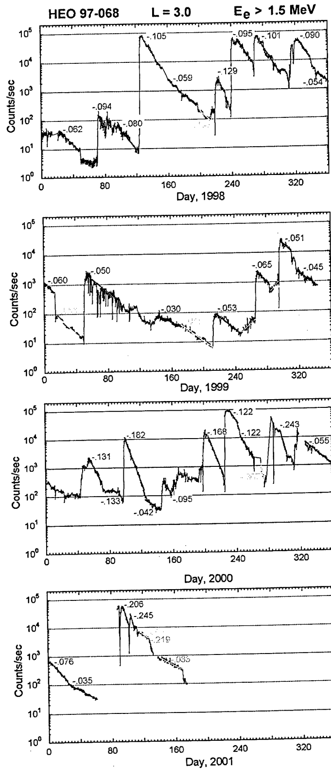
Figure 8. Flux history of electrons >1.5 \text{ MeV} at L = 3 .
