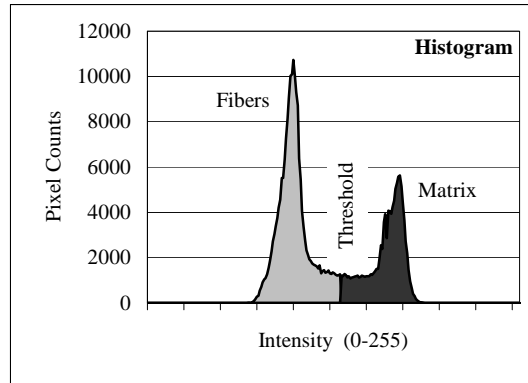
FIGURE 6.6.6.5.4(a) Typical histogram of gray scale fiber and matrix distribution.
