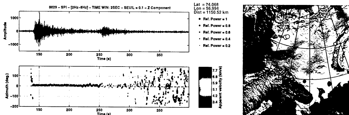
Fig. 6.5.7. Time evolution of the parameters of propagation for an event of group G3 recorded at SPITS.
