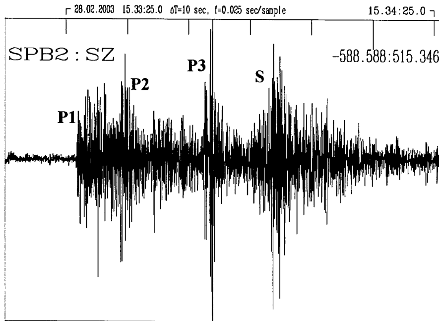
Fig. 6.3.3. SPITS recordings of earthquake in the rift zone. At least three P-arrivals can be seen. The trace has been high-pass filtered above 4 Hz.
