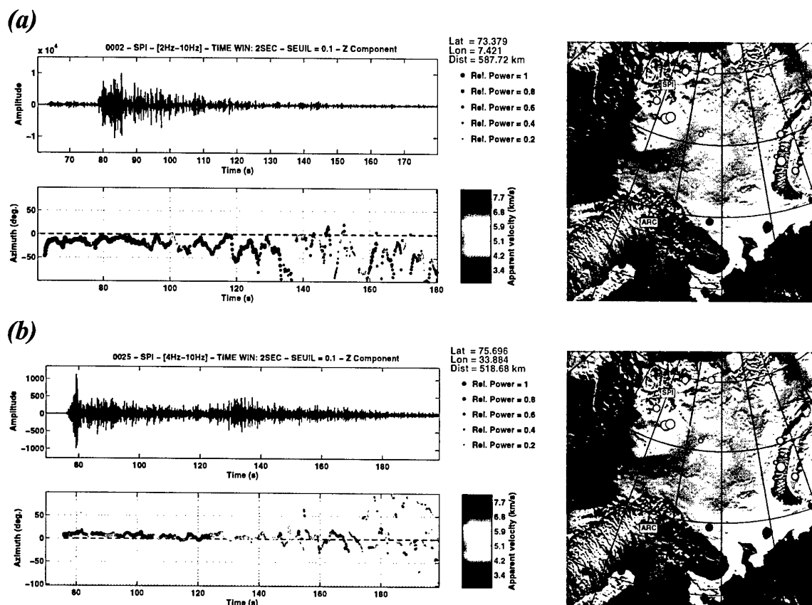
Fig. 6.5.7. Time evolution of the parameters of propagation for an event of group G3 recorded at SPITS.
