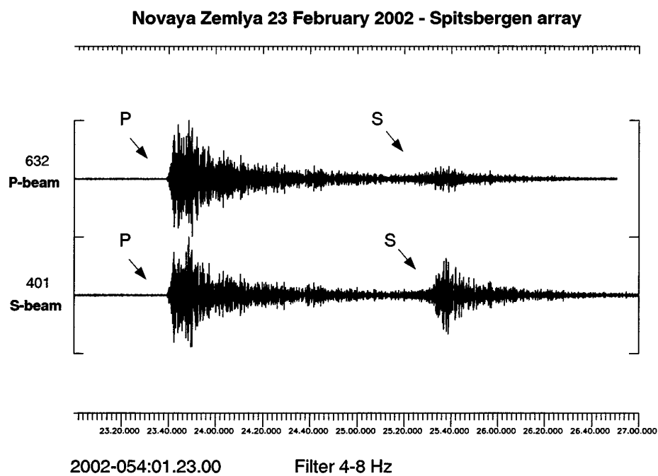
Fig. 6.1.4. Spitsbergen P and S beams for the Novaya Zemlya event on 23 February 2002
