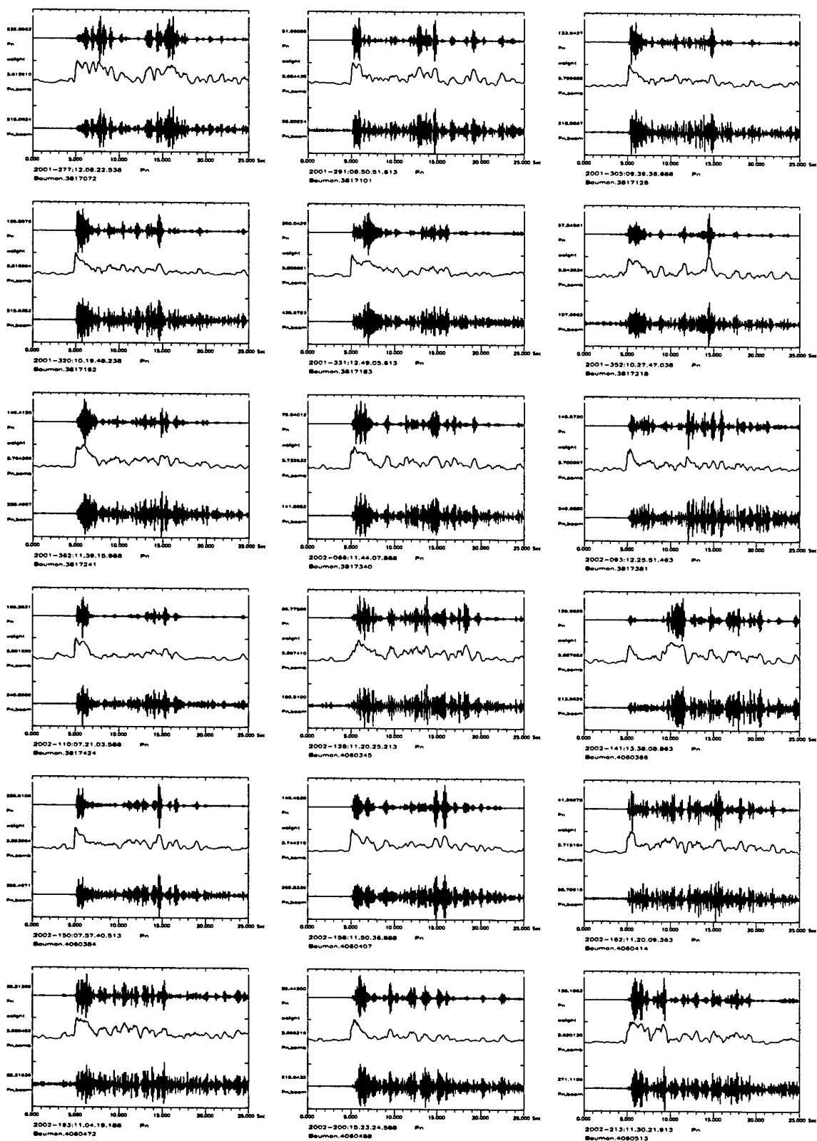
Appendix C. ARCES recordings of 18 explosions in the Bauman open-pit mine. For each panel we show the Pn beam (bottom), the semblance coefficient (middle) and the Pn beam weighted with the semblance coefficient.
