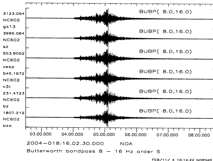
Fig. 4.4.3. The above figure shows from top to bottom, data observed in site NC602 for GS13, Tele-dyne 20171, Guralp CMG-ESPV, Guralp CMG-3TV, Guralp CMG-3T and KS54000. The data is filtered with a Butterworth bandpass filter of order 5 and band 8 - 16 Hz. The numbers annotated to the left side, is maximum amplitude in counts for the corresponding trace.
