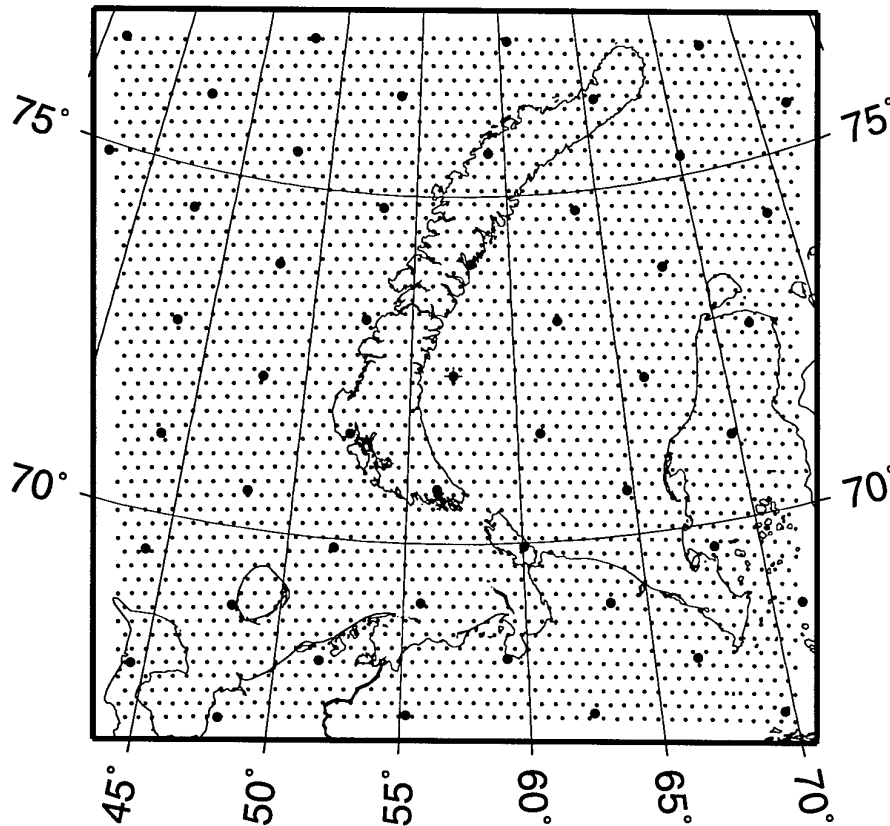
Fig. 6.1.3. Example of a map of the "beampacking" grid system used by the NORSAR GBF, in this case constructed around an initial event location in the Kara Sea. This dense grid is used to refine locations provided by the initial grid (shown here as large dots). The distance between the grid nodes is 0.2 degrees.
