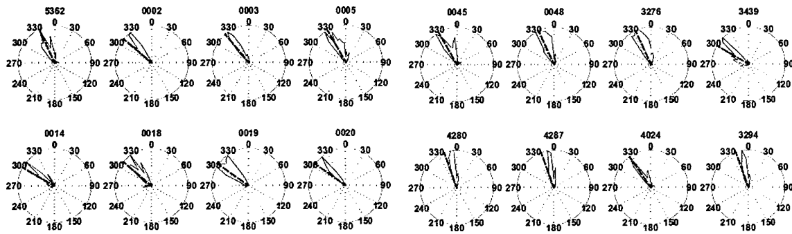
Fig. 6.5.5. Energetic distributions of the directions of propagation for all the events of the group G1 observed at ARCES.
