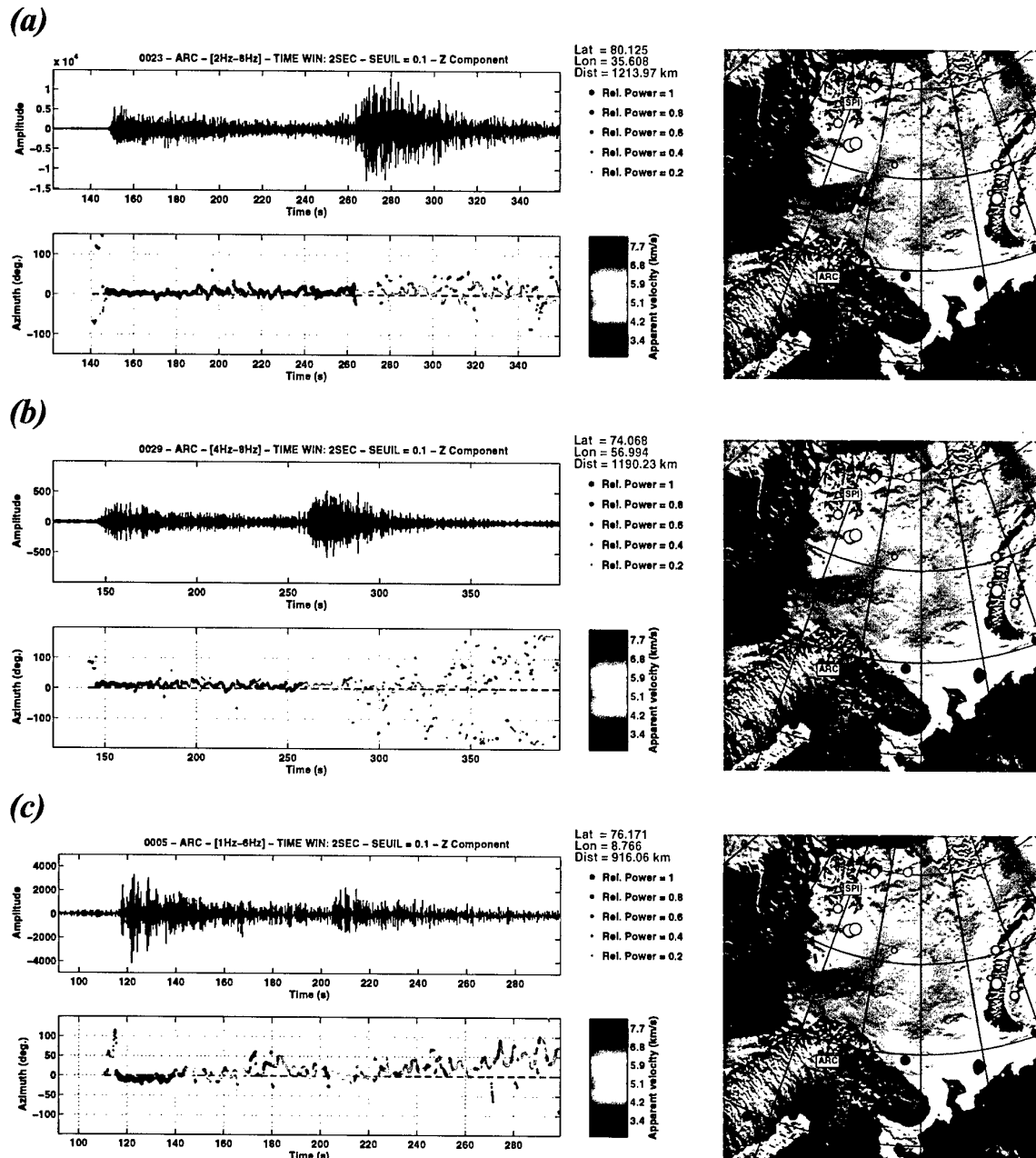
Fig. 6.5.4. (a) Typical time evolution of the parameters of propagation for an event of group G2 observed at ARCES. (b) Idem for an event of group G3. (c) Idem for an event of group G1. On the right hand side, the propagation paths for the 3 events considered are represented.
