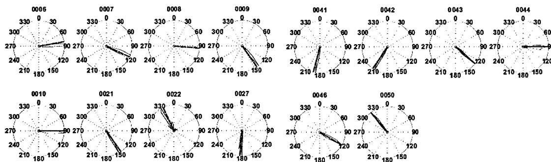
Fig. 6.5.3. Energetic distributions of the directions of propagation for all the events of group G4 observed at ARCES.
