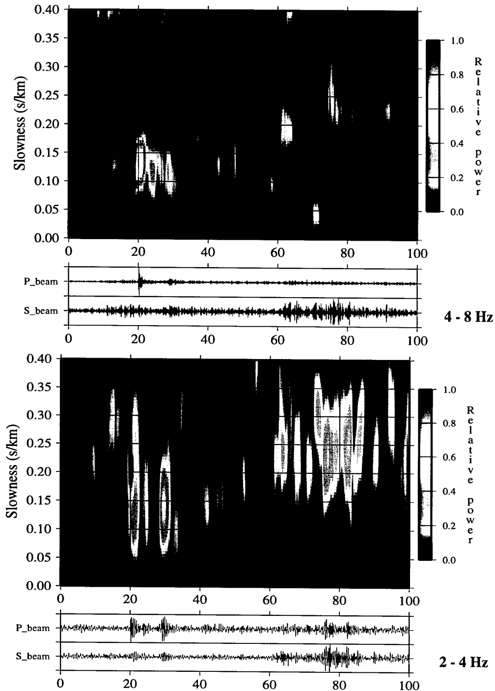
Fig. 6.6.5. The upper panel shows a 4-8 Hz ARCES vespagram of the Rasvumchorr compact shot shown in Figure 6.6.4. The slowness space is scanned at a back-azimuth of 120 degrees, using a window length of 2 seconds sampled at 0.1 second steps. The ARCES center instrument (A0), the C- and D-ring instruments are used in the calculations. The P beam shown below the vespagram is steered with an apparent velocity of 7.5 km/s, and 4.3 km/s is used for the S beam. The lower panel show similar plots for the 2-4 Hz frequency band.
