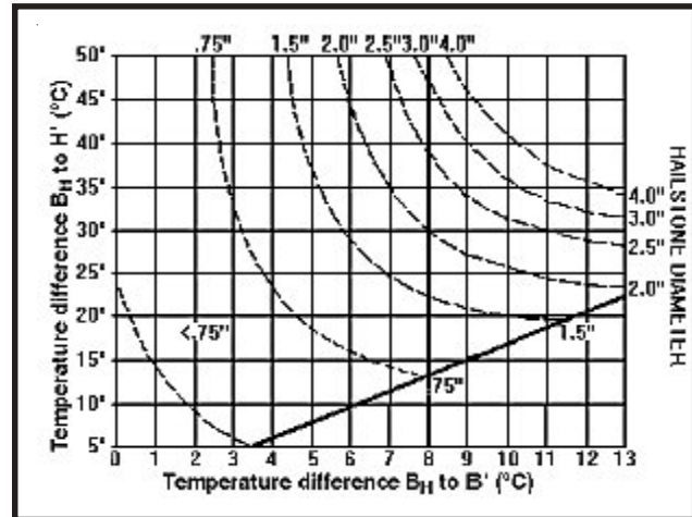
Figure 3-21. Preliminary Hail Size Nomogram.
