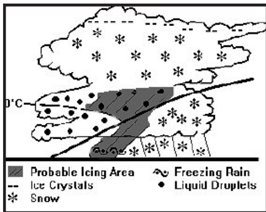
Figure 2-64. Icing with a Warm Front.
