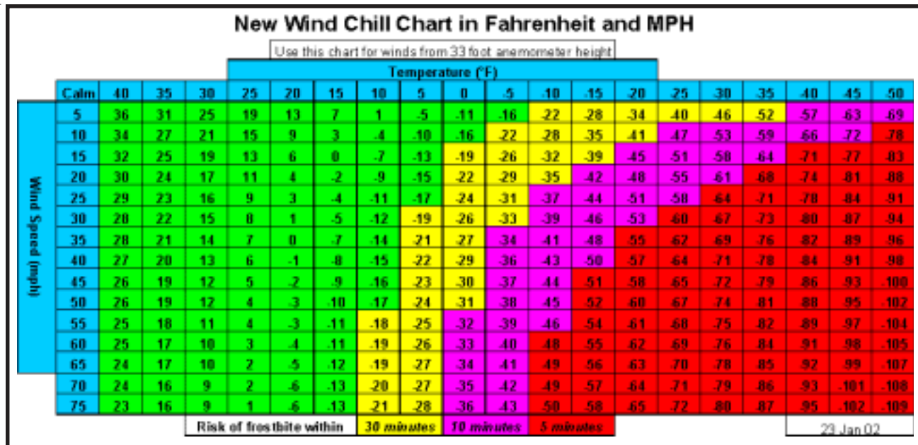
Figure 1-29. Wind Chill Temperature (WCT) Index Chart with 33-Foot Garrison Anemometer Height (degrees Fahrenheit and MPH).
