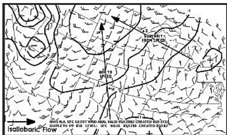
Figure 1-16. Isolobaric Flow. Isolobaric winds flow perpendicular to isobaric contours from an isobaric high to an isobaric low.
