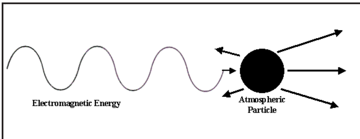
Figure 2-98. Mie Scattering.
