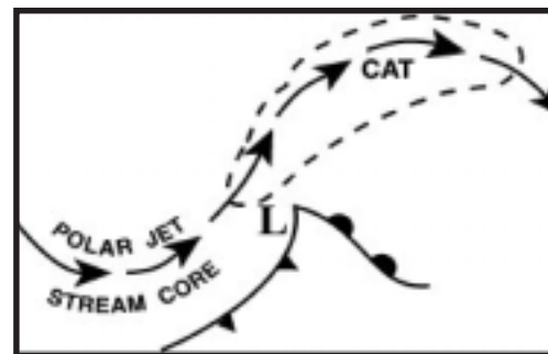
Figure 2-28a. CAT and Surface Cyclogenesis. The figure shows CAT near the jet stream core northeast of the surface low development.
