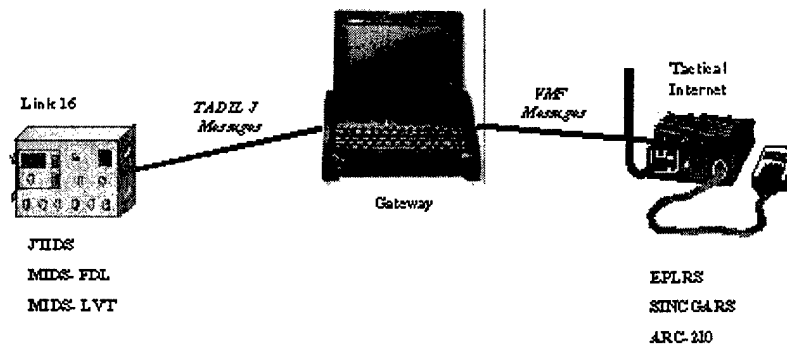
Figure 2-7 Trivial Link 16/VMF Gateway
