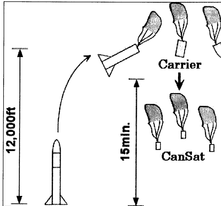
Figure 4-19 Low Altitude Deployment
