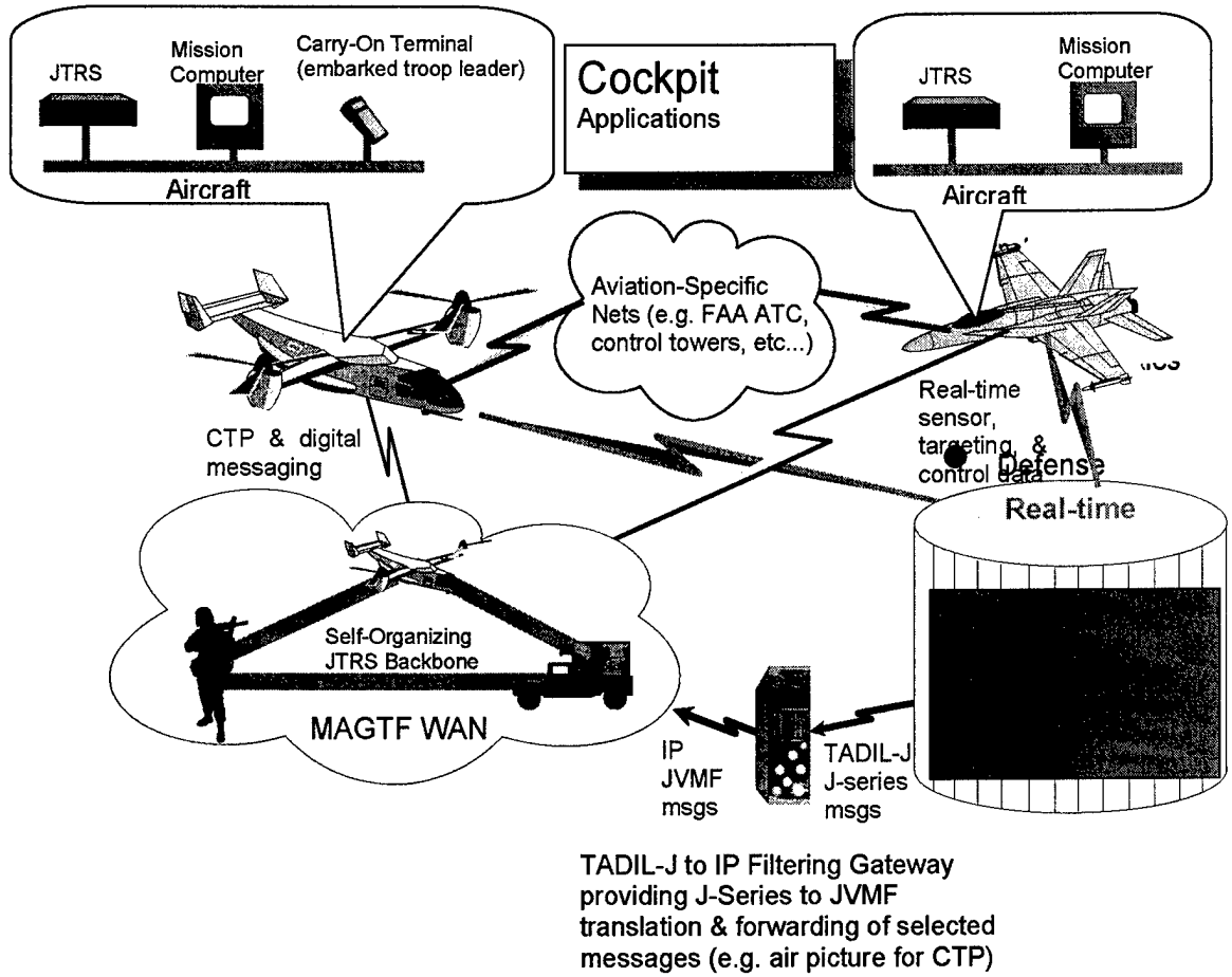
Figure 3-6 Marine Corps Architecture Vision
