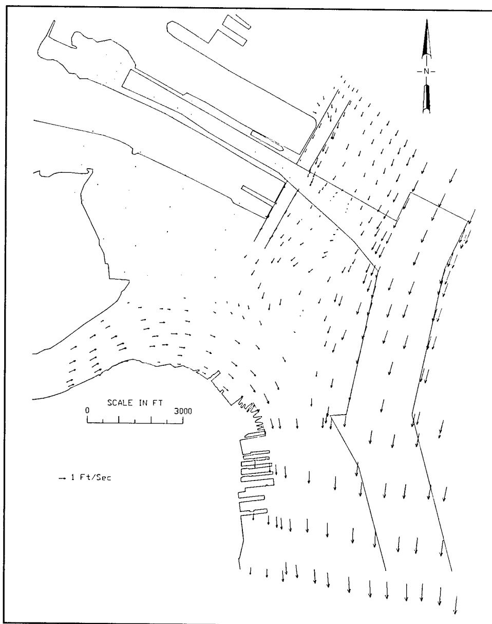
Figure 8. Port Jersey currents, ebb tide
