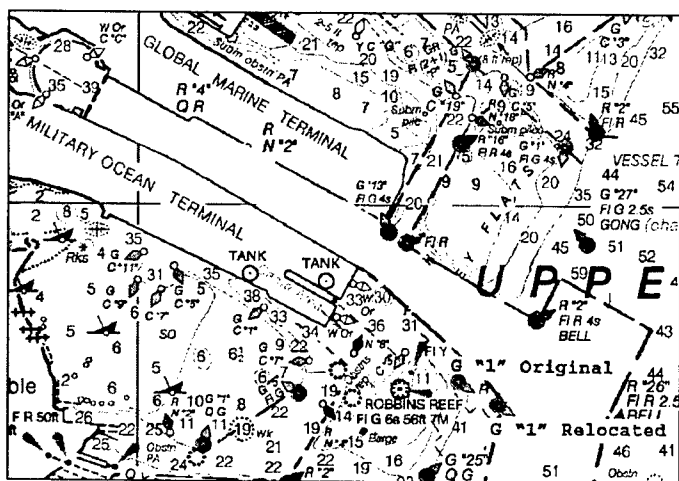
Figure 17. Buoy G "1" moved to channel's edge
