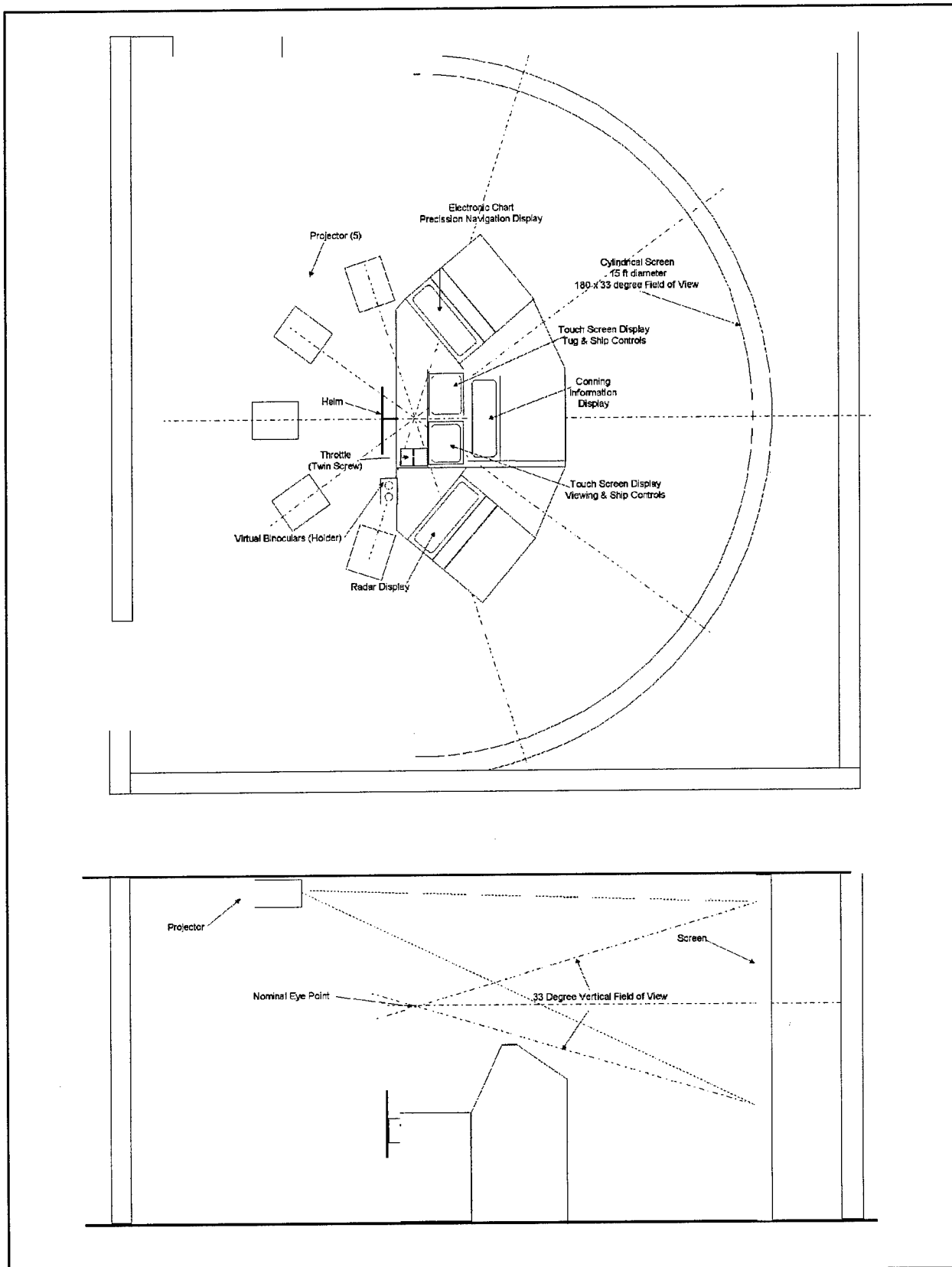
Figure 11. ERDC simulator layout
