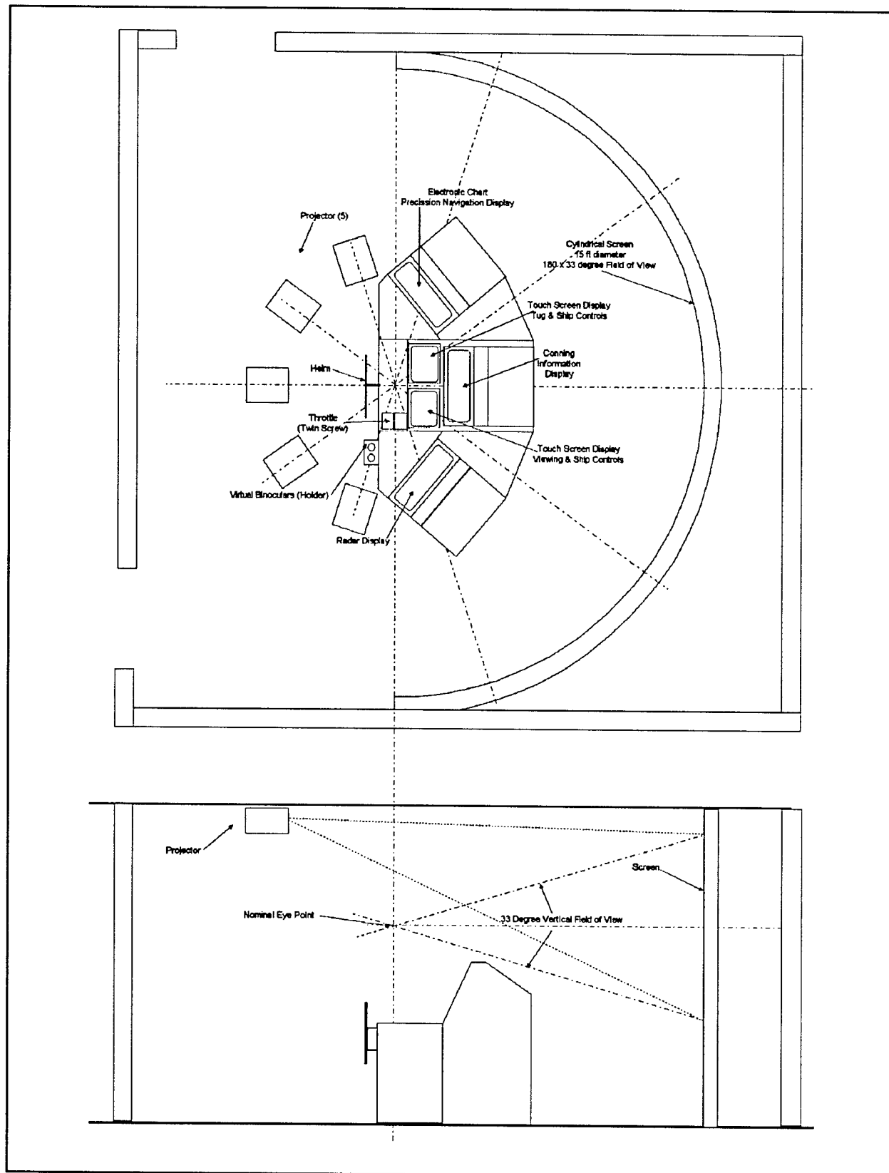
Figure 12. Arrangement of ERDC Ship/Tow Simulator bridge module
