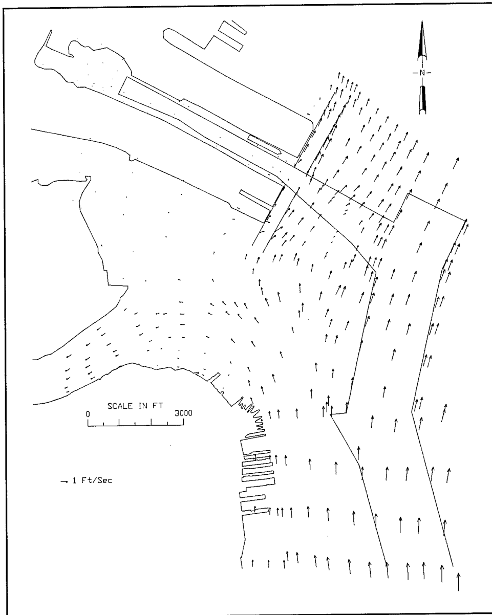
Figure 9. Port Jersey currents, flood tide
