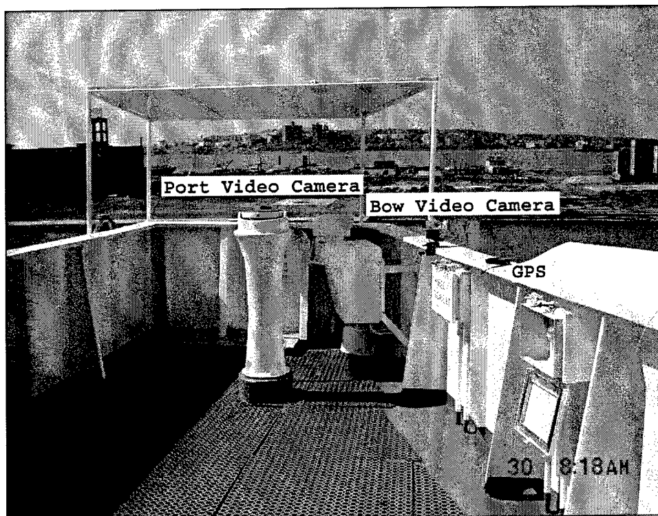
Figure 6. Camera setup on port wing
