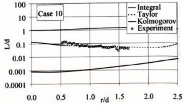
Figure 9. Comparison between calculated and experimental length scales L_{\text{int}} , L_{\text{Kol}} , L_{\text{Tay}} at x/d=10 , 6MPa, 1.9m/s, T=132 K.
