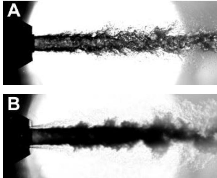
Figure 25. Binary liquid N 2 /GHe system at A: 1.0 MPa, B: 6.0 MPa. d_{\text{LN}_2} = 1.9 mm, v_{\text{LN}_2} = 5 m/s, v_{\text{He}} = 100 m/s, T_{\text{LN}_2} = 97 K, T_{\text{He}} = 280 K (from Mayer and Smith, in press).
