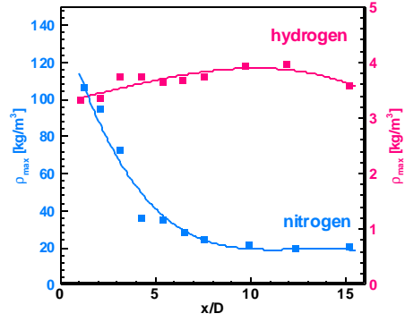
Figure 28. Evolution of the maximum nitrogen and hydrogen density downstream of the injector for test case D4.
