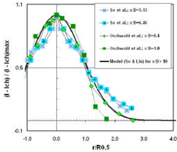
Figure 14. (a) Plots of normalized intensity vs. normalized radius for \text{LN}_2 injected into \text{GN}_2 , at x/D=12.2 , at subcritical, near-critical, and supercritical pressures (Chehroudi et al. (2000)). (b) Similar results by Oswald and Schick (1999), and gaseous jet experimental data by So et al. (1990). The solid curve is the self-similar model that represents data from a gaseous jet injected into a gaseous environment. I and I_{ch} are measured intensities in the jet and in the chamber far away from the jet.
