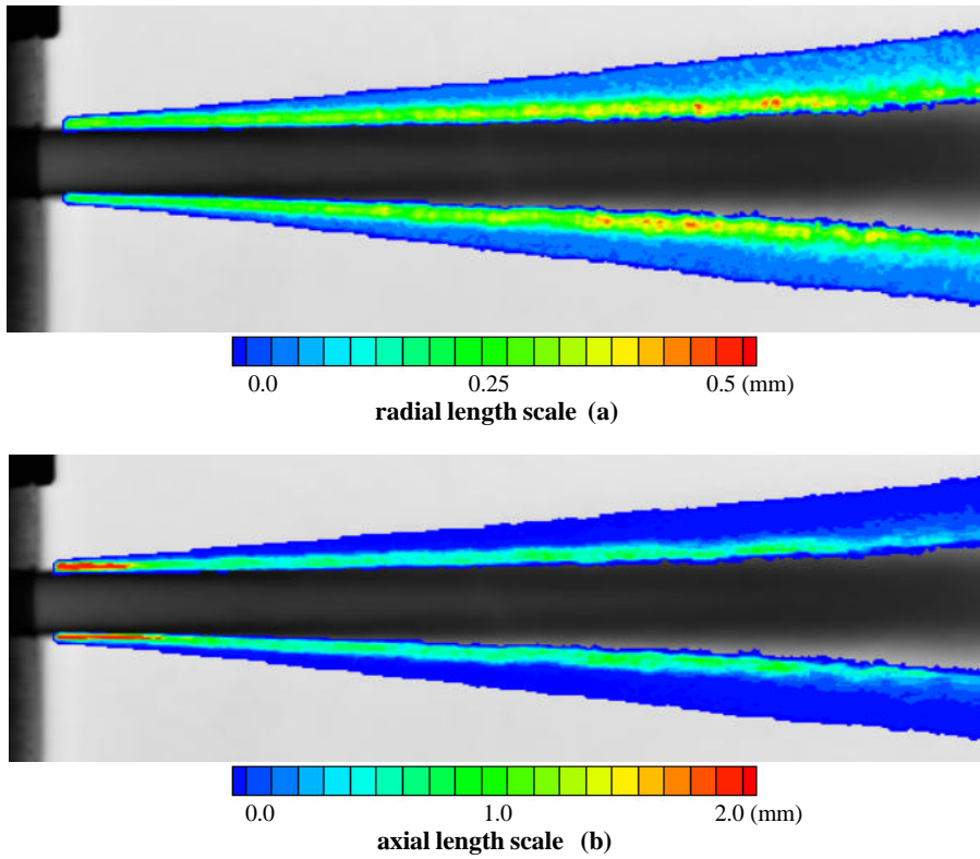
Figure 10. Experimental length scales for \text{LN}_2 into \text{GN}_2 , 4MPa, 123 K.
