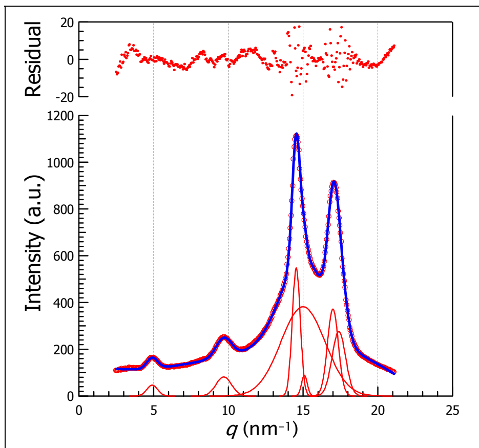
Figure 6. Graphical results of peak fitting analysis, showing WAXS data for 101 spot 1, fit data, and the seven individual components (as listed in table 3) that comprise the fit data. All peak shapes are Gaussian. The variation from the WAXS data of the fit is given as the residual component, indicating the quality of the fit.
