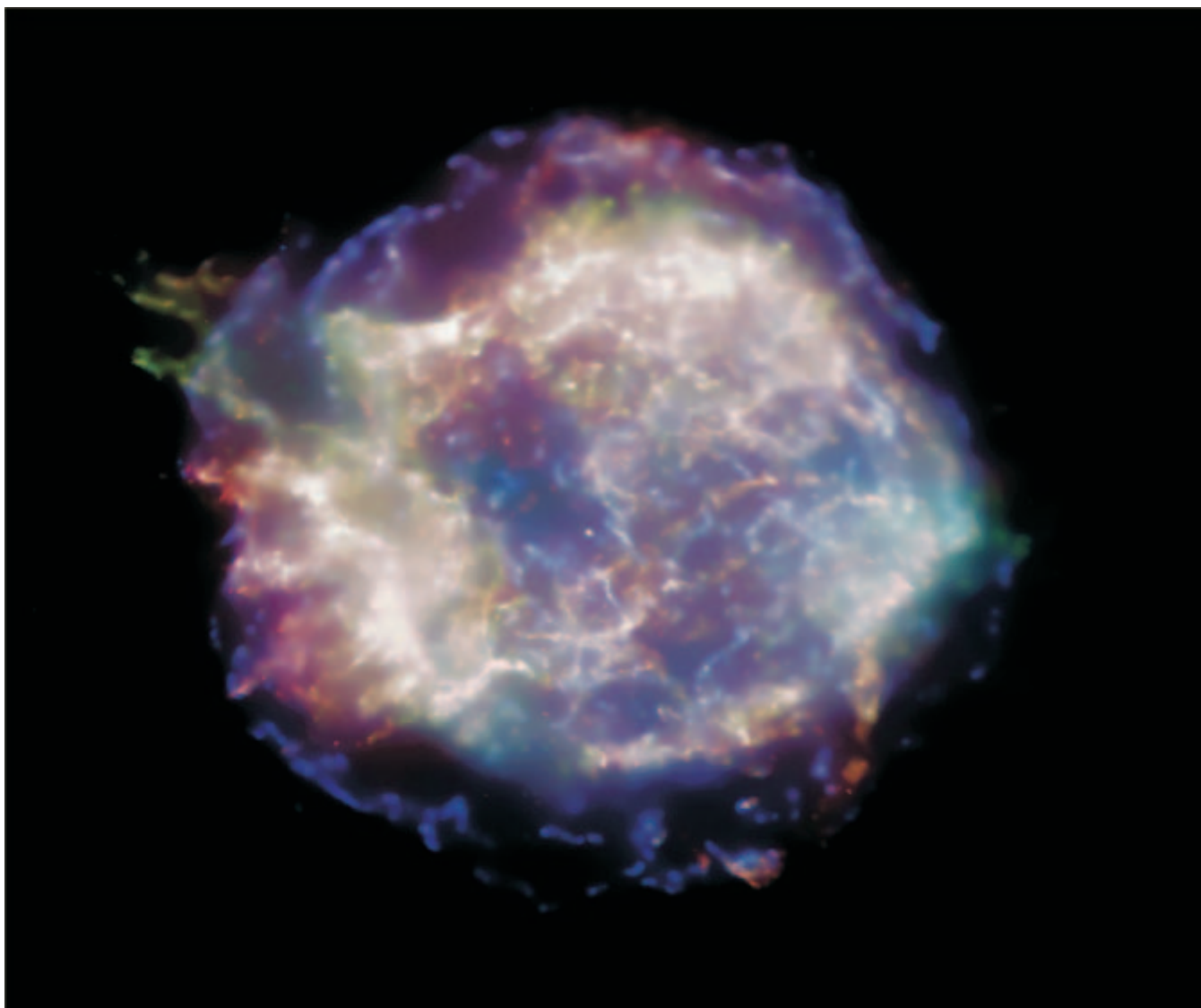
This image of the Cas A supernova remnant shows remarkable structure in the debris of a gigantic stellar explosion, as well as an enigmatic source in the center, which could be a rapidly spinning neutron star or black hole. The low, medium, and higher X-ray energies of the Chandra X-ray Observatory data are shown as red, green, and blue, respectively.
