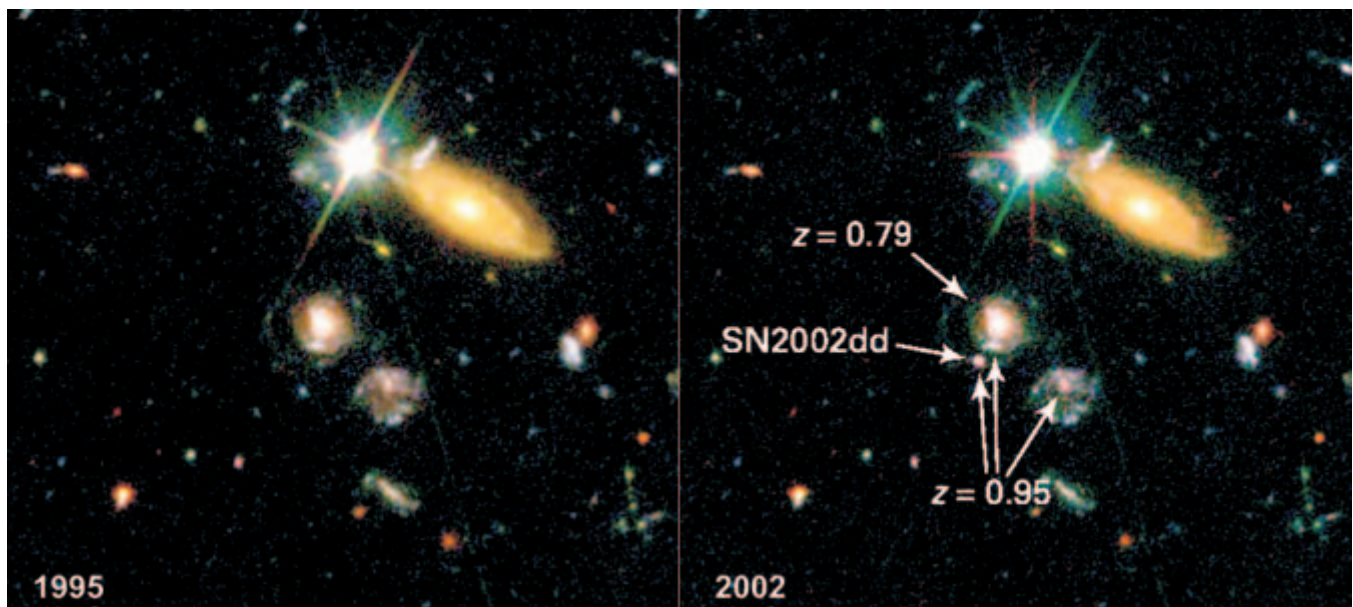
[Left] - A Hubble Space Telescope image of a portion of the Hubble Deep Field North as originally photographed in 1995 with the Wide Field and Planetary Camera 2 (WFPC2). [Right] - A composite image of the same field as imaged by Hubble's Advanced Camera for Surveys (ACS), combined with the original WFPC2 image. The ACS observations were made in May and June 2002. The red spot is the glow of a very distant supernova captured exploding in the field. The supernova is estimated to be eight billion light-years away. The supernova appears deep red in this composite image because it was photographed by the ACS at far-red wavelengths. Distant supernovae are used by astronomers to fill in the blank region where the universe's rate of expansion switched from deceleration due to gravity to acceleration due to the repulsive force of "Dark Energy."
