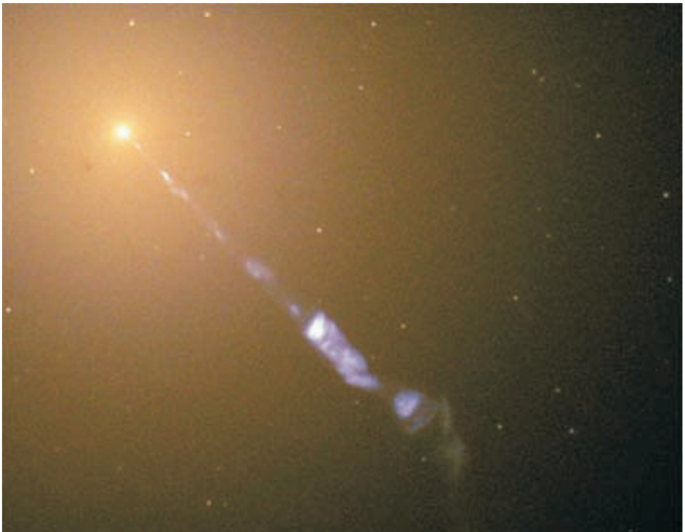
Seen in this Hubble telescope image is a black-hole-powered jet of electrons and other sub-atomic particles traveling at nearly the speed of light. The monstrous black hole at the center of galaxy M87 has swallowed up matter equal to two billion times our Sun's mass.
