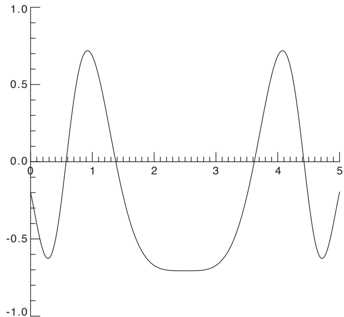
Fig. 2 — Basebanded signal from Fig. 1. This is the real part of the modulated signal removed from the 11.5-kHz carrier signal as calculated by Eq. (3). This chirp signal sweeps from -1 to +1 kHz. The \sqrt{2} amplitude reduction is a normalization factor in Eq. (3).
