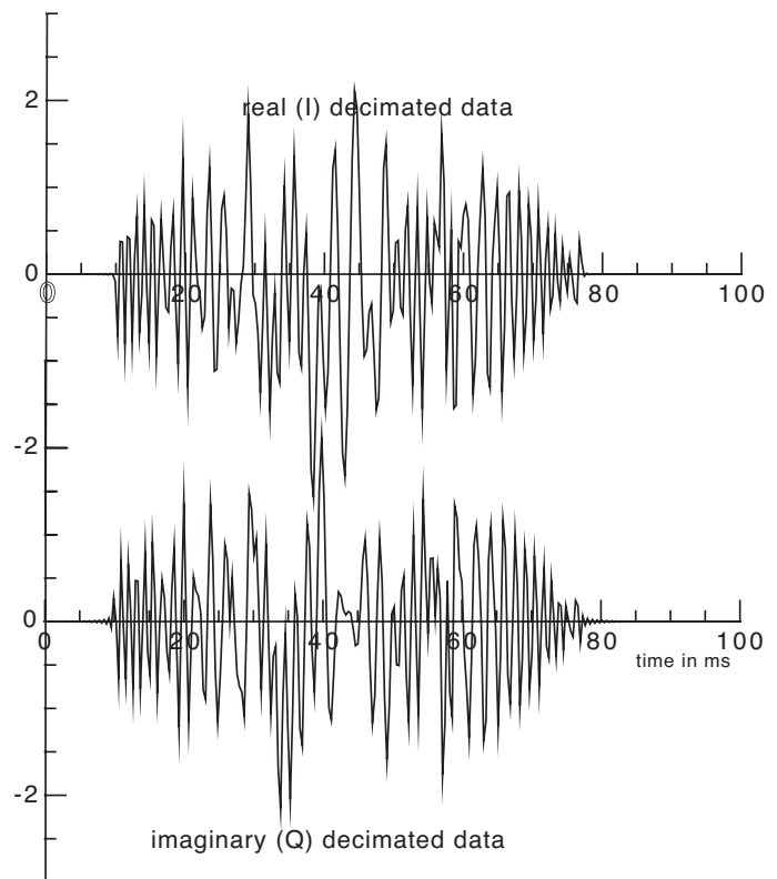
Fig. 6 — The real ( I or “in phase”) and the imaginary ( Q or “quadrature”) part of the quadrature decimated, basebanded data from Fig. 5. This data has been decimated by a factor of 16 so that there are 288 samples in each of the two time series rather than the 4,600 samples in the original 100-ms long real time series.
