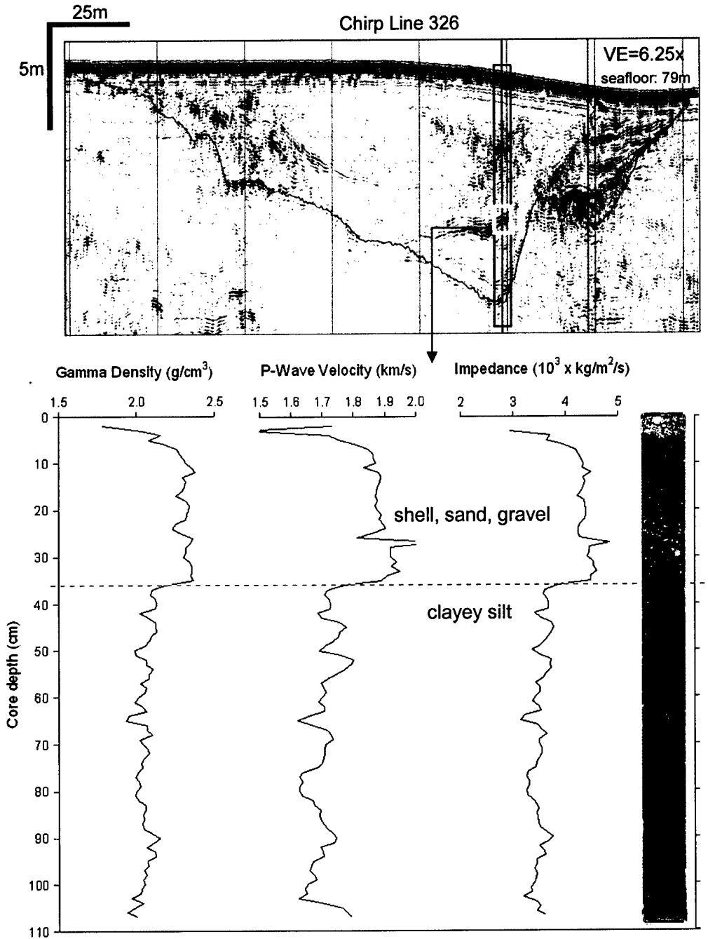
Figure 1. Example of correlated seismic and sediment physical properties data for Geoclutter drillcore Site 2. (Top) Chirp profile showing a buried channel with internal seismic reflectors of variable amplitude. The 13-m section cored during cruise KN-168 is shown (black rectangle). (Bottom) Downcore physical properties and photograph for the core section corresponding to a prominent seismic discontinuity near the channel base (white rectangle). The discontinuity is created by a contrast in acoustic impedance (density x velocity) across a stratal surface formed by the contact of shell-gravel-sand (high impedance) and clayey silt (low impedance). Seismic profile courtesy of UTIG.
