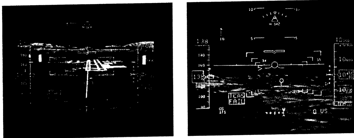
Figure 3. NASA Synthetic Vision Head-Up Display
