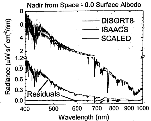
Figure 8. Results for DISORT Spectral Scaling of ISAACS Radiances with a Black Surface (Albedo = 0).
