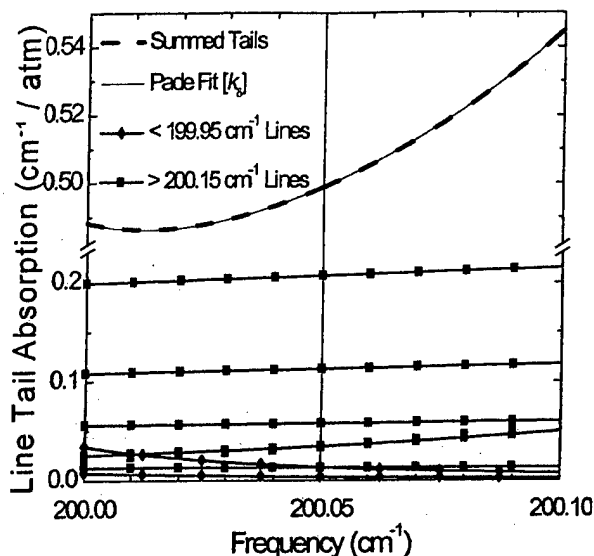
Figure 3. High Spectral Resolution Line Tail Absorption Curve (thick dash) and Padé Approximant Fit (thin line) for Lorentzian \text{H}_2\text{O} Lines at 305K and 1atm Pressure. The spectral curves from largest contributors are also illustrated (lines with diamond for lower frequency transitions and lines with squares for higher frequency transitions).
