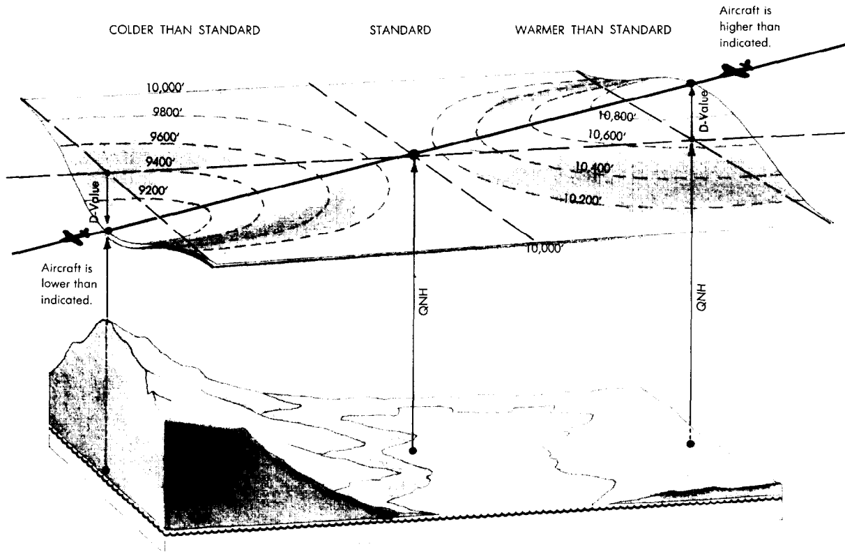
Figure 4-18. Altitude Error Due to Nonstandard Temperatures Aloft (D-Value).
