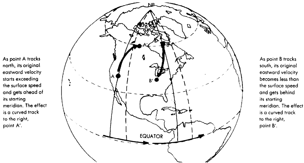
Figure 5-3. Coriolis Force.
