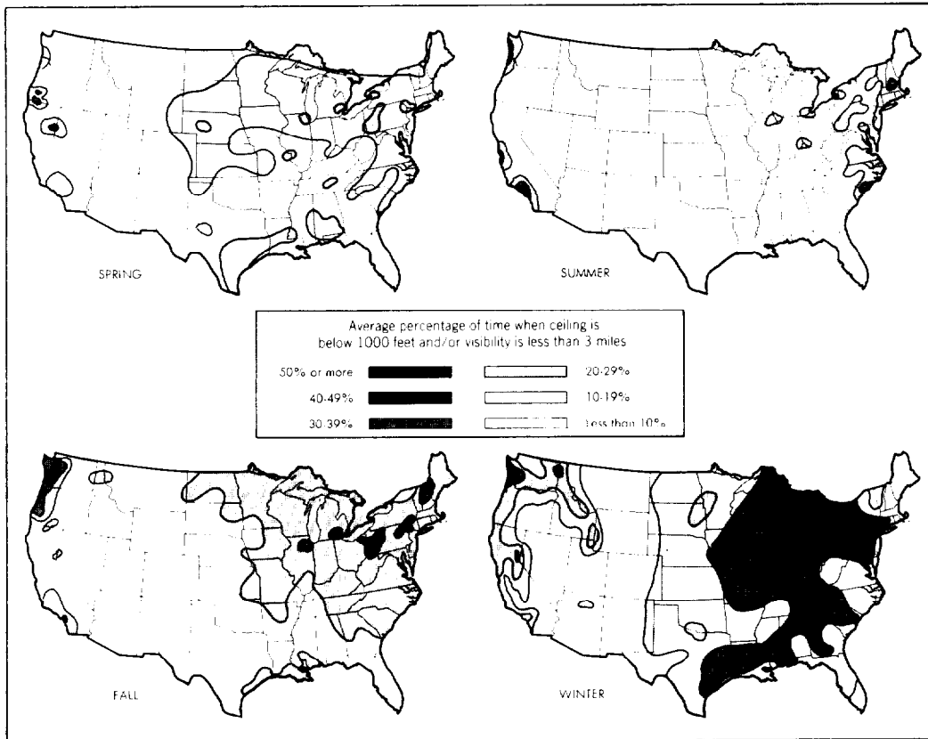
Figure 12-7. Seasonal Restrictions to Visibility.
