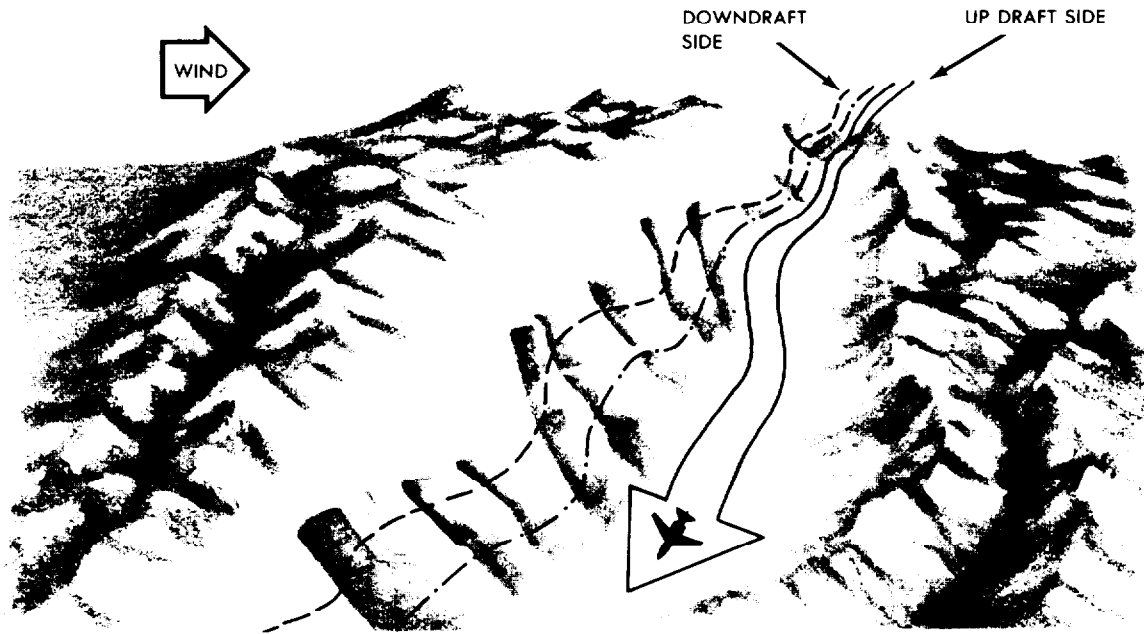
Figure 9-8. In a Valley or Canyon, Safest Path is on Upslope Wind Side.
