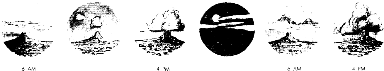
Figure 7-3. Heating Moist Air from Below.
