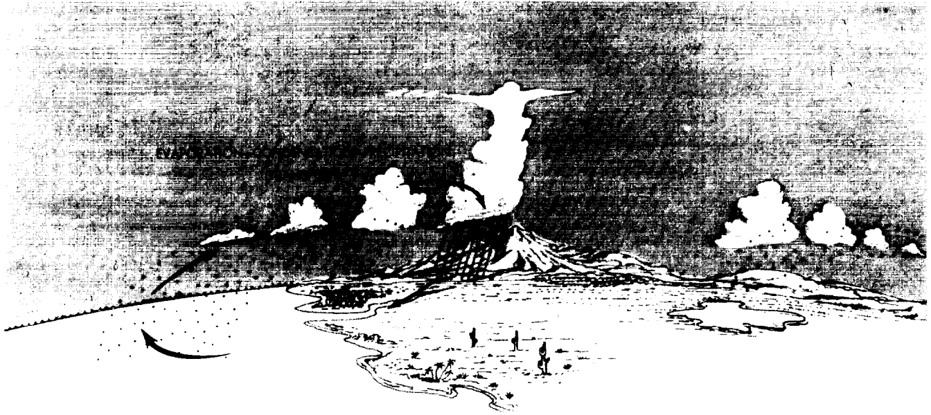
Figure 2-1. Hydrologic Cycle.
