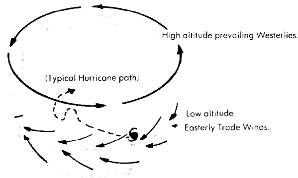
Figure 14-11. Hurricane Movement in Northern Hemisphere.
