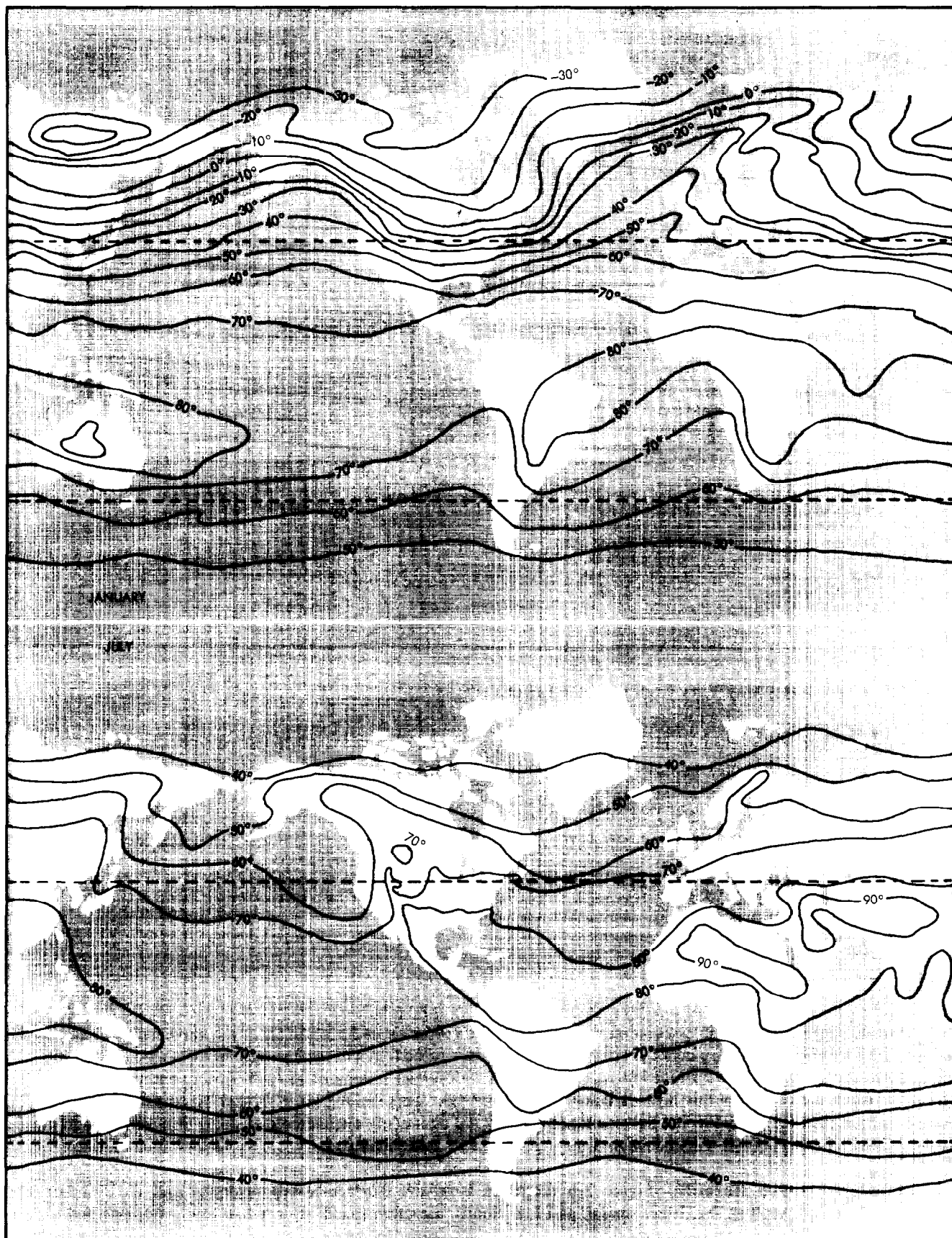
Figure 3-3. Surface Temperature Distribution.
