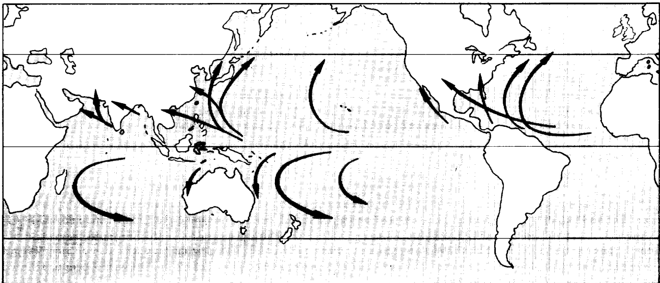
Figure 14-9. Principal Regions of Tropical Cyclone Formation and Favored Direction of Movement.
