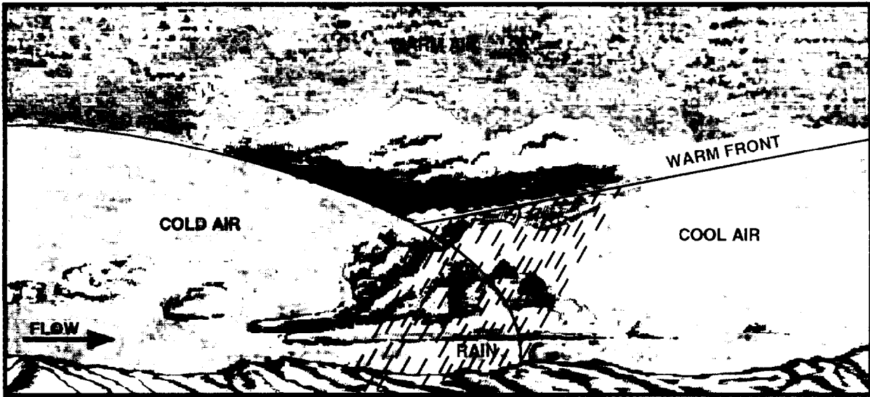
Figure 8-17. Cold Frontal Occlusion.
