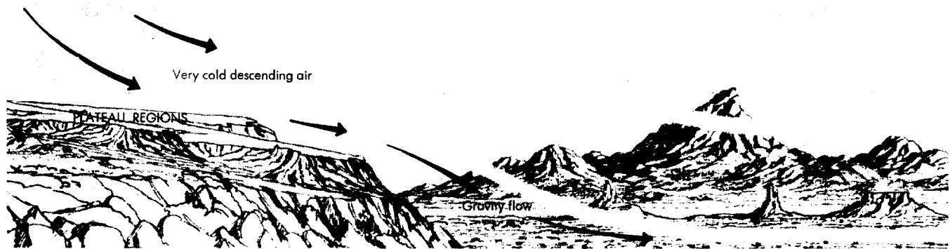
Figure 5-14. Fall Wind.
