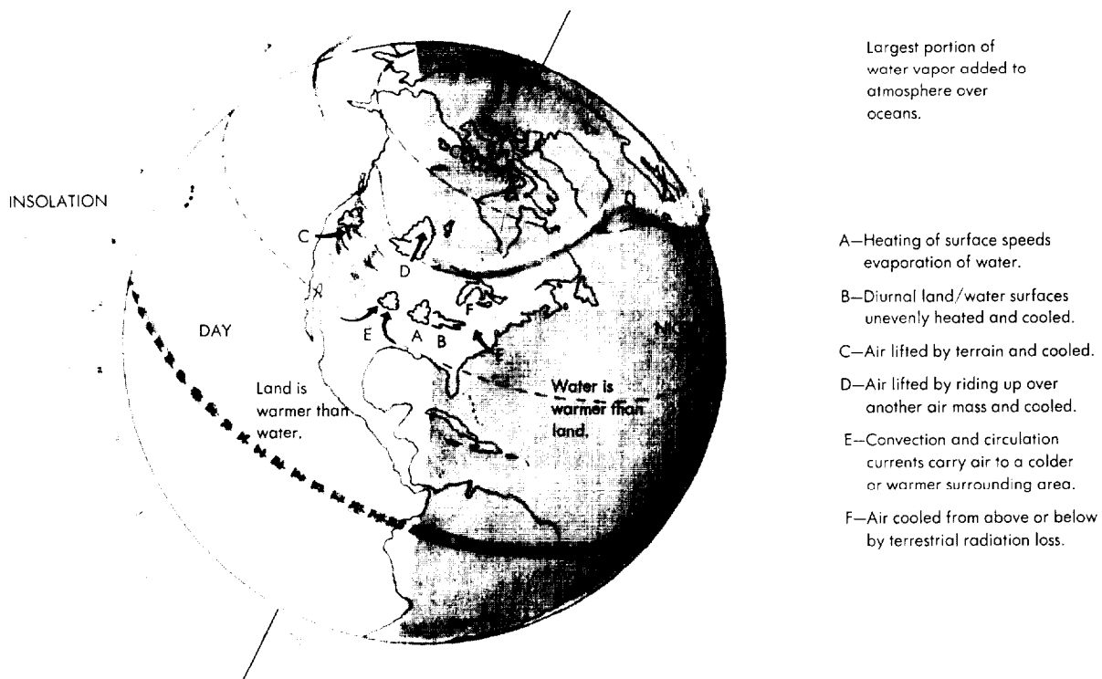
Figure 2-2. Factors Affecting Hydrologic Cycle.
