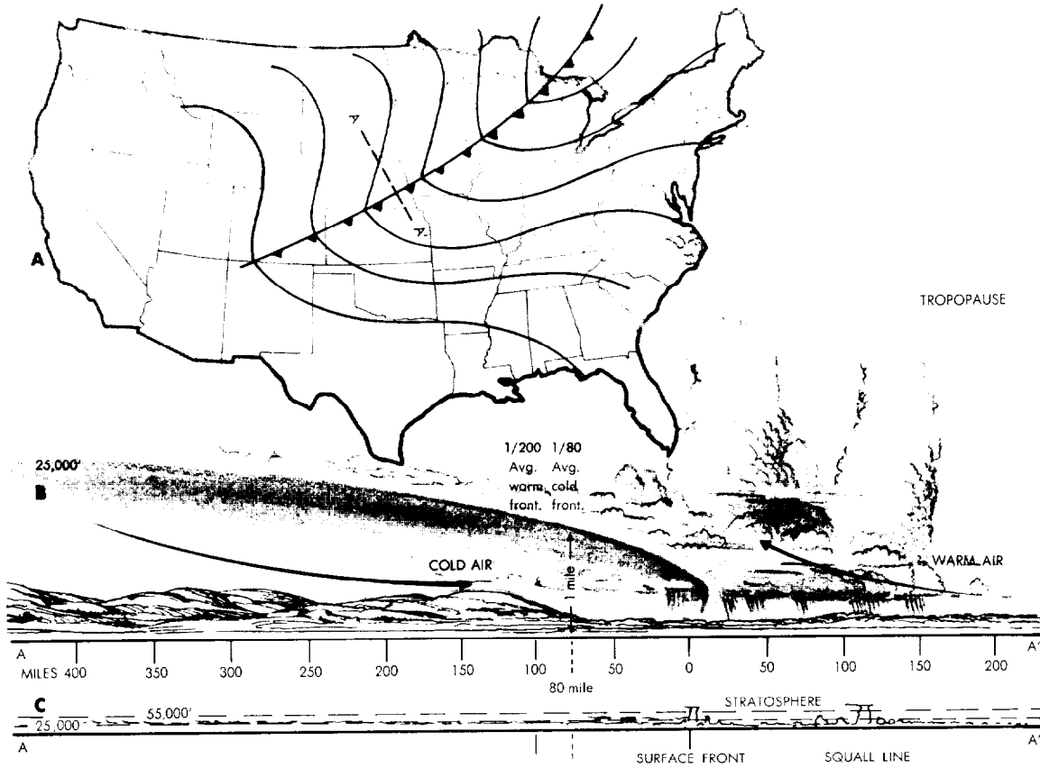
Figure 8-7. Fast Moving Cold Front and Squall Line.
