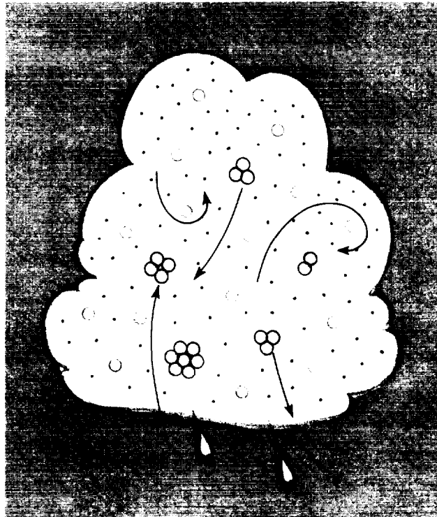
Figure 2-10. Growth of Raindrops by Collision.
