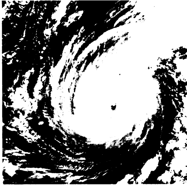
Figure 14-14. Satellite Picture of a Hurricane.
