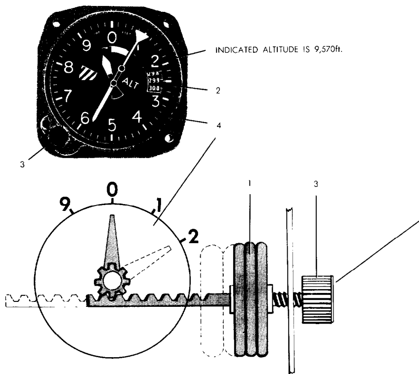
Figure 4-12. Aneroid Altimeter.
