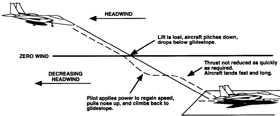
B. Performance decreasing shear where over-correction results in a long landing
