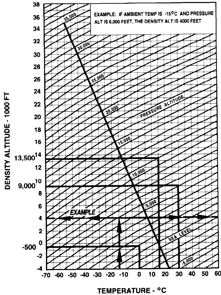
Figure 4-17. Density Altitude Chart.
