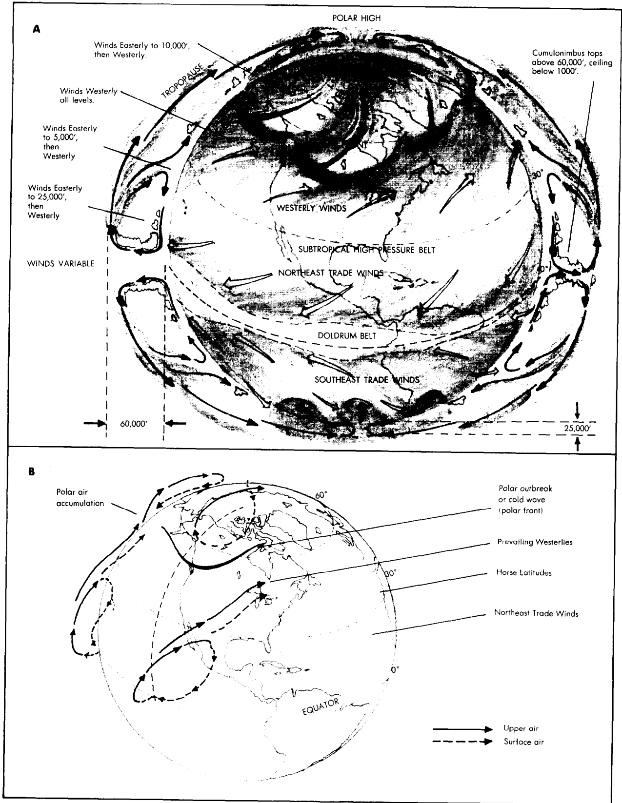
Figure 5-5. Patterns of Atmospheric Circulation.
