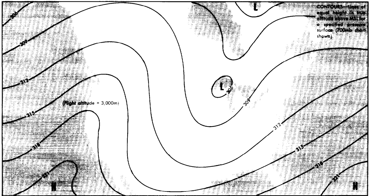
Figure 4-11. Comparison of Isobars and Contours.
