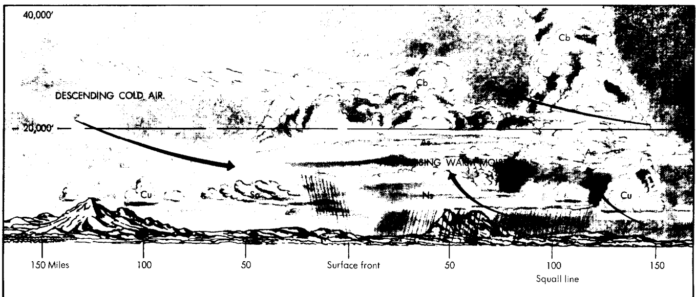
Figure 8-7. Fast Moving Cold Front and Squall Line.
