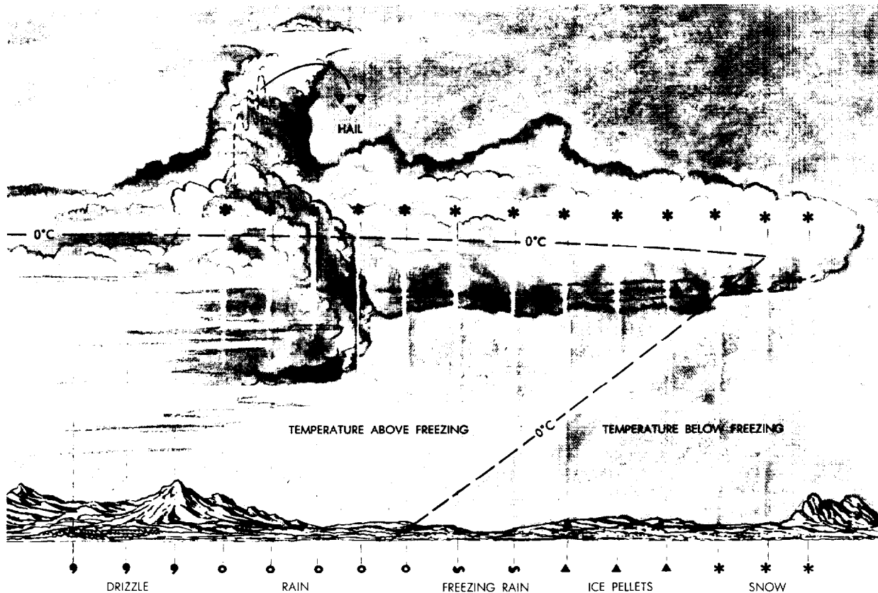
Figure 2-9. Precipitation Products.
