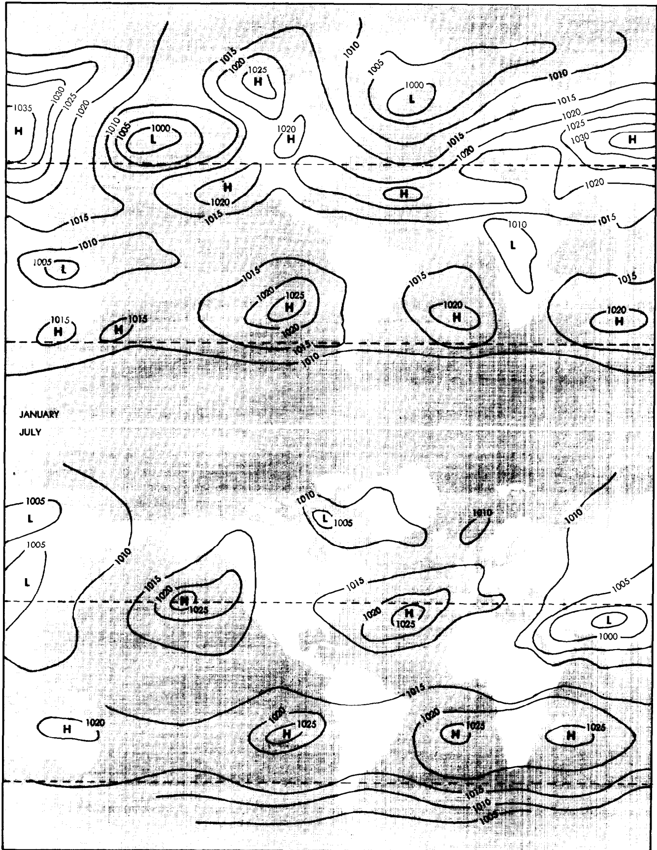
Figure 5-2. Worldwide Surface Pressure Distribution.
