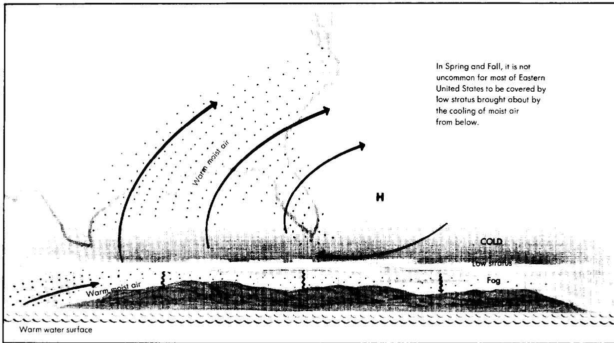
Figure 7-8. Arctic Inversion Stable Layer.
