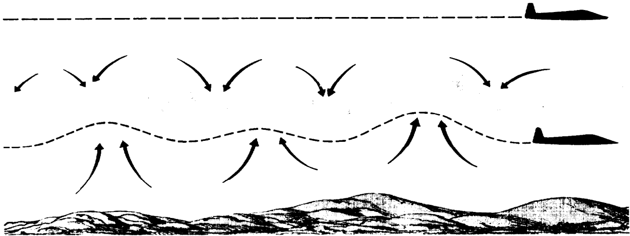
Figure 9-5. Surface Obstructions Cause Eddies and Other Irregular Wind Movements.
