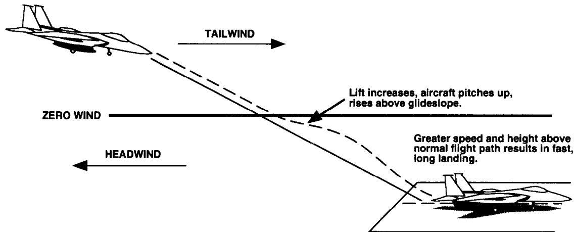
A. Performance increasing shear resulting in a long landing
