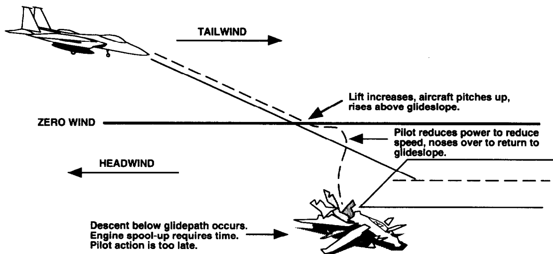
B. Performance increasing shear where over-correction results in impact short of runway
