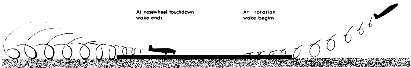
Figure 9-26. Vortex Circulation.
