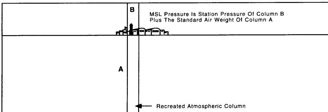
Figure 4-6. Mean Sea Level Pressure (MSL).
