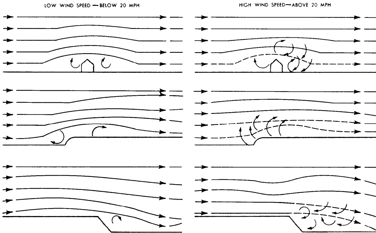
Figure 9-5. Surface Obstructions Cause Eddies and Other Irregular Wind Movements.
