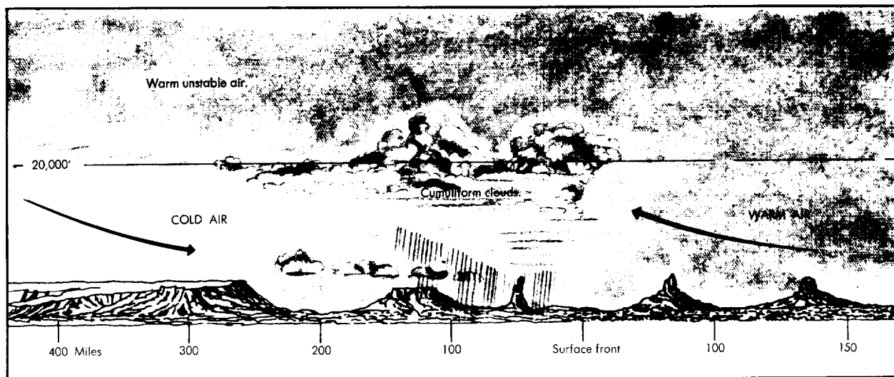
Figure 8-9. Slow Moving Cold Front and Unstable Air.
