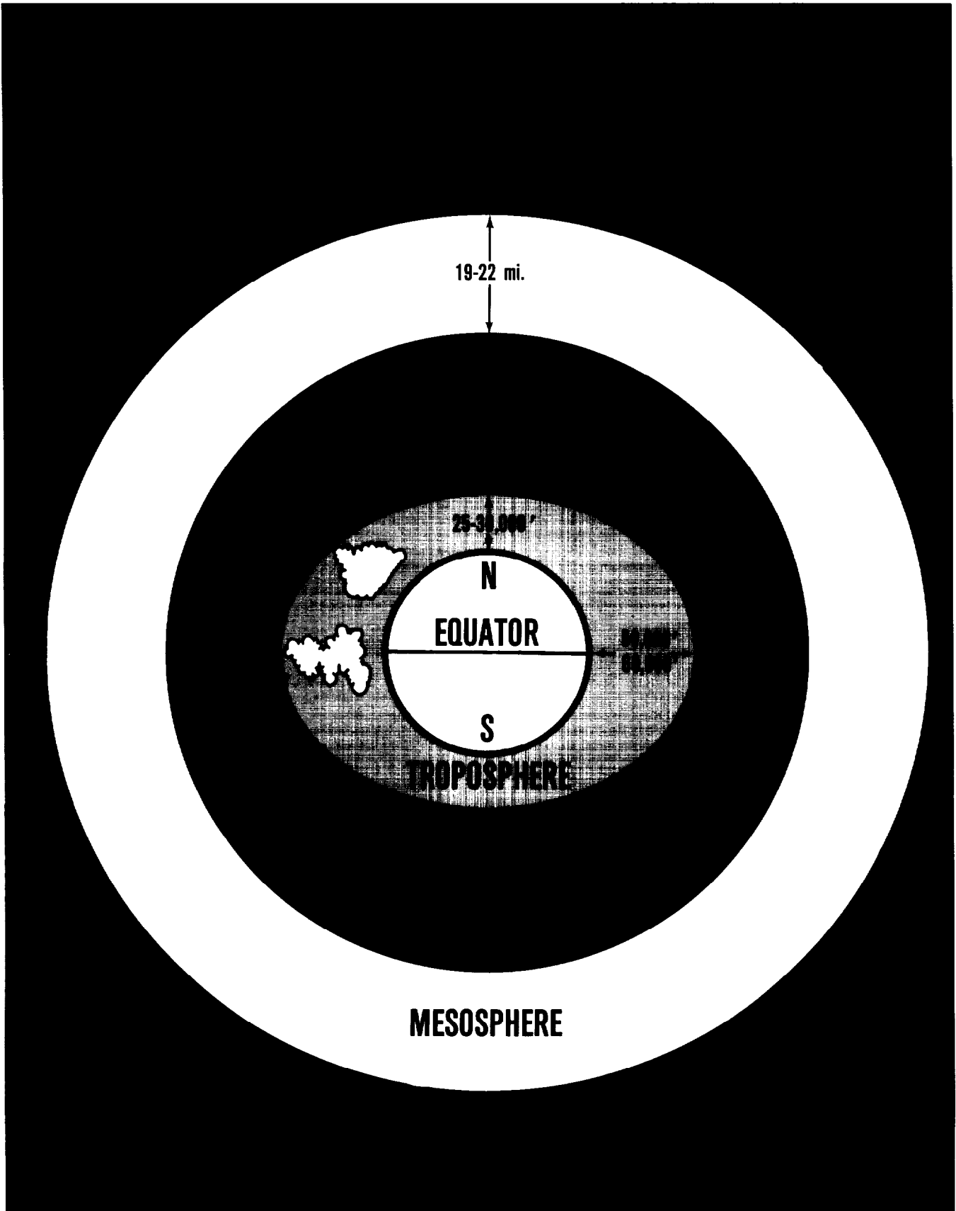
Figure 1-3. Atmospheric Layers.
