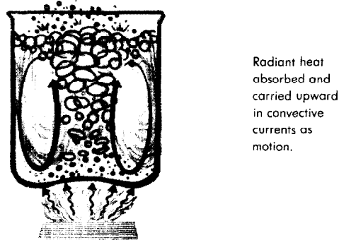
Figure 7-2. Heating from Below Causes Instability.
