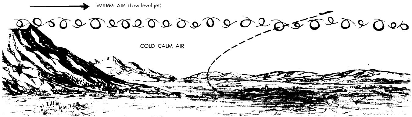
Figure 5-15. Horizontal Wind Shear Turbulence.
