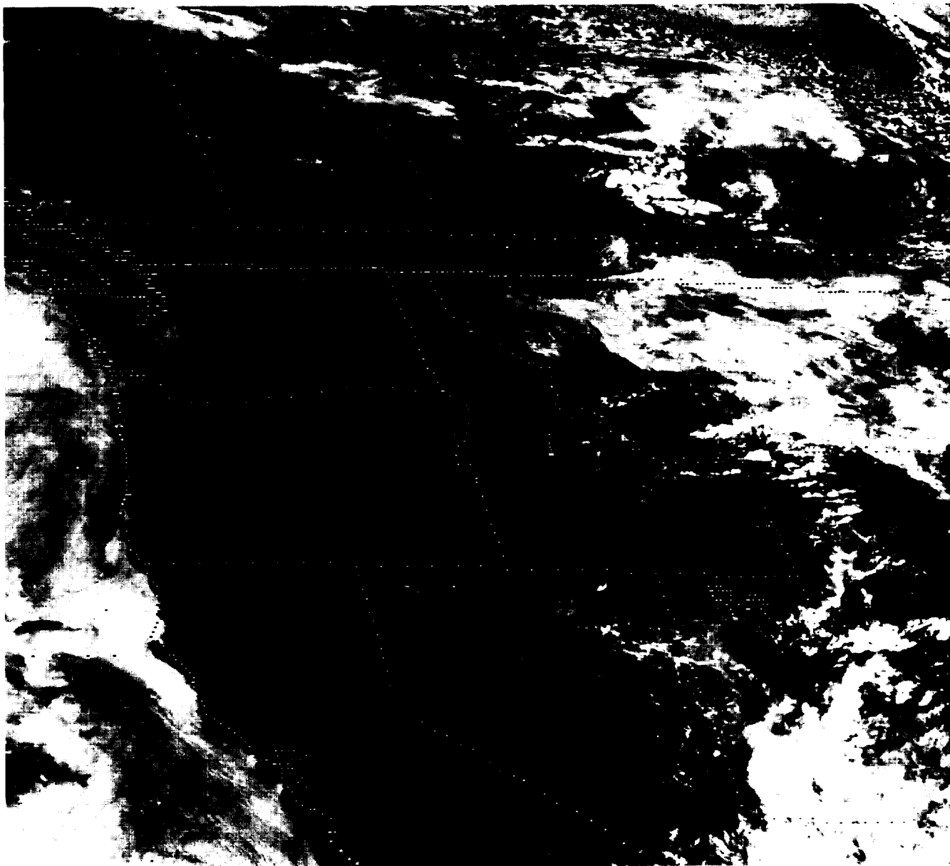
Figure 12-11. Precipitation-Induced Fog.
