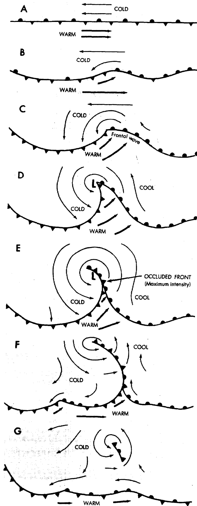
Figure 8-16. Frontal Wave and Occlusion.
