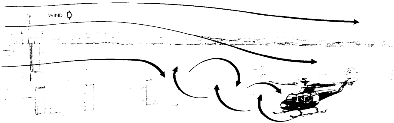
Figure 9-6. Buildings Near Landing Area May Cause Turbulence.
