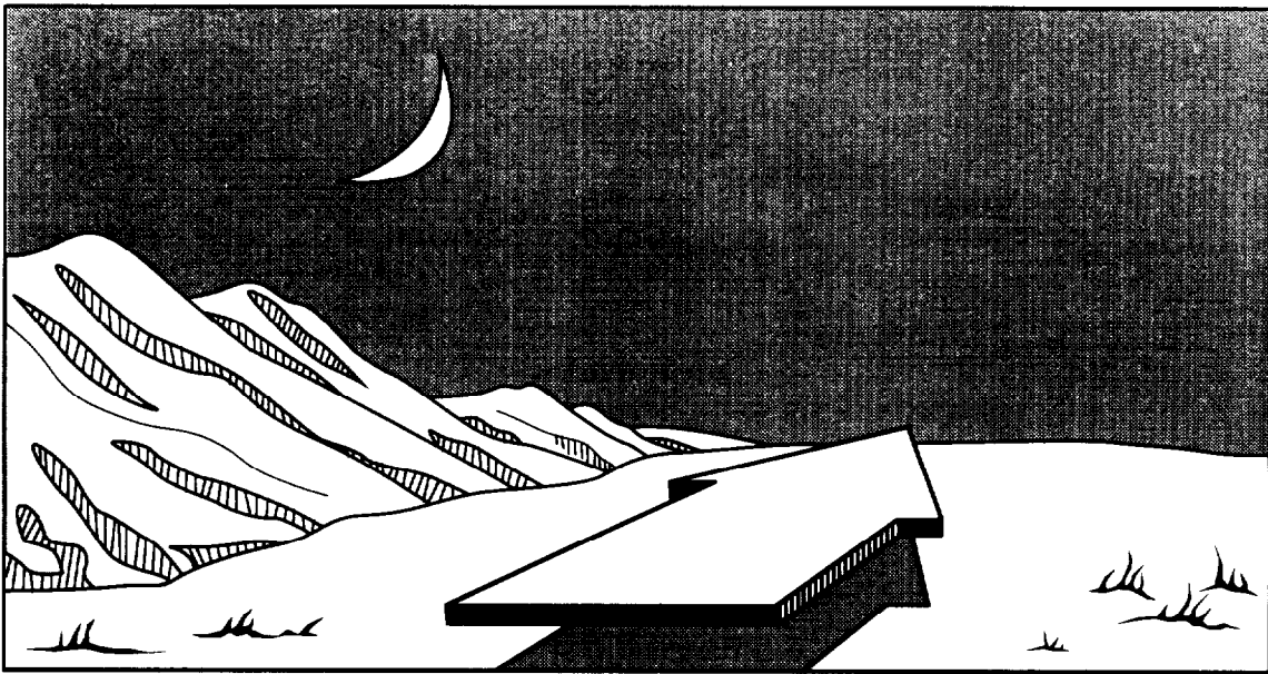
Figure 9-11. The Low Level Nocturnal Jet Stream.
