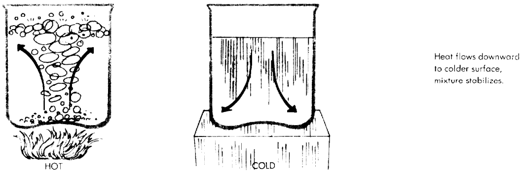
Figure 7-5. Cooling from Below Improves Stability.
