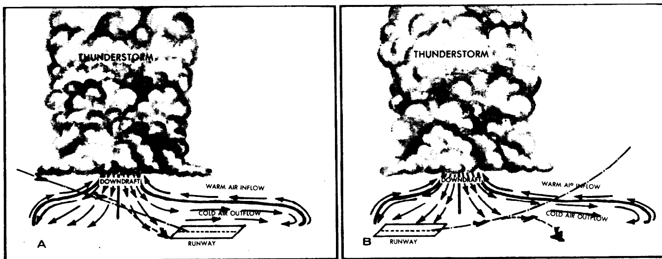
Figure 13-31. Thunderstorm Wind Shear Hazard Zones.
