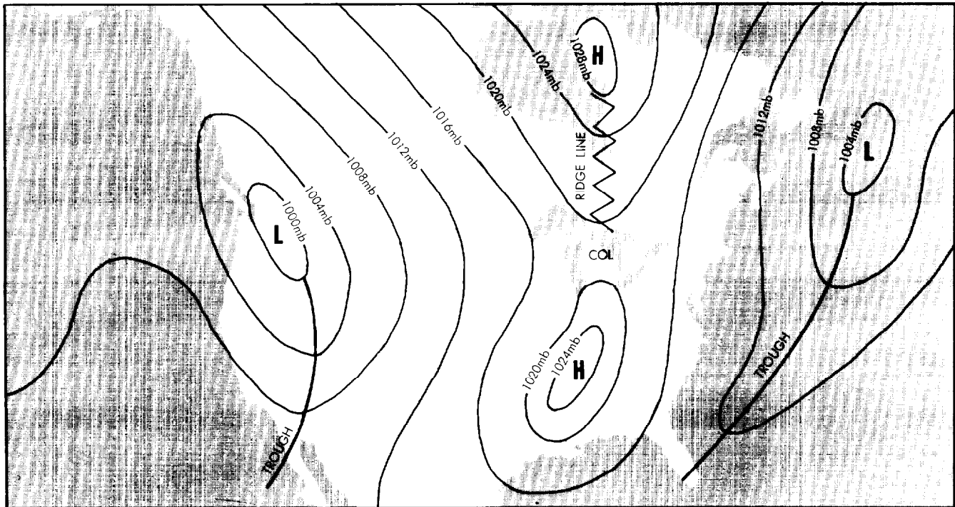
Figure 4-9. Surface Pressure Chart.
