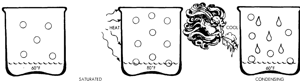
Figure 2-5. Saturation of Air Depends on its Temperature.
