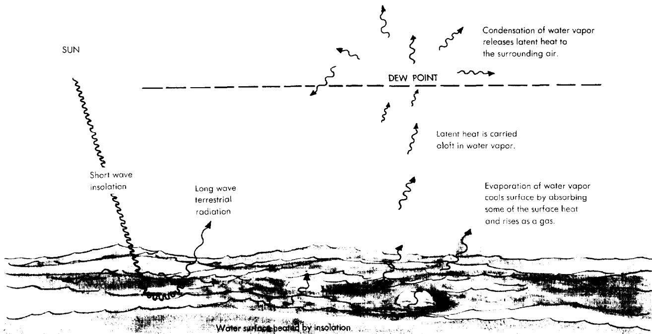
Figure 2-4. Evaporation and Condensation.
