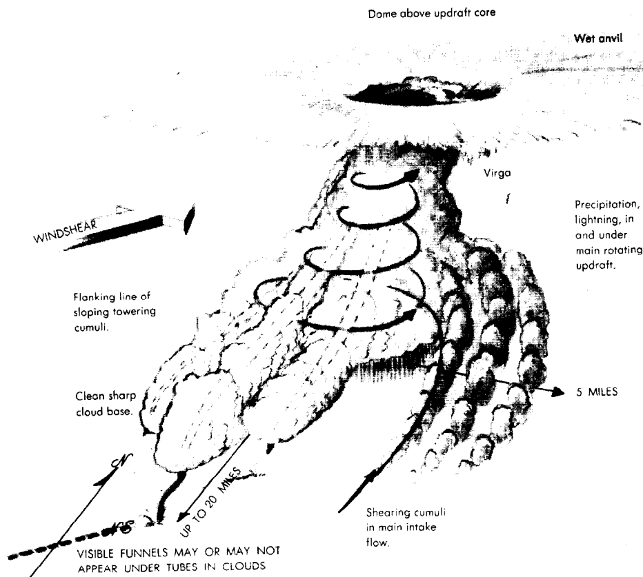
Figure 13-29. Anatomy of a Funnel Cloud.
