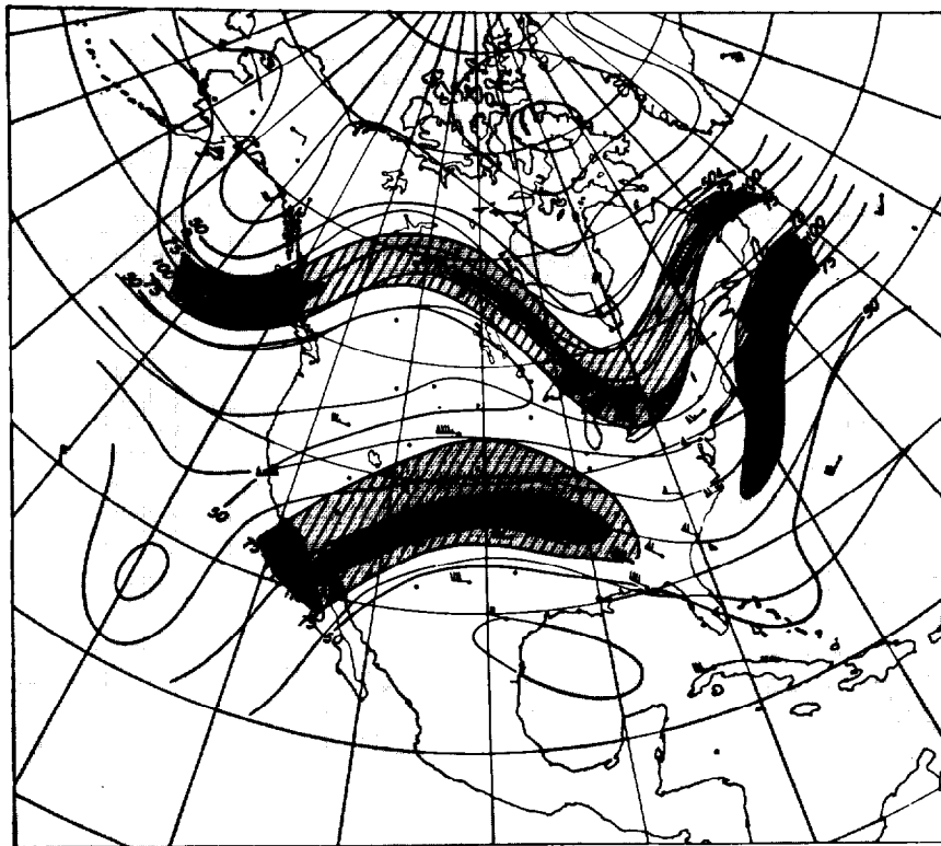
Figure 9-20. Examples of Multiple Structure of Jet Stream.
