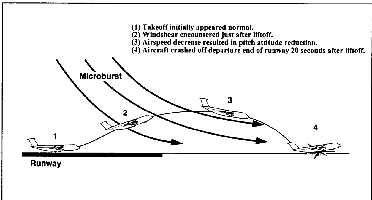
Figure 10-9. Windshear Encounter During Takeoff After Liftoff.
