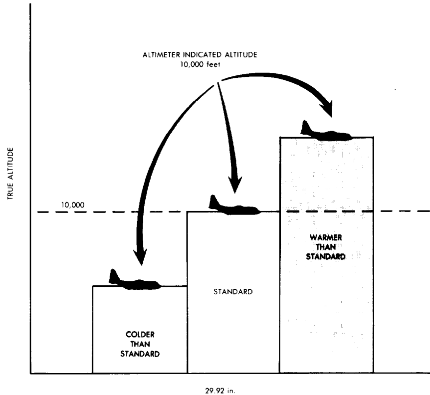
Figure 4-13. Effects of Temperature on True and Indicated Altitude.
