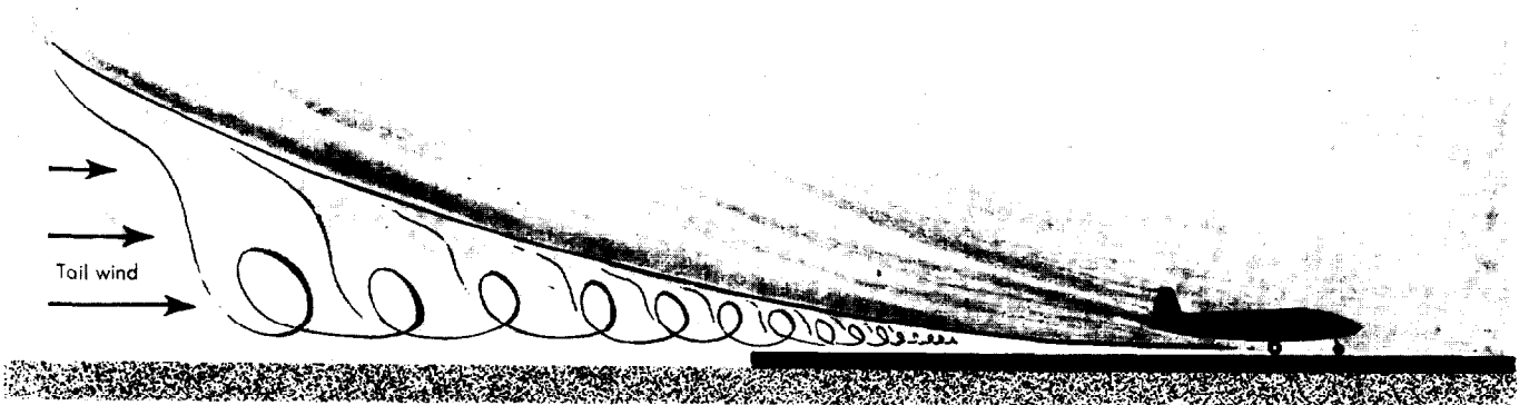
Figure 9-31. Helicopter Vortices.
