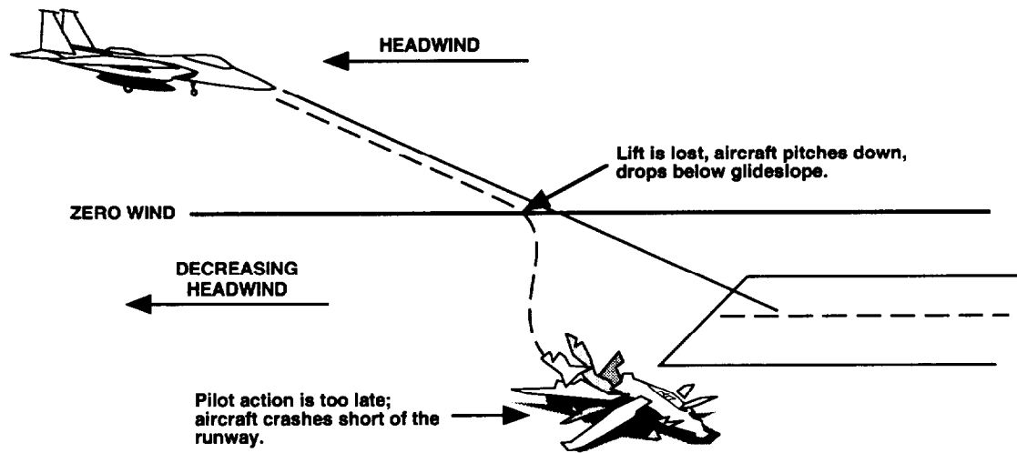
Figure 10-1. Performance Decreasing Shear.
