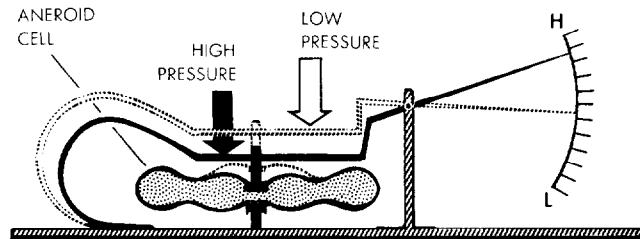
Figure 4-3. Aneroid Barometer Inner View.
