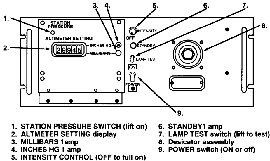
Figure 4-2. Digital Barometer Altimeter Setting Indicator (DBASI).
