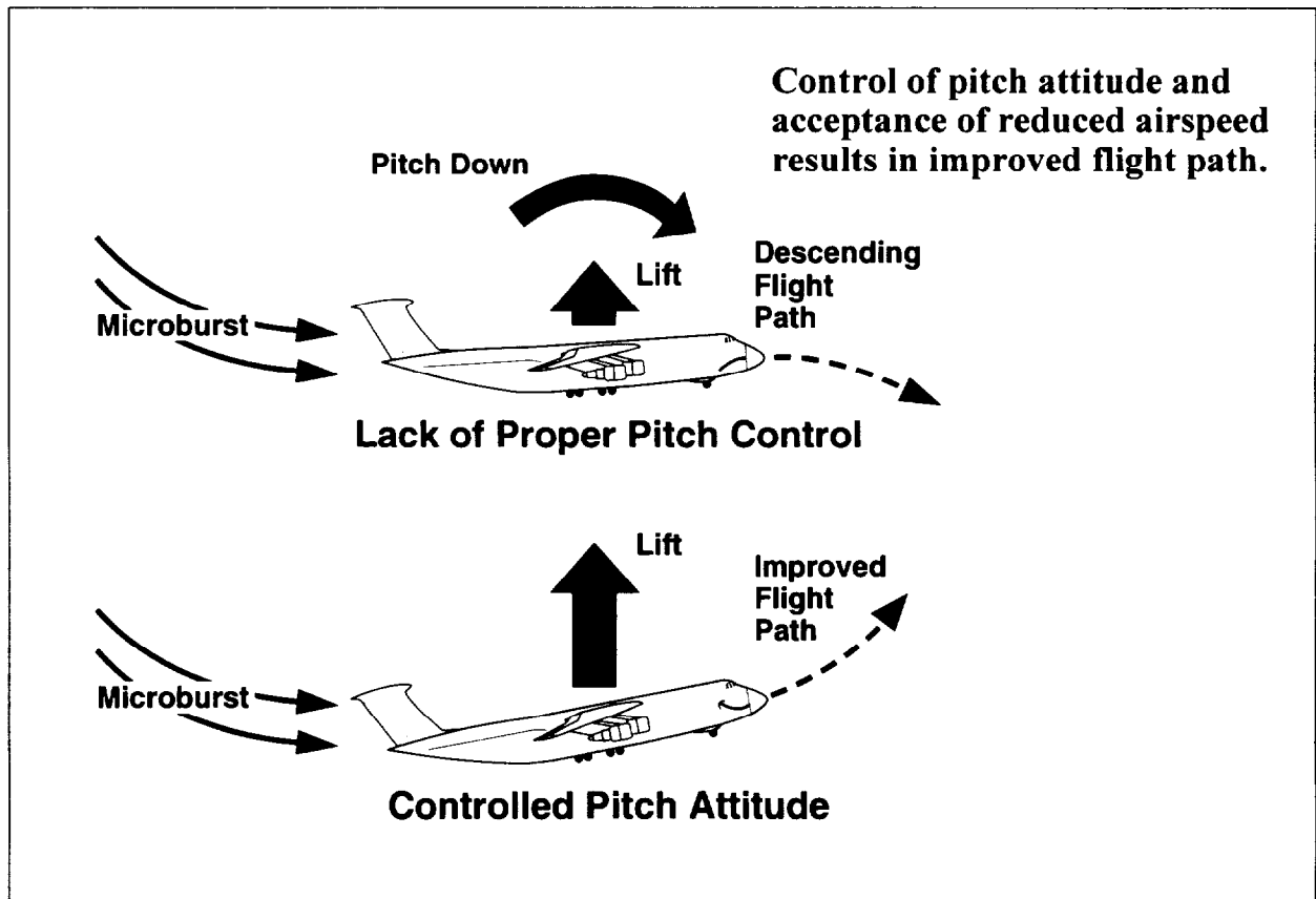
Figure 10-11. Pitch Controls on Flight Path.
