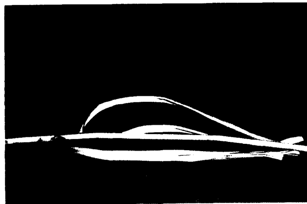
Figure 13-23. FB-111 Pitot Tubes after being Struck by Lightning.
