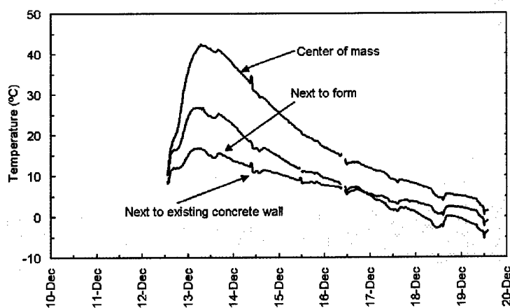
Figure 51. Concrete temperatures.
