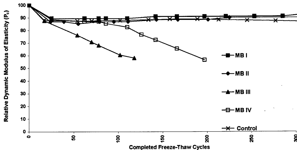
Figure 13. Relative dynamic modulus of elasticity using the Master Builders admixtures. Each line represents the average values from three replicate beams. (The air contents of fresh concrete were: MB I, 6.25%; MB II, 6.25%; MB III, 1.5%; MB IV, 7.5%; control, 8.5%.)
