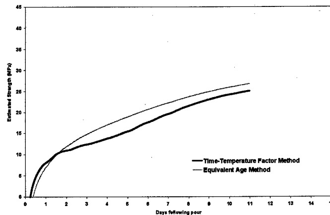
Figure D15. Strength-maturity relationships used to estimate in-place concrete strength development for Concord, NH, field site.
