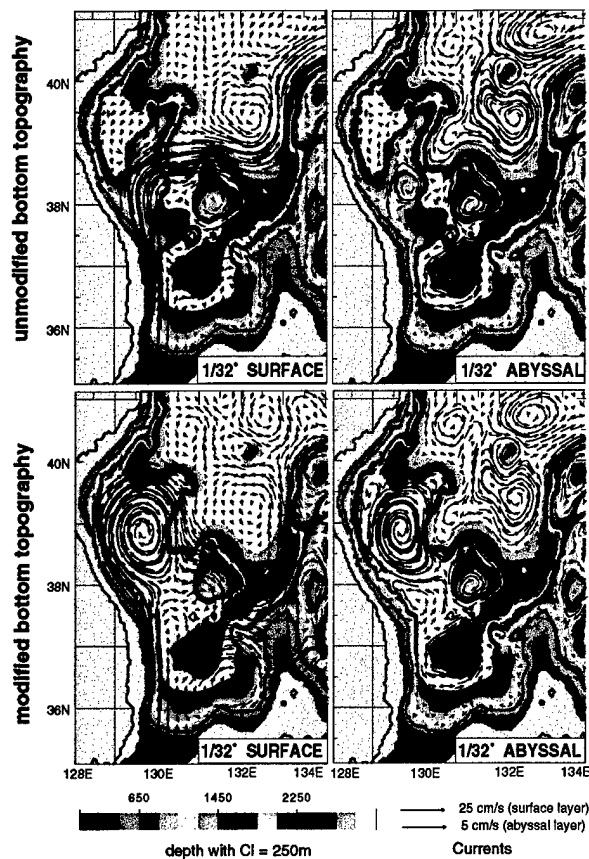
Figure 3. Bottom topography (color) and mean currents from 1/32^\circ simulations of the Japan/East Sea using the NRL Layered Ocean Model in the region where the East Korea Warm Current (EKWC) separates from the coast. Only the southern portion of the model domain is shown. Left panels show surface currents and the right panels show abyssal currents. In the bottom row, the topographic ridge near 39^\circ\text{N} , 130^\circ\text{E} has been removed. This modified the offshore abyssal flow in this region and affected the separation latitude ( 37^\circ - 38^\circ\text{N} ) of the EKWC. Adapted from Hogan and Hurlburt (2000).
