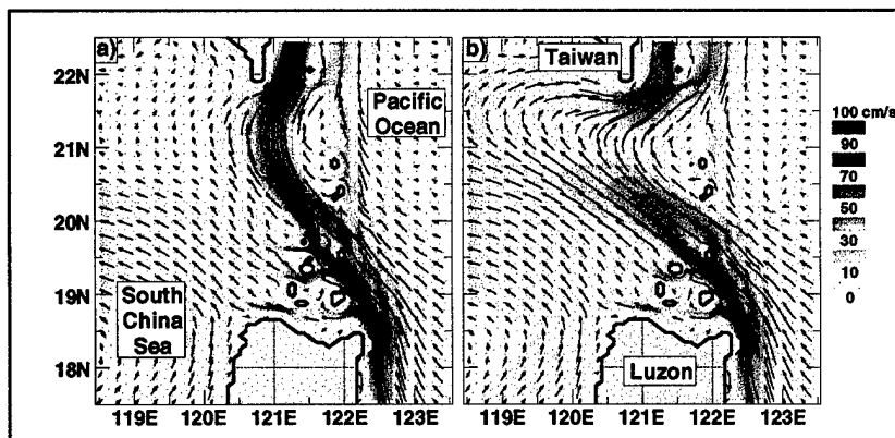
Figure 4. The 6-year mean upper layer speed and currents from 1/16^\circ Pacific NLOM simulations (zoom-in on the Luzon Strait that connects the Pacific Ocean and the South China Sea) that (a) include Calayan Bank and the shoal north of Calayan Island and (b) exclude these three model gridpoints. The specified model gridpoints are highlighted in blue on the left panel. Adapted from Metzger and Hurlburt (2001).
