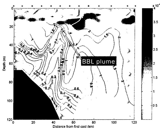
Figure 12. Spring section of N^2 (color, s^{-2} \times 10^{-4} ), with ATC overlaid (black contours, ^{\circ}C ). The tongue of low ATC, indicating the detached BBL, is indicated. The white contours denote the potential density ( kg\ m^{-3} ).
