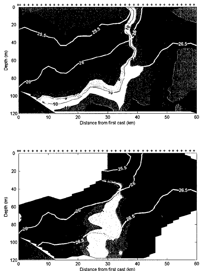
Figure 8. A spring section of (a) potential temperature and (b) accumulated temperature change from May 1996.
