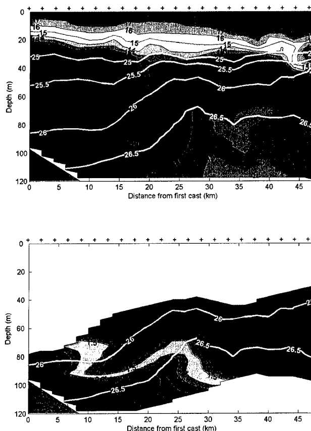
Figure 10. A summer section of (a) potential temperature and (b) accumulated temperature change from July 1996.
