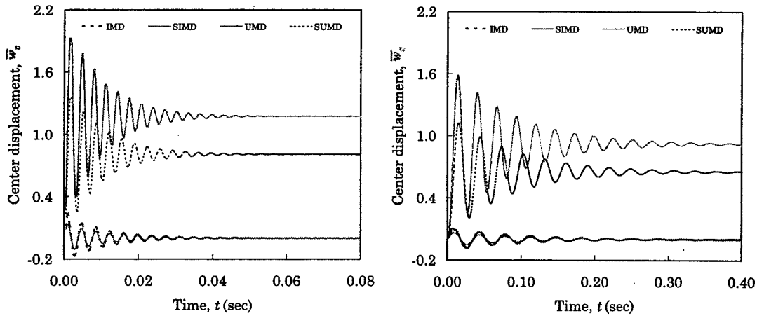
(a) Sym. cross-ply laminate ( a/h=10 )
