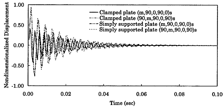
Figure 11. Nondimensionalized central displacement for simply supported and clamped laminated plates under suddenly applied uniformly distributed loading.
