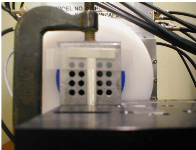
Figure 38. Source positioning for activated Sn strips to produce the AFIT “T”
