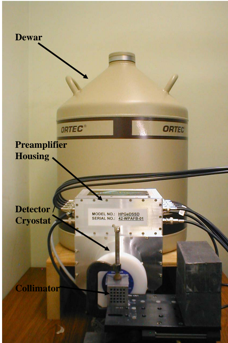
Figure 11. Photograph of the detector, dewer, and collimator
