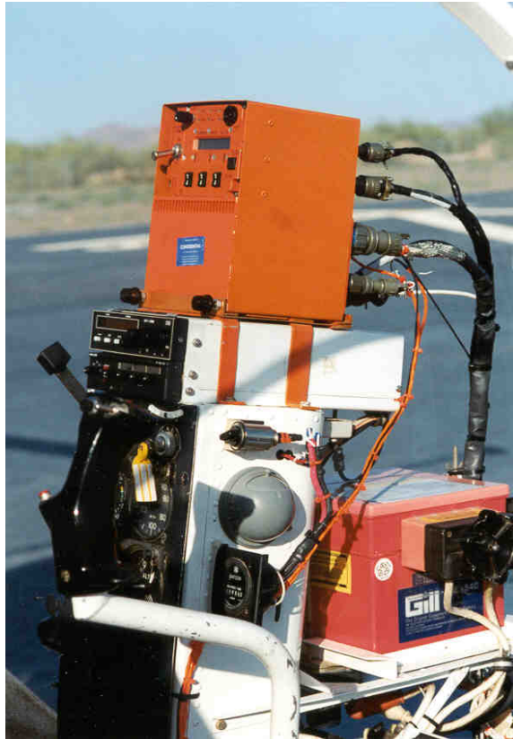
Figure 3. ASVS Control Installation
