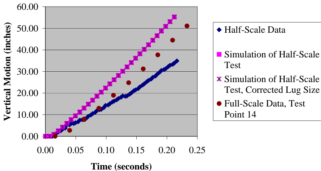
Figure 14. Effect of Lug Size on Vertical Motion, 40 Knots Full-Scale Conditions
