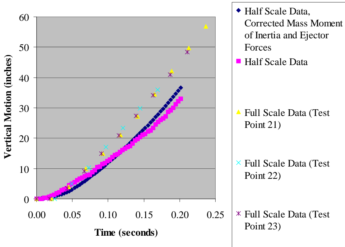
Figure I-2 Effect of Correct Mass Moment of Inertia Plus Ejector Forces on Half-Scale Vertical Motion, 100 Knots Full-Scale Conditions
