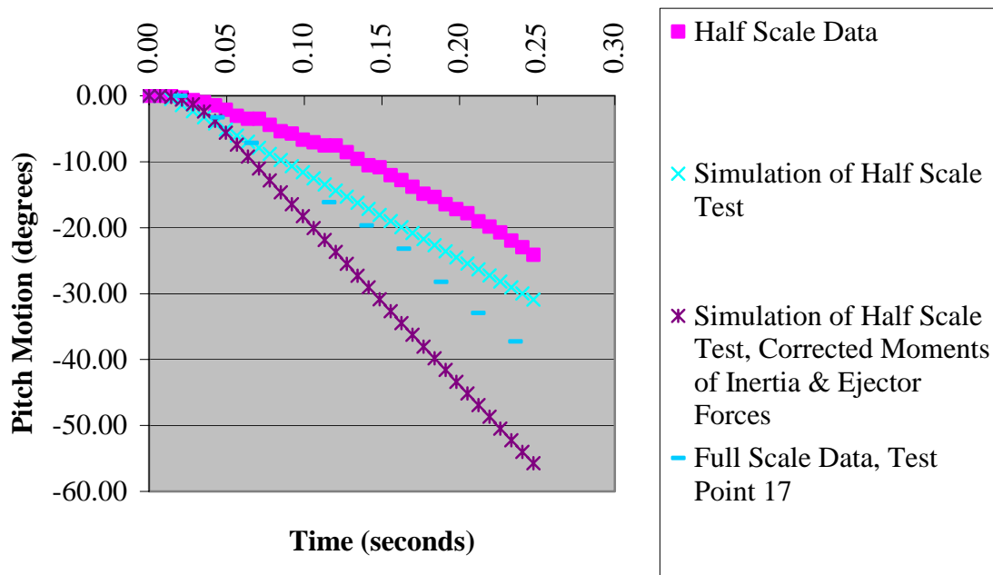
Figure H-1. Effect of Mass Moment of Inertia Plus Ejector Forces on Pitch Motion, 70 Knots Full-Scale Conditions
