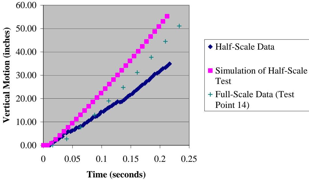
Figure 8. Simulation of Half-Scale Test, Vertical Motion, 40 Knots Full-Scale
