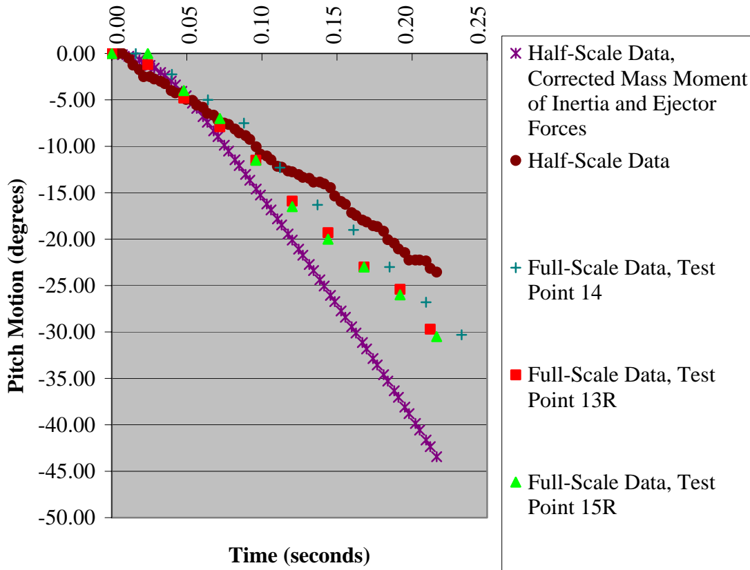
Figure 19. Effect of Ejector Forces and Mass Moment of Inertia on Half-Scale Pitch Motion Data, 40 Knots Full-Scale Conditions
