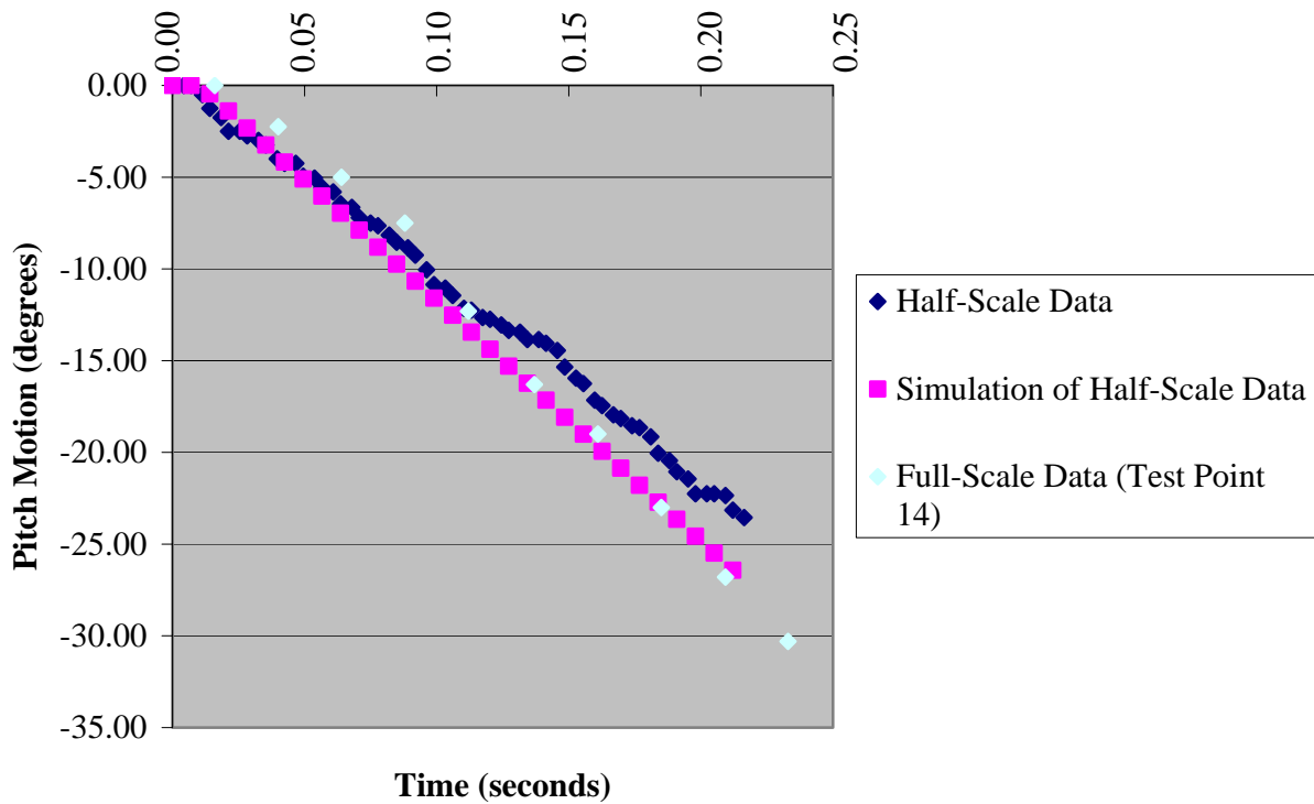
Figure 9. Simulation of Half-Scale Test, Pitch Motion, 40 Knots Full-Scale
