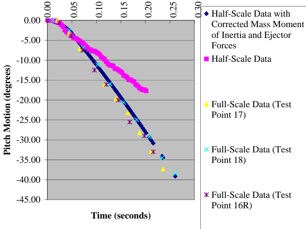
Figure 20. Effect of Ejector Forces and Mass Moment of Inertia on Half-Scale Pitch Motion Data, 70 Knots Full-Scale Conditions
