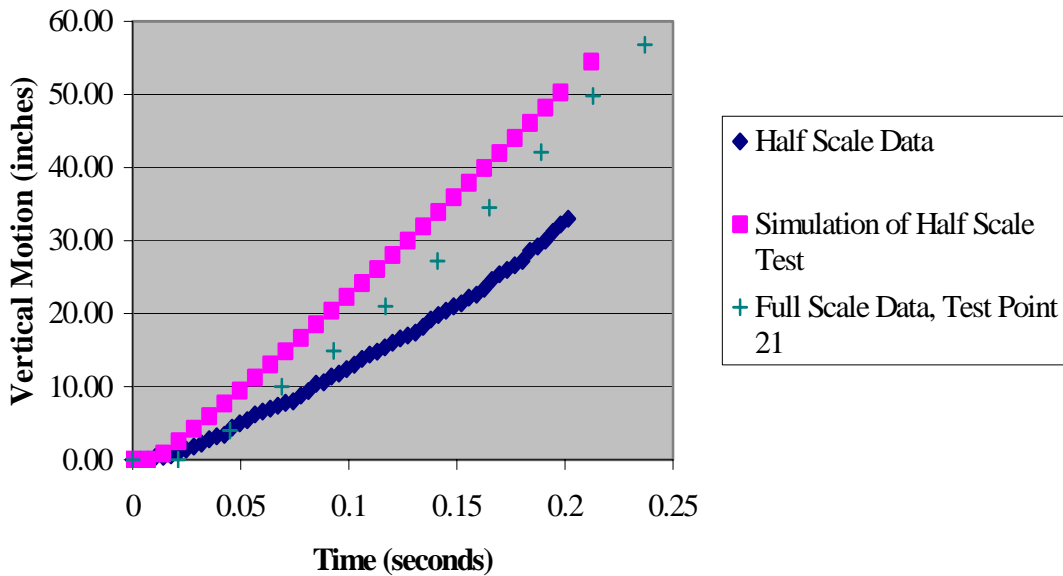
Figure G-2. Baseline Simulation Results, Vertical Motion, 100 Knots Full-Scale Conditions
