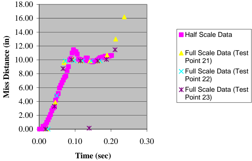
Figure E-2 Comparison of Miss-Distance Versus Time Calculation at 100 Knots Full-Scale Conditions
