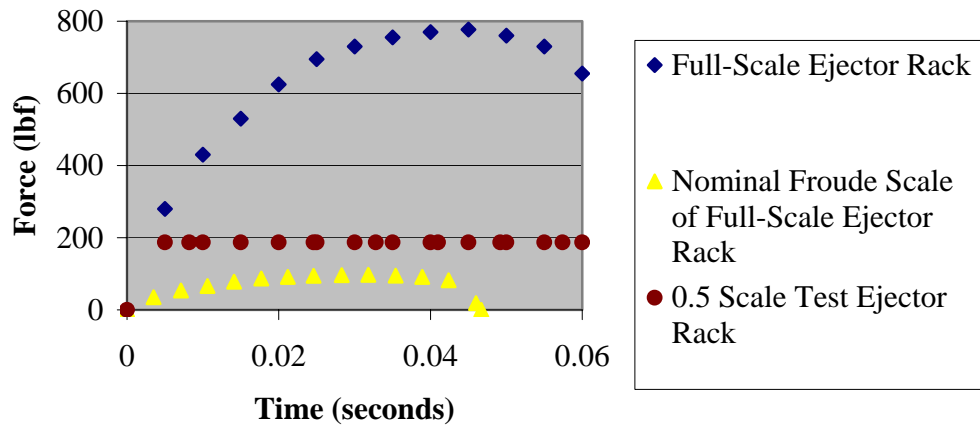
Figure 1. Comparison of Scale Ejector Force Versus Froude Nominal Values
