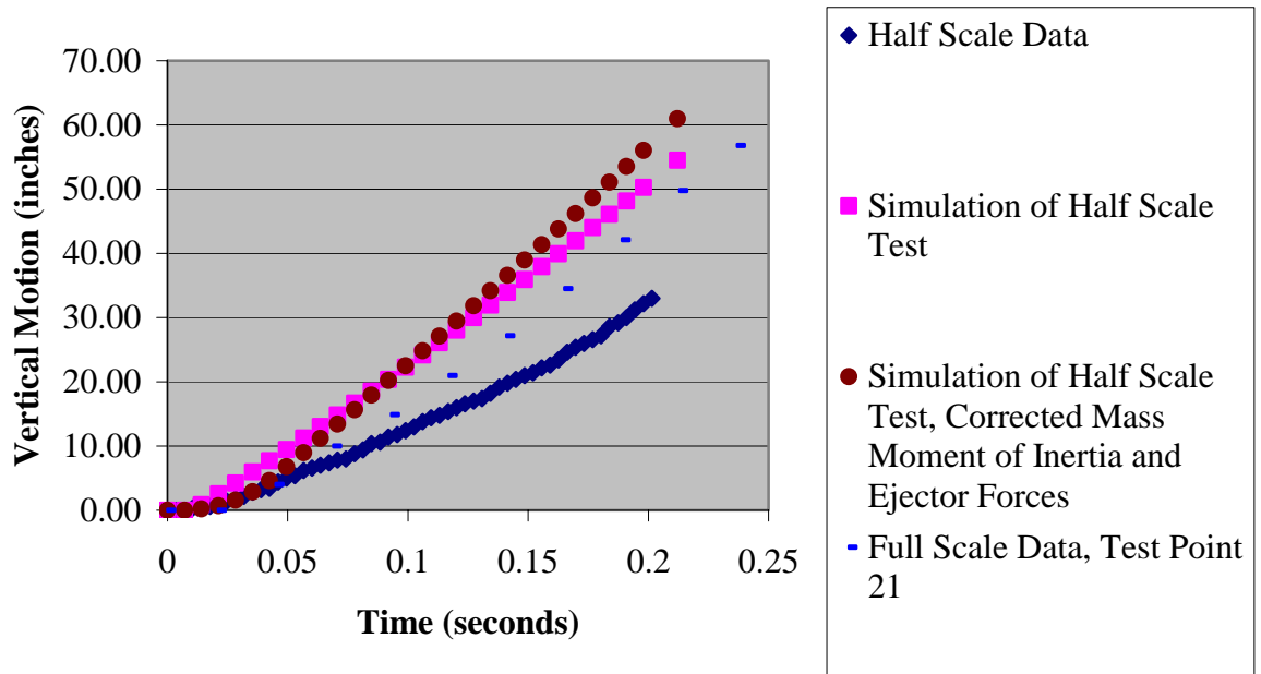
Figure H-4. Effect of Mass Moment of Inertia Plus Ejector Forces on Vertical Motion, 100 Knots Full-Scale Conditions
