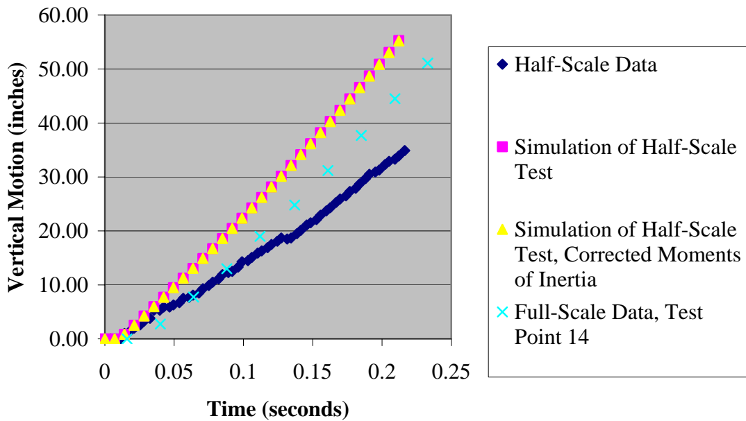
Figure 10. Effect of Mass Moment of Inertia on Vertical Motion, 40 Knots Full-Scale Conditions
