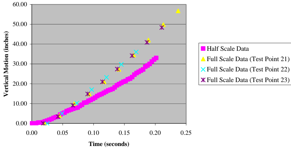
Figure C-2. Comparison of Vertical Motion at 100 Knots Full-Scale Conditions
