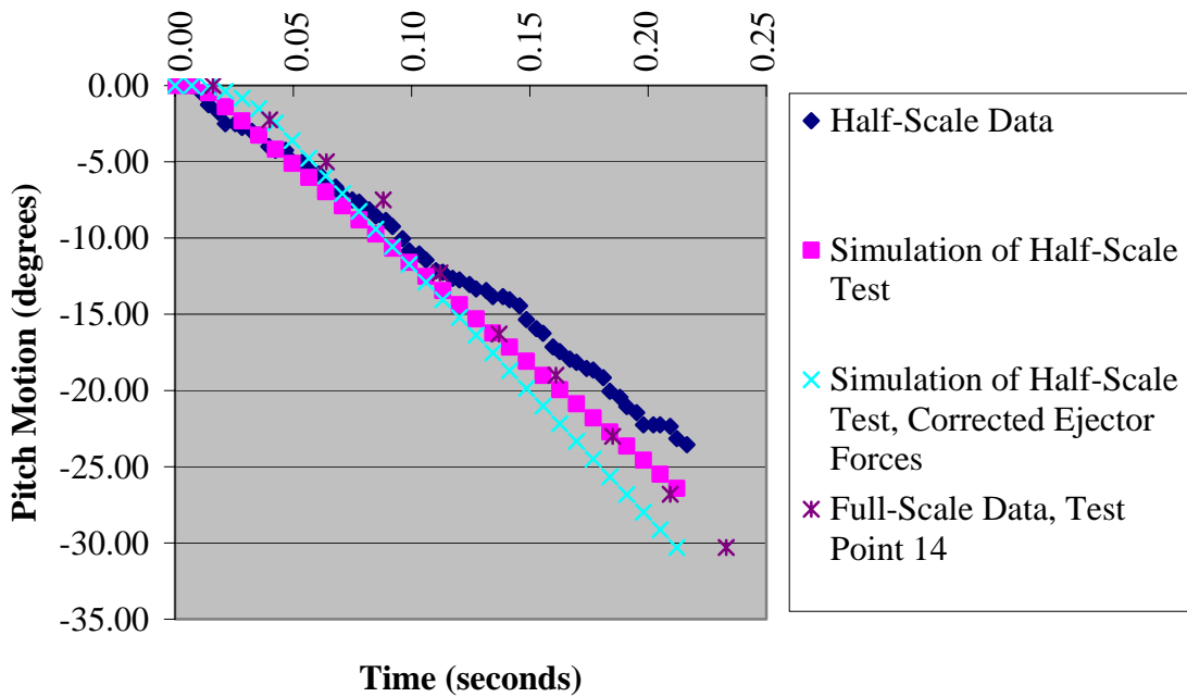
Figure 13. Effect of Ejector Force on Pitch Motion, 40 Knots Full-Scale Conditions
