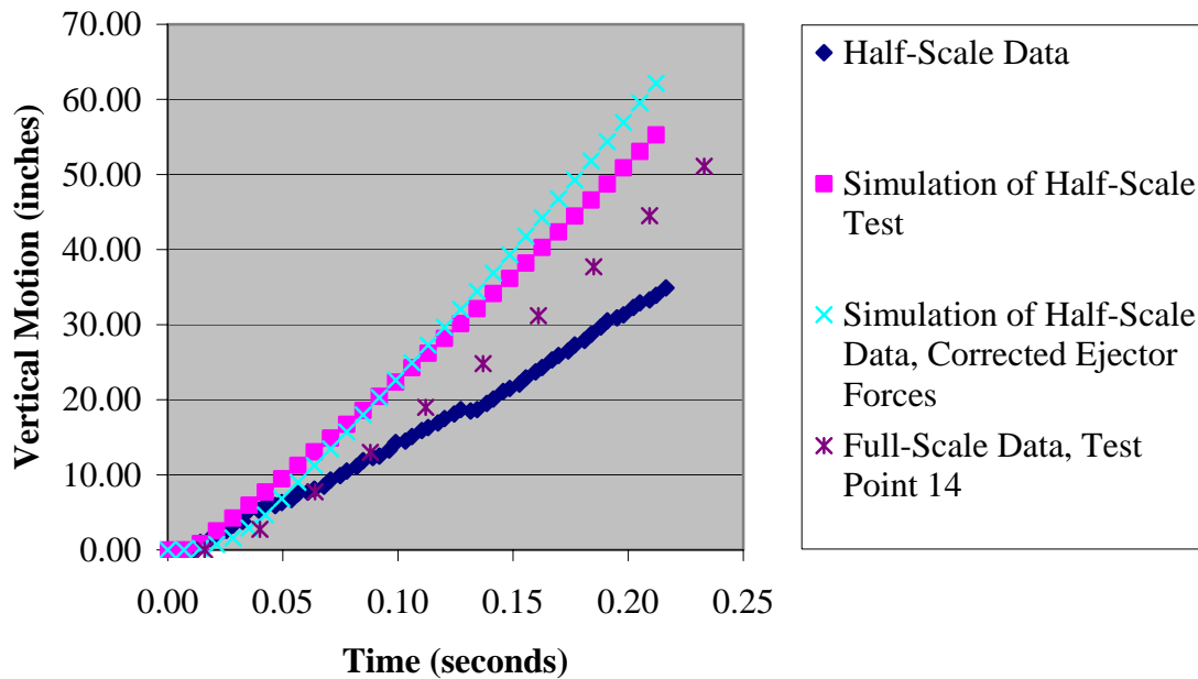
Figure 12. Effect of Ejector Force on Vertical Motion, 40 Knots Full-Scale Conditions
