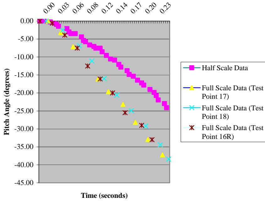
Figure D-1. Comparison of Pitch Motion at 70 Knots Full-Scale Conditions
