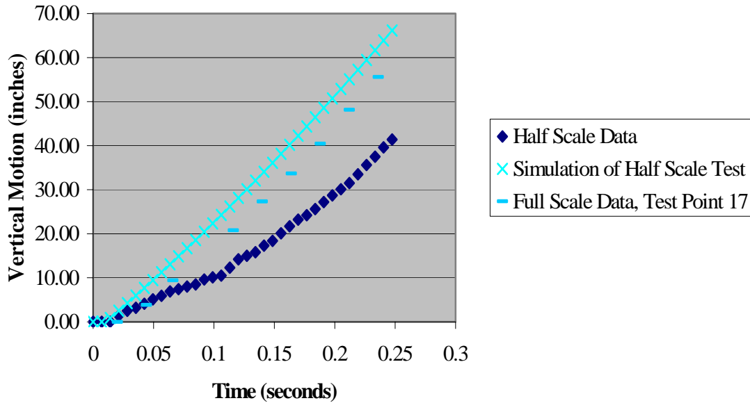
Figure G-1. Baseline Simulation Results, Vertical Motion, 70 Knots Full Scale-Conditions
