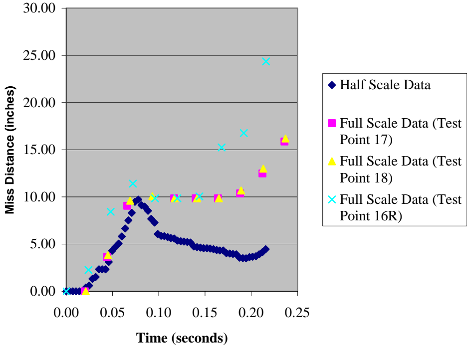
Figure E-1. Comparison of Miss-Distance Versus Time Calculation at 70 Knots Full-Scale Conditions
