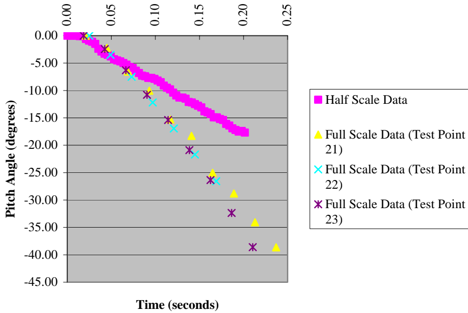
Figure D-2. Comparison of Pitch Motion at 100 Knots Full-Scale Conditions
