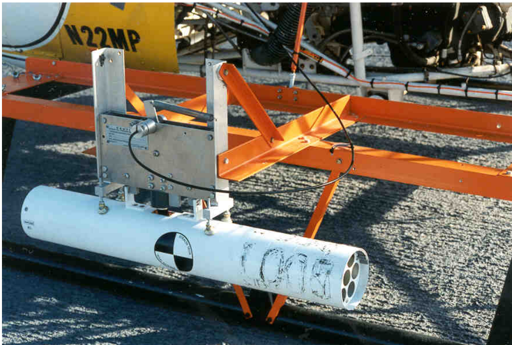
Figure 2. Scale Model and Ejector Rack Installation
