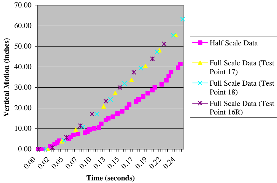
Figure C-1. Comparison of Vertical Motion at 70 Knots Full-Scale Conditions
