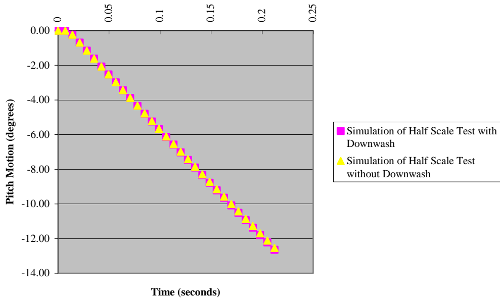
Figure F-2. Effect of Downwash on Pitch Motion, 40 Knots Full-Scale Conditions
