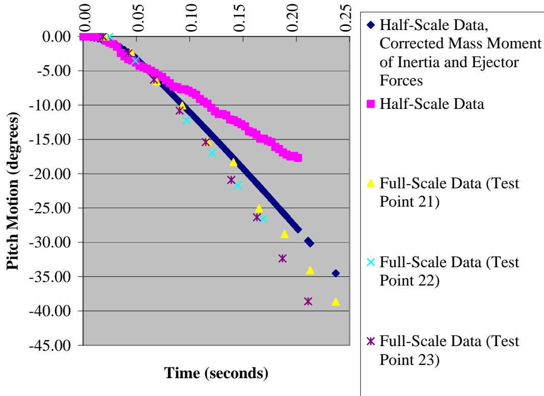
Figure 21. Effect of Ejector Forces and Mass Moment of Inertia on Half-Scale Pitch Motion Data, 100 Knots Full-Scale Conditions
