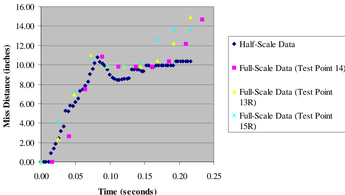
Figure 7. Calculated Miss-Distance Versus Time Curves at 40 Knots Full-Scale Conditions
