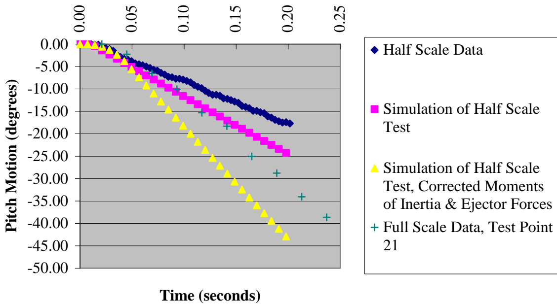
Figure H-3. Effect of Mass Moment of Inertia Plus Ejector Forces on Pitch Motion, 100 Knots Full-Scale Conditions
