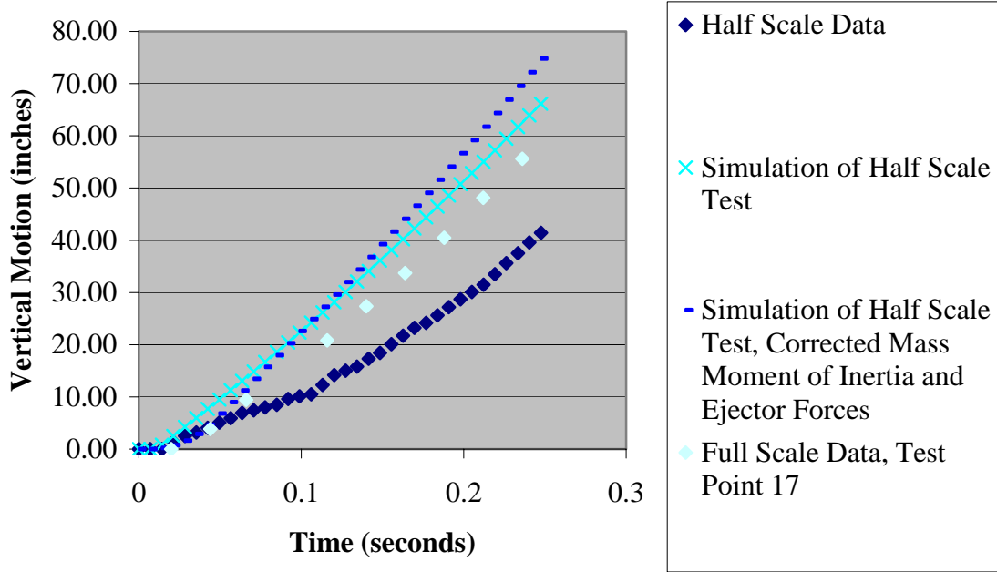
Figure H-2. Effect of Mass Moment of Inertia Plus Ejector Forces on Vertical Motion, 70 Knots Full-Scale Conditions
