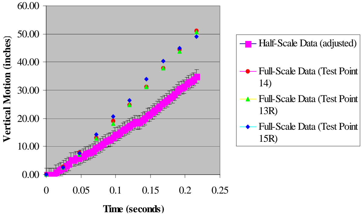
Figure 5. Comparison of Vertical Motion at 40 Knots Full-Scale Conditions
