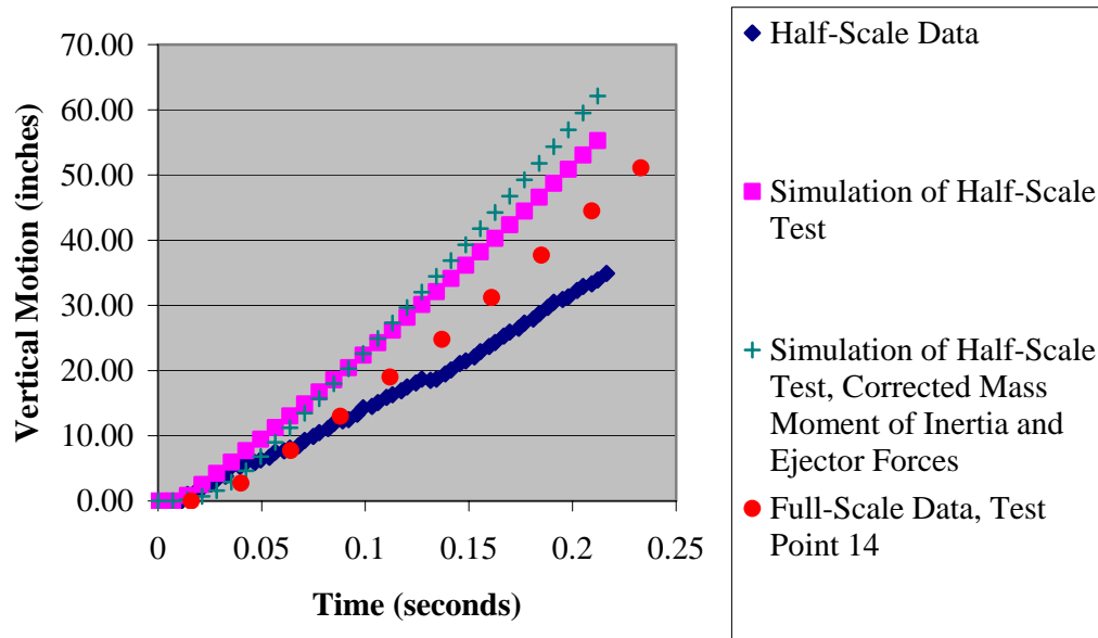
Figure 16. Effect of Mass Moment of Inertia and Ejector Forces on Vertical Motion, 40 Knots Full-Scale Conditions
