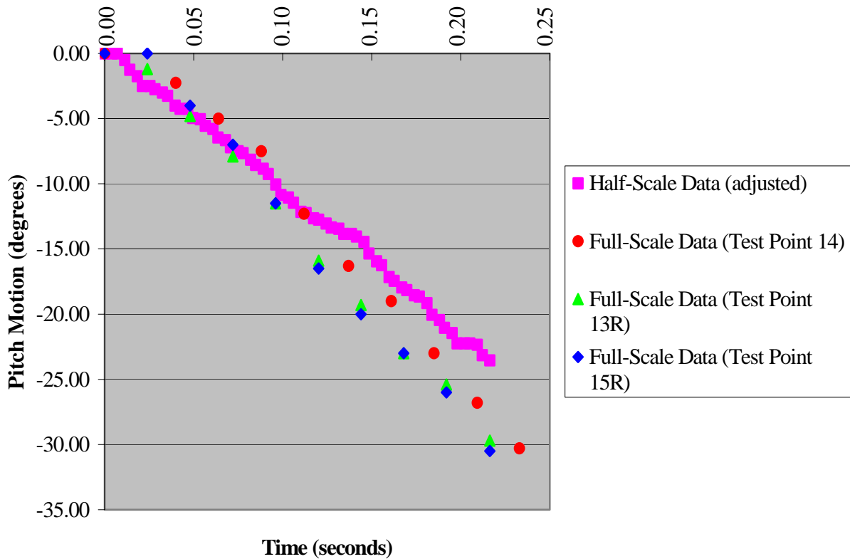
Figure 6. Comparison of Pitch Axis Motion at 40 Knots Full-Scale Conditions
