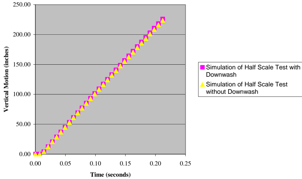
Figure F-1. Effect of Downwash on Vertical Motion, 40 Knots Full-Scale Conditions
