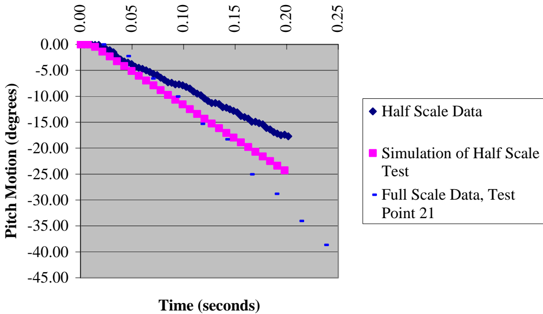
Figure G-4. Baseline Simulation Results, Pitch Motion, 100 Knots Full-Scale Conditions
