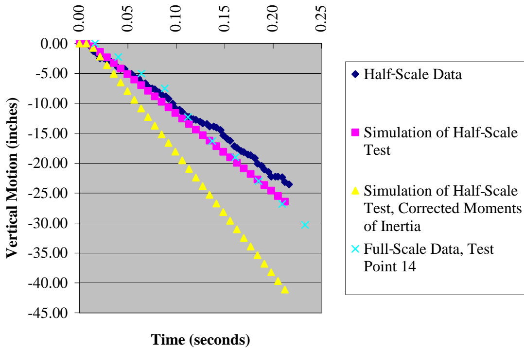
Figure 11. Effect of Mass Moment of Inertia on Pitch Motion, 40 Knots Full-Scale Conditions
