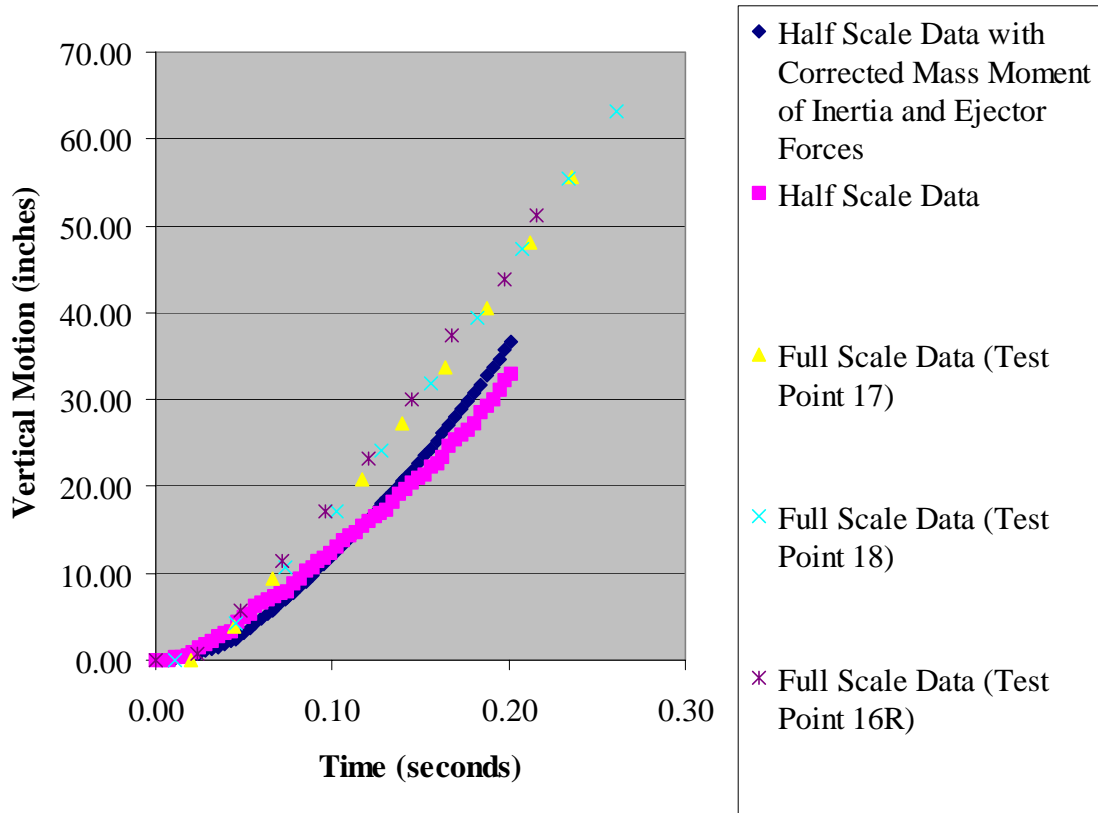
Figure I-1 Effect of Correct Mass Moment of Inertia Plus Ejector Forces on Half-Scale Vertical Motion, 70 Knots Full-Scale Conditions
