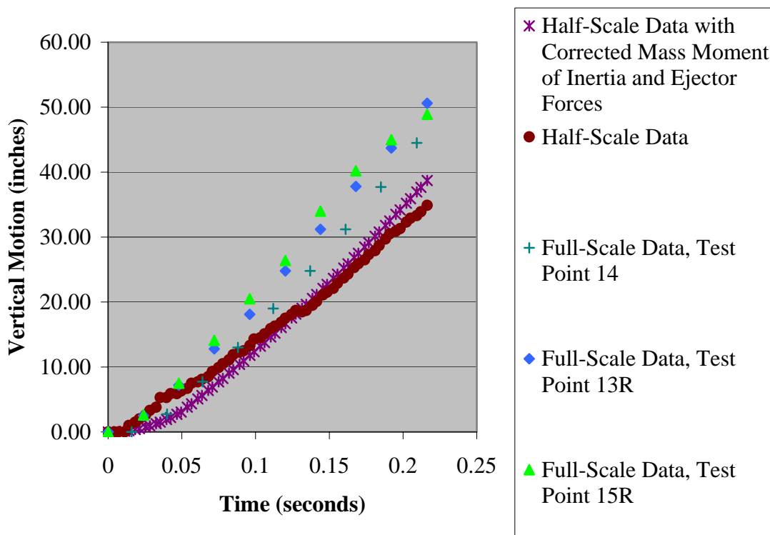
Figure 18. Effect of Ejector Forces and Mass Moment of Inertia on Half-Scale Vertical Motion Data, 40 Knots Full-Scale Conditions
