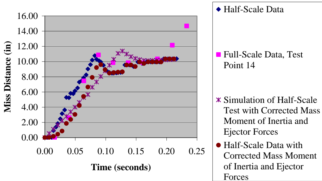
Figure 22. Effect of Mass Moment of Inertia and Ejector Forces on Miss-Distance at 40 Knots Full-Scale Conditions
