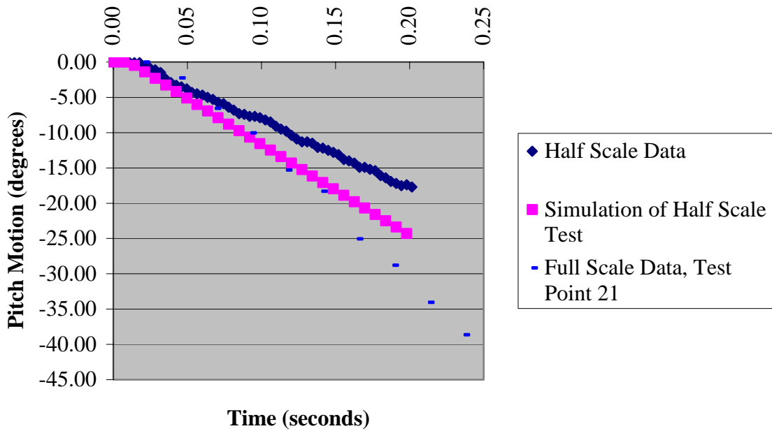
Figure G-3. Baseline Simulation Results, Pitch Motion, 70 Knots Full-Scale Conditions
