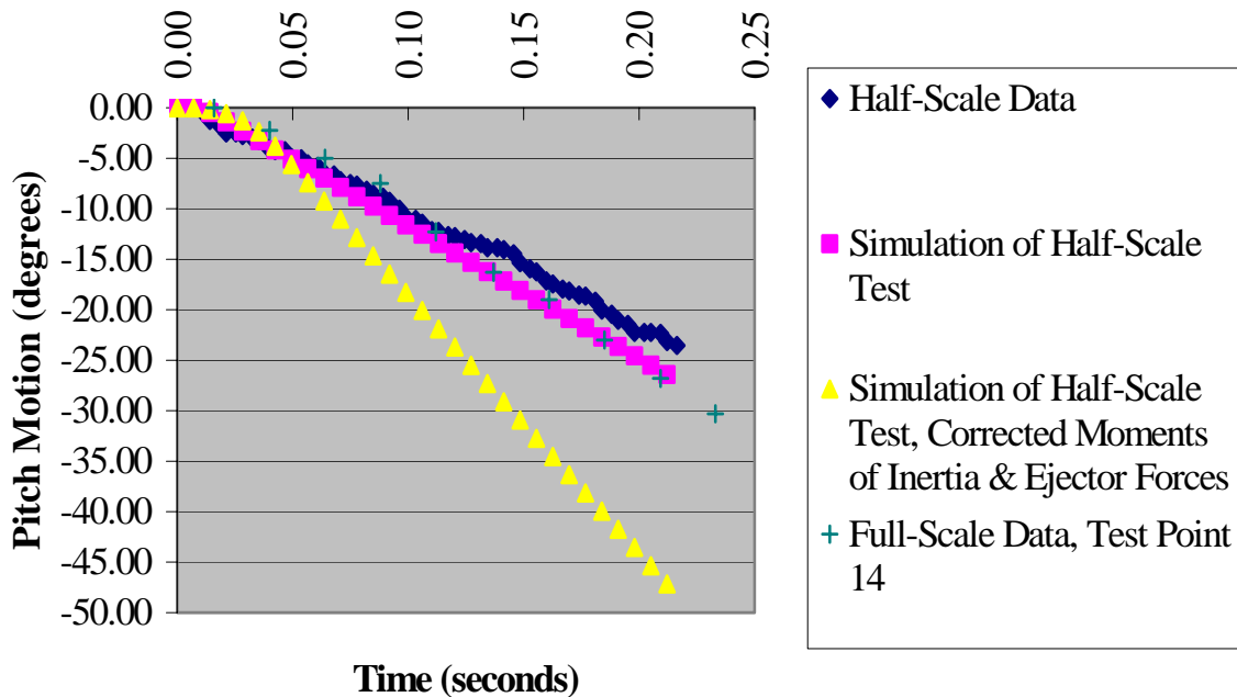
Figure 17. Effect of Mass Moment of Inertia and Ejector Forces on Pitch Motion, 40 Knots Full-Scale Conditions
