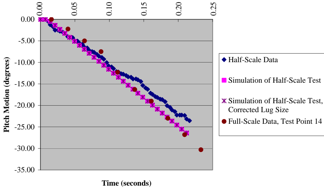
Figure 15. Effect of Lug Size on Pitch Motion, 40 Knots Full-Scale Conditions
