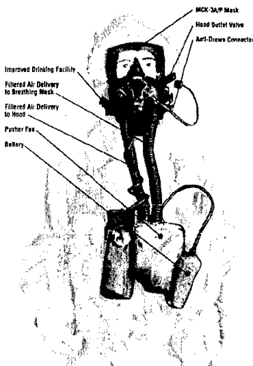
A/P22P-14(V)1 Non-Oxygen Assembly for Rotary Wing
