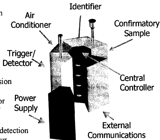
Potential JBPDS Block II Configuration
