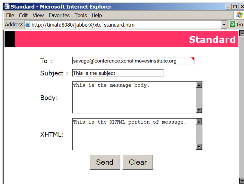
Figure 89. Sample HTML form for posting of data.
