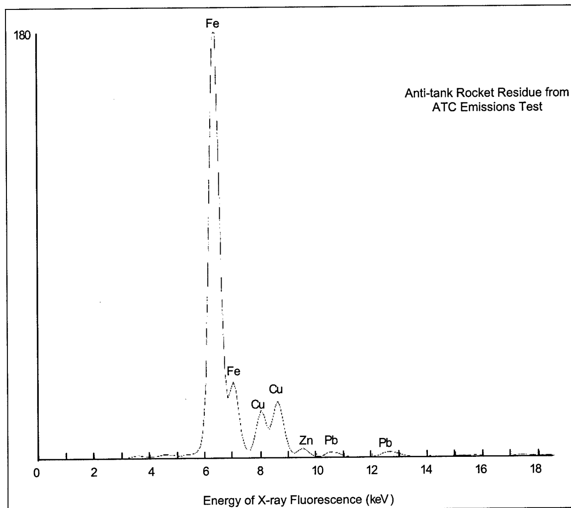
Figure 3. FP-XRF spectra of samples of post-blast ordnance residue from the Aberdeen Test Center Blast Chamber.
