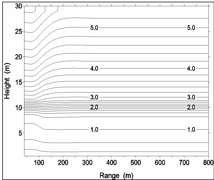
Figure 9. Horizontal wind velocity, \langle \bar{u} \rangle , in units \text{ms}^{-1} , within and above a uniform forest stand, where canopy height ( h ) is 10 m.
