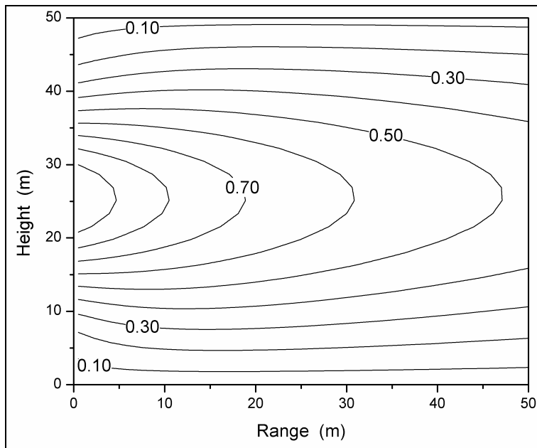
Figure 7. The 2-D steady-state scalar field derived from a scalar diffusion model solved via an implicit differencing scheme. In this example, the scalar diffusivity is K = 10 m^2 s^{-1} and the horizontal grid is \Delta x = 0.5 m .
