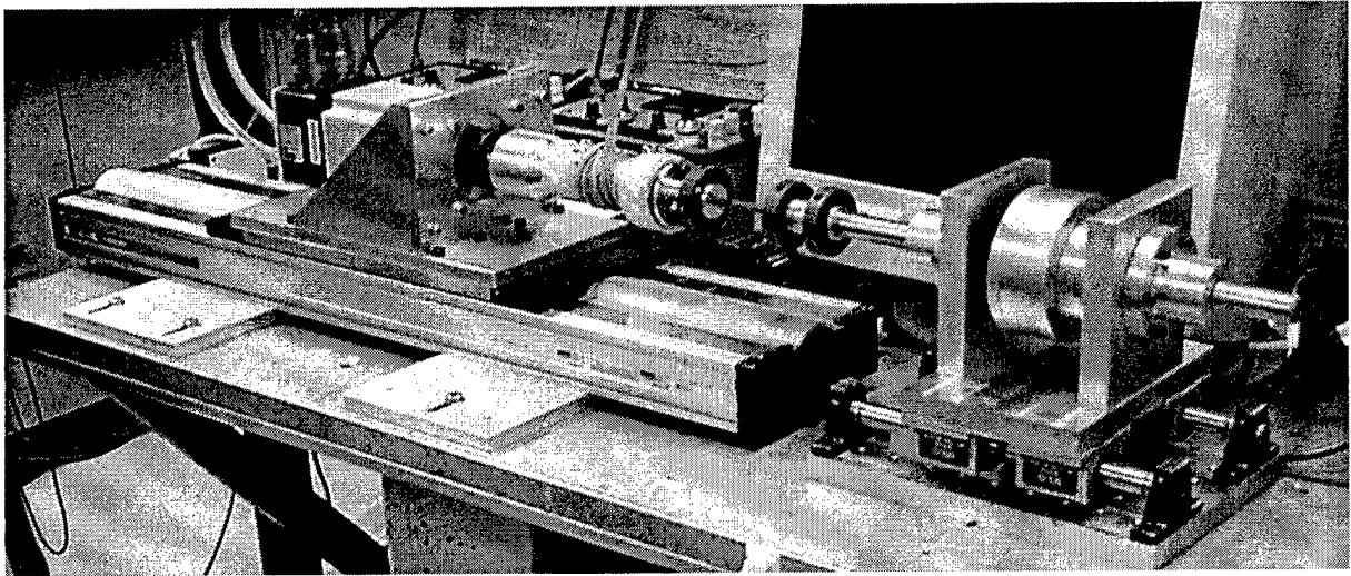
Figure 3: Photograph of multi-component hysteretic system with adjustable nonlinear characteristics
