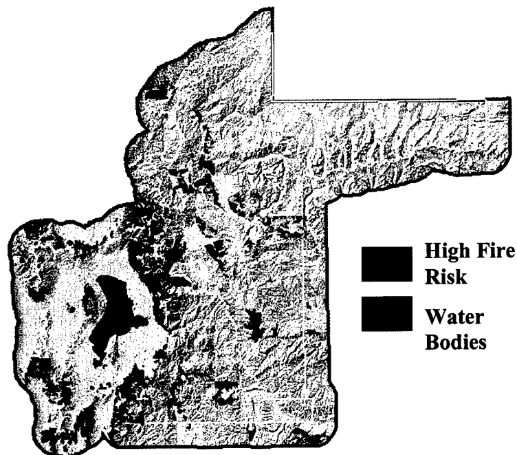
Figure 12. Areas in the study area with high wildfire risk (in red).
