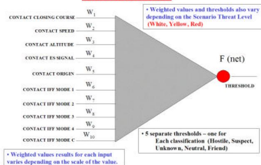
Figure 9. Contact Classification Artificial Neuron (From [24])
