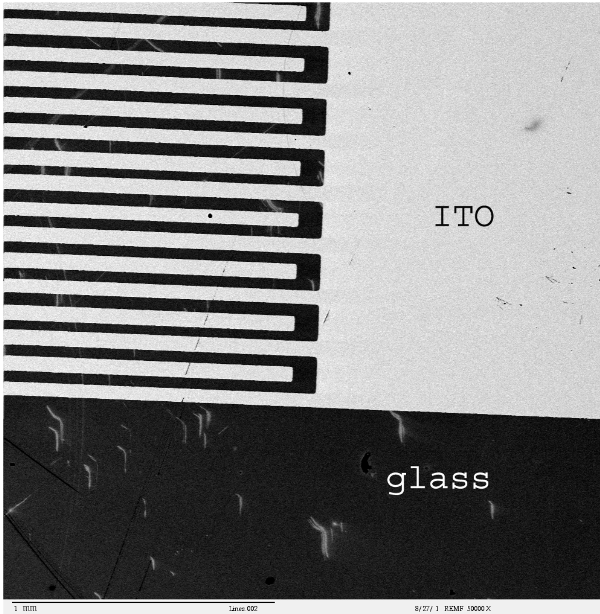
Figure 17. A wide electric bus and narrow electrodes are shown at the edge of the transparent device. ITO-coated glass (Compagnie de Saint-Gobain, France), SEM image (Zeiss DSM-962) (Back-Scattered Electron image).
