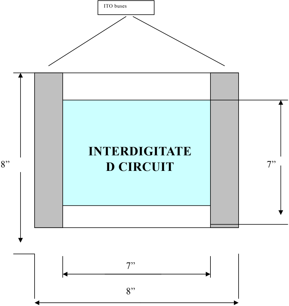
Figure 15. De-icer dimensions
