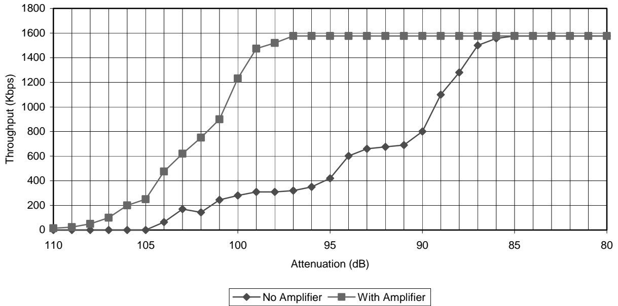
Figure 12. Significant Improvement in Distance With the Addition of a 2W Amplifier
