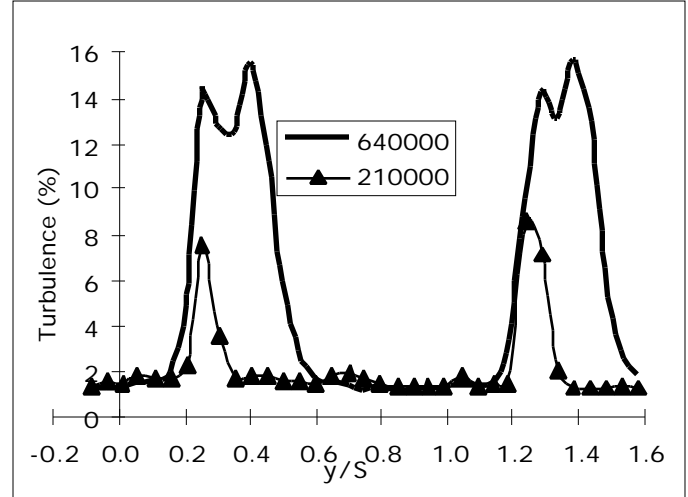
Fig. 11 Exit turbulence distributions for the highest and lowest Reynolds number flows.
