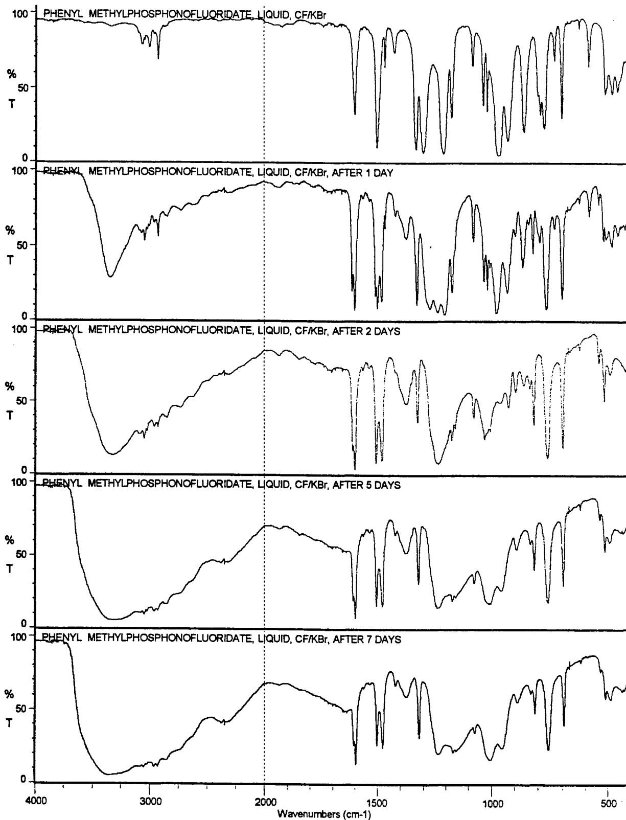
Figure 83 PHENYL METHYLPHOSPHONOFLUORIDATE, LIQUID, CF/KBr, AFTER EXPOSURE TO ATMOSPHERIC MOISTURE
