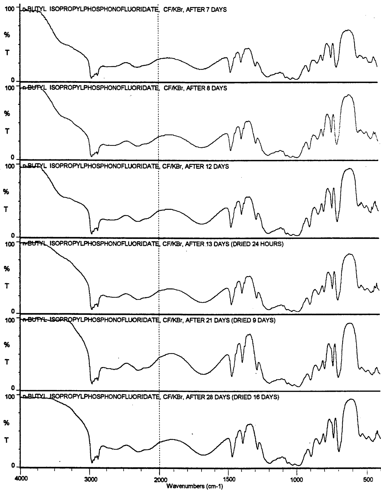
Figure 15. n -BUTYL ISOPROPYLPHOSPHONOFLUORIDATE, LIQUID, CF/KBr, AFTER EXPOSURE TO ATMOSPHERIC MOISTURE (CONTINUED)
