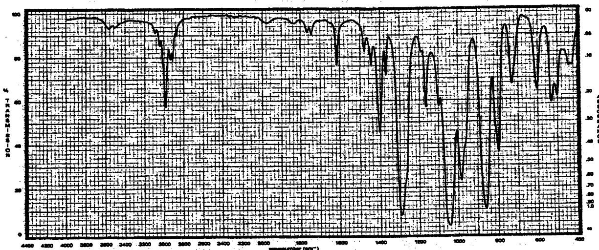
Figure 16 ETHYL VINYLPHOSPHONOFLUORIDATE, 99.5 MOLE %, LIQUID, CF/CsI
