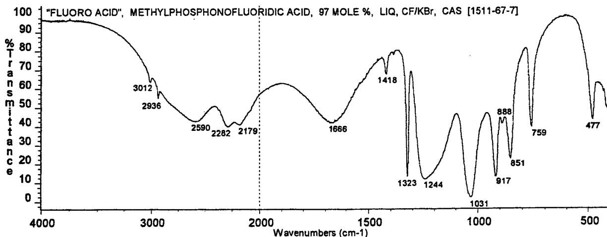
Figure 53 METHYLPHOSPHONOFUORIDIC ACID (FLURO ACID), LIQUID, CF/KBr
