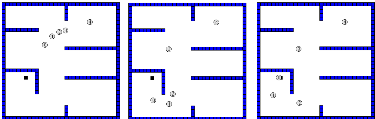
Figure 4. A simulation of the convoying strategy, developed by the University of Massachusetts, Amherst. Robot 0 is the leader, who is trying to reach the goal (black square). Robot 4 is the base station. The others act as relay nodes.
