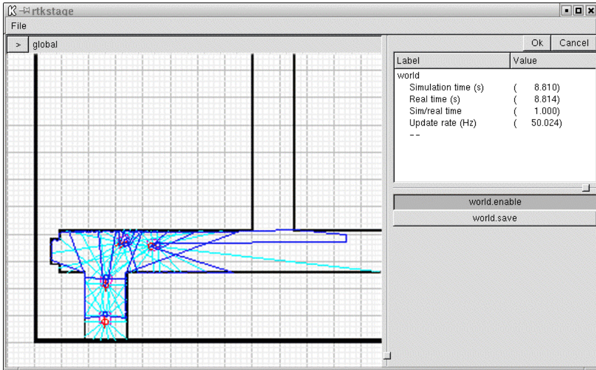
Figure 3. A simulation of the convoying behavior using laser-retroreflective beacons mounted on the back of each robot. The lead robot is moving randomly. The dark lines outline the areas visible to each ladar. The light lines represent sonar pings.
