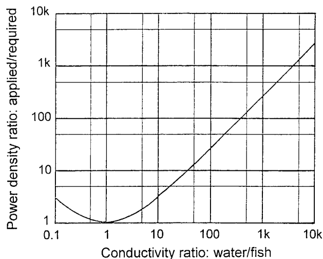
Fig. 12. Power-density-transfer curve. (Represents the relation D_w/D_f = (1 + q)^2/(4q) , where q = c_w/c_f (the conductivity mismatch ratio, water to fish) for predicting the increase in applied power density in water ( D_w ) necessary to maintain a constant transfer of required power density (e.g., that for a desired response) to the fish ( D_f ) as the conductivity ratio ( \delta ) increases or decreases from unity with changes in water conductivity. This relation was derived from concepts of normalized power and load mismatch by Kolz, 1989a and is fundamental to his theory of power transfer for electrofishing. Reproduced with permission from Fig. 1 in Kolz and Reynolds, 1989b; axis labels modified.)
