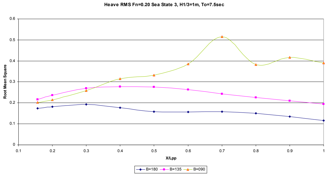
Figure 40. Fn=0.2 Heave RMS Values at Sea State 3 for Different Headings
