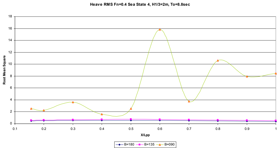
Figure 47. Fn=0.4 Heave RMS Values at Sea State 4 for Different Headings
