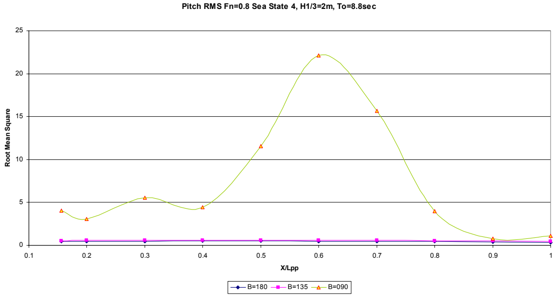
Figure 62. F_n=0.8 Pitch RMS Values at Sea State 4 for Different Headings
