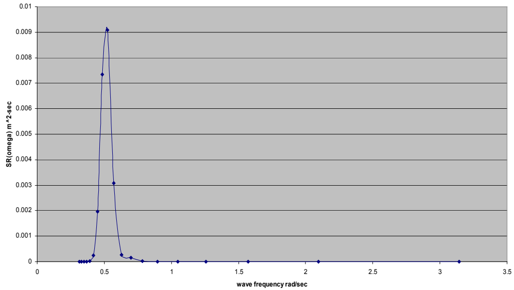
Figure 8. Ship response spectrum for generic trimaran at Sea State 4
