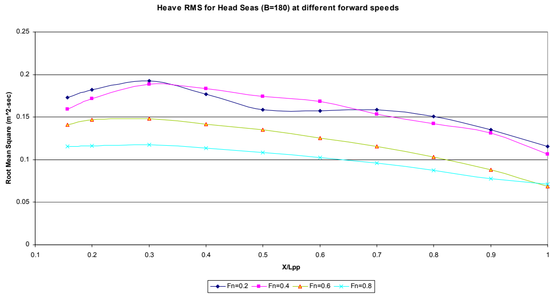
Figure 66. Heave RMS Values at Different Forward Speeds for Head Seas
