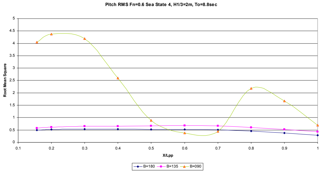
Figure 56. F_n=0.6 Pitch RMS Values at Sea State 4 for Different Headings
