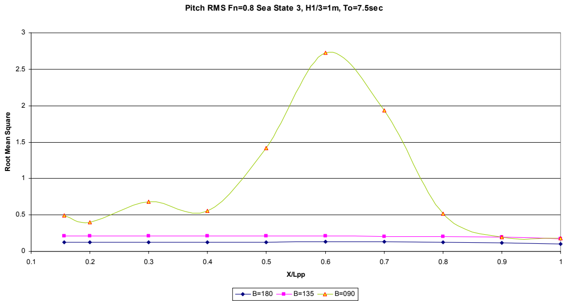
Figure 61. Fn=0.8 Pitch RMS Values at Sea State 3 for Different Headings
