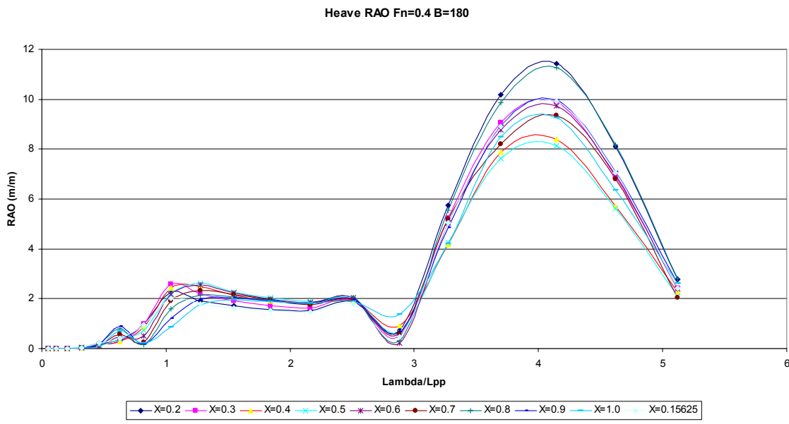
Figure 20. F_n=0.4 Heave Response Amplitude Operators for Head Seas
