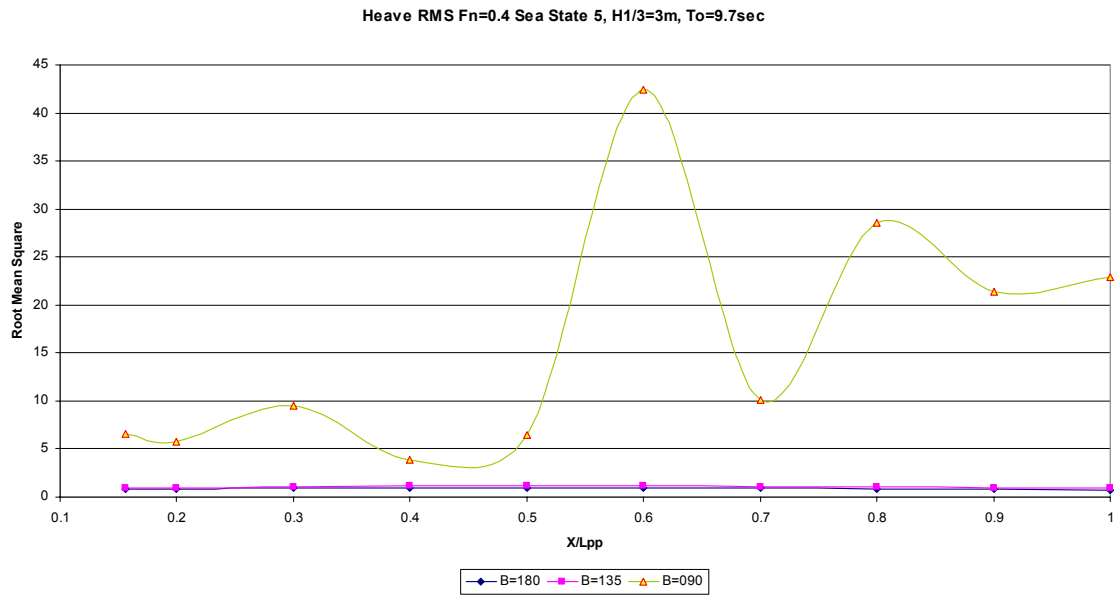
Figure 48. Fn=0.4 Heave RMS Values at Sea State 5 for Different Headings
