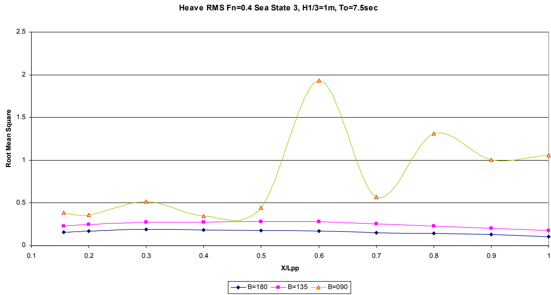
Figure 46. Fn=0.4 Heave RMS Values at Sea State 3 for Different Headings
