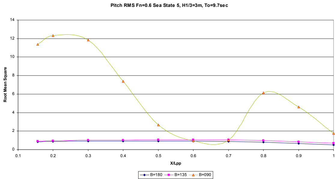
Figure 57. F_n=0.6 Pitch RMS Values at Sea State 5 for Different Headings
