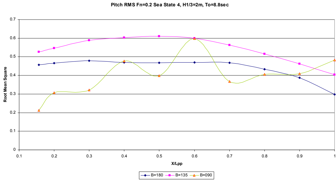
Figure 44. Fn=0.2 Pitch RMS Values at Sea State 4 for Different Headings
