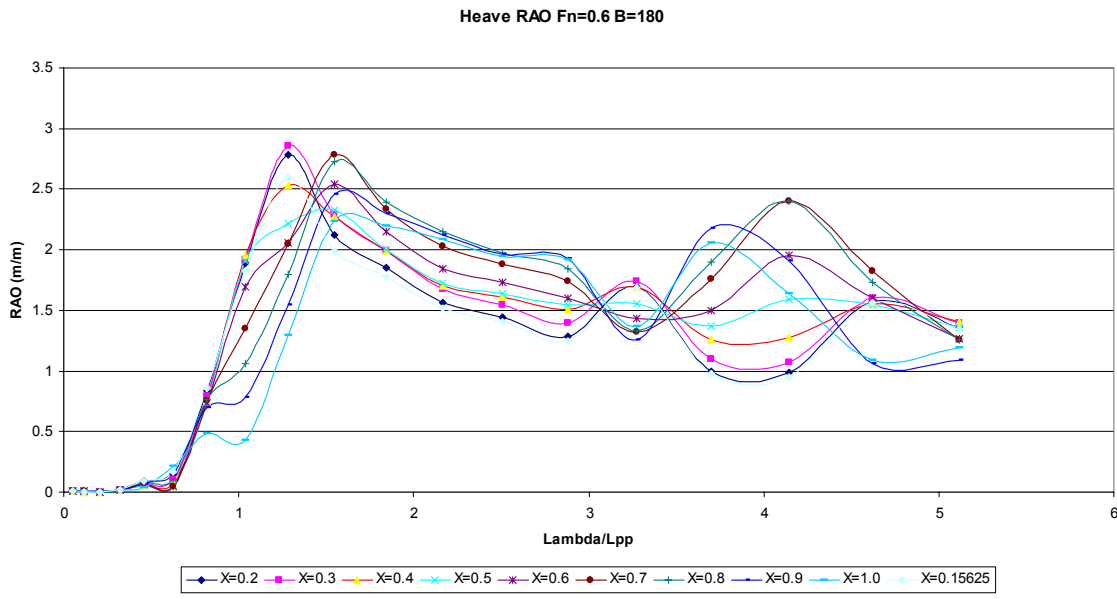
Figure 26. Fn=0.6 Heave Response Amplitude Operators for Head Seas
