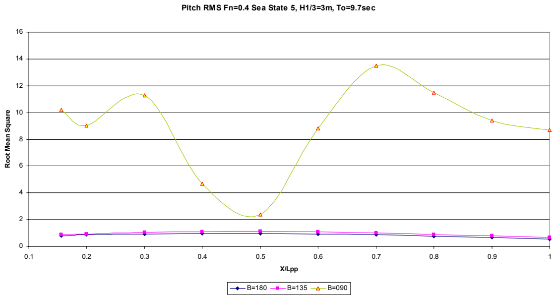
Figure 51. Fn=0.4 Pitch RMS Values at Sea State 5 for Different Headings
