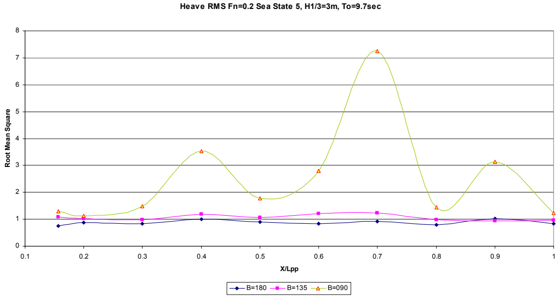
Figure 42. F_n=0.2 Heave RMS Values at Sea State 5 for Different Headings
