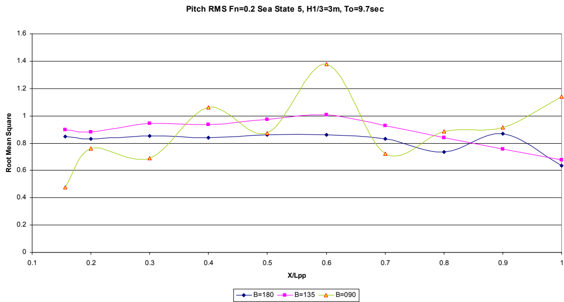
Figure 45. Fn=0.2 Pitch RMS Values at Sea State 5 for Different Headings
