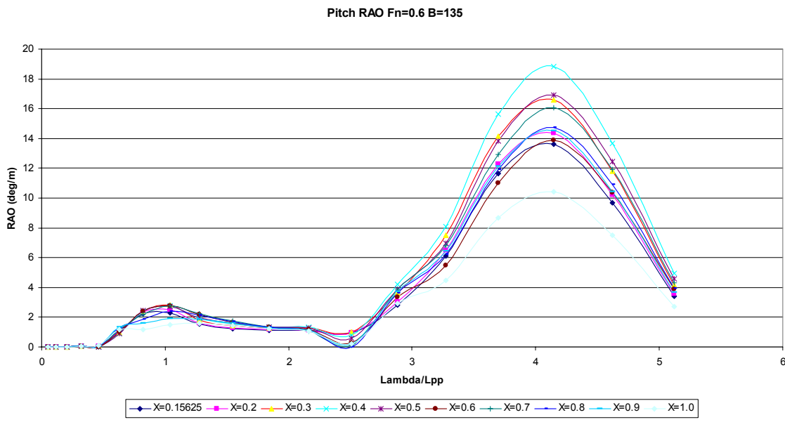
Figure 30. Fn=0.6 Pitch Response Amplitude Operators for Bow Quartering Waves
