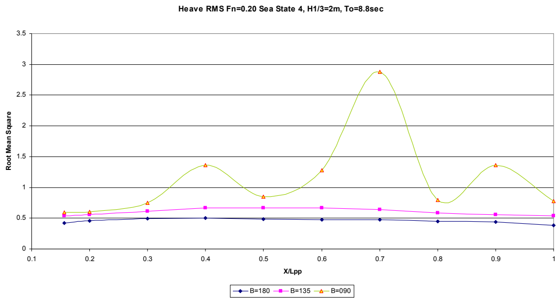
Figure 41. Fn=0.2 Heave RMS Values at Sea State 4 for Different Headings
