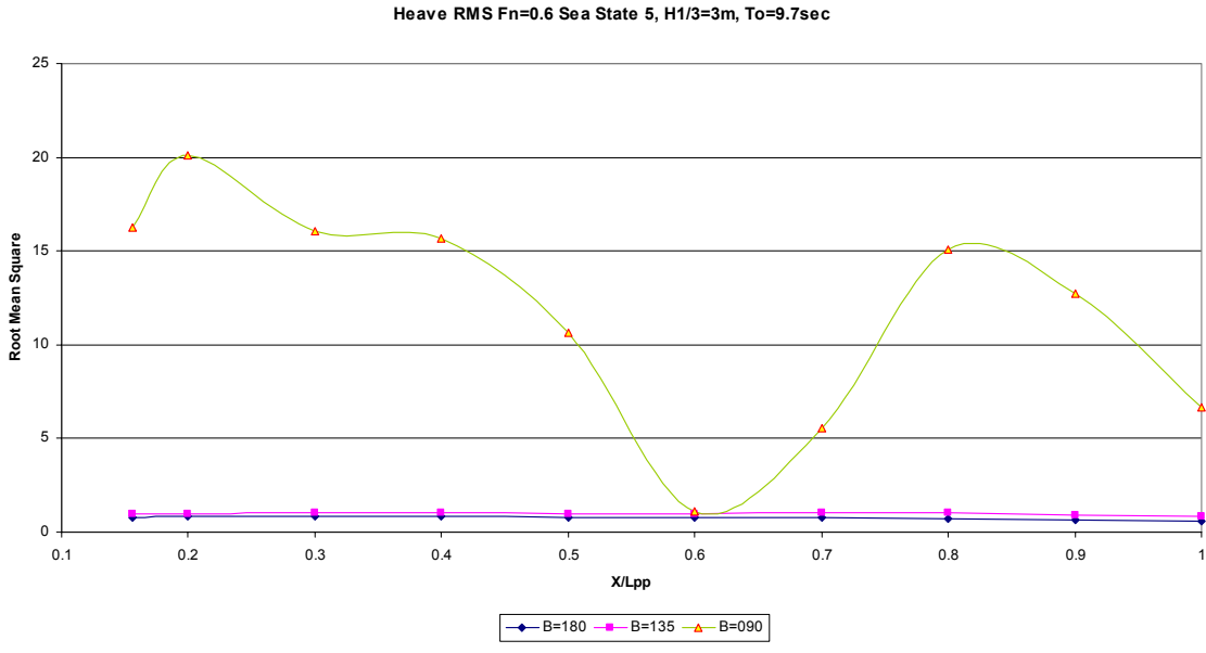
Figure 54. F_n=0.6 Heave RMS Values at Sea State 5 for Different Headings
