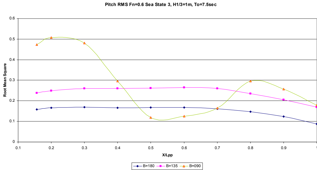
Figure 55. F_n=0.6 Pitch RMS Values at Sea State 3 for Different Headings
