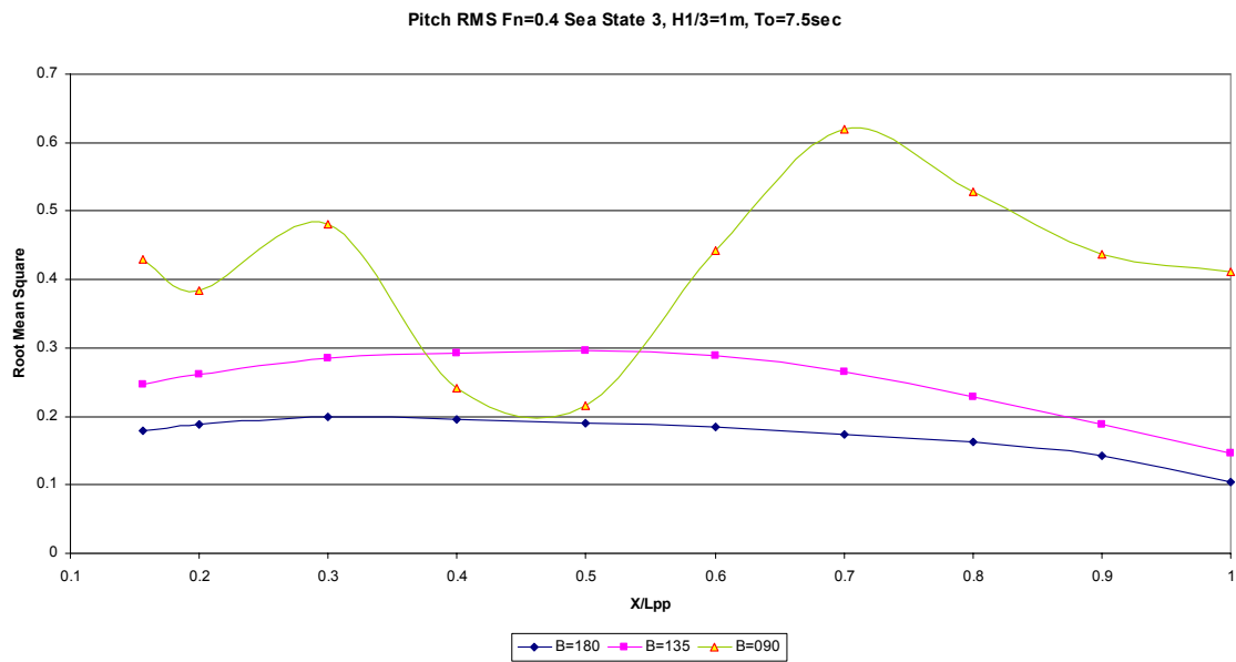
Figure 49. Fn=0.4 Pitch RMS Values at Sea State 3 for Different Headings
