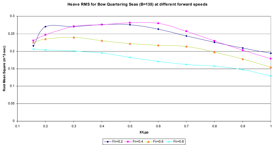
Figure 67. Heave RMS Values at Different Forward Speeds for Bow Quartering Waves
